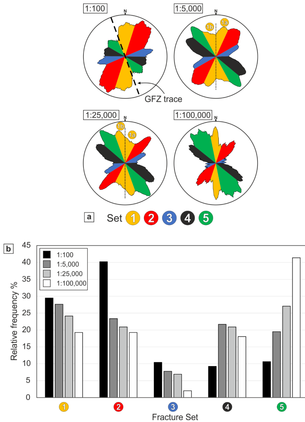
Figure 5. Rose diagrams (a) and histograms of the relative frequencies (b) of the identified orientation sets at different scales of observation.
