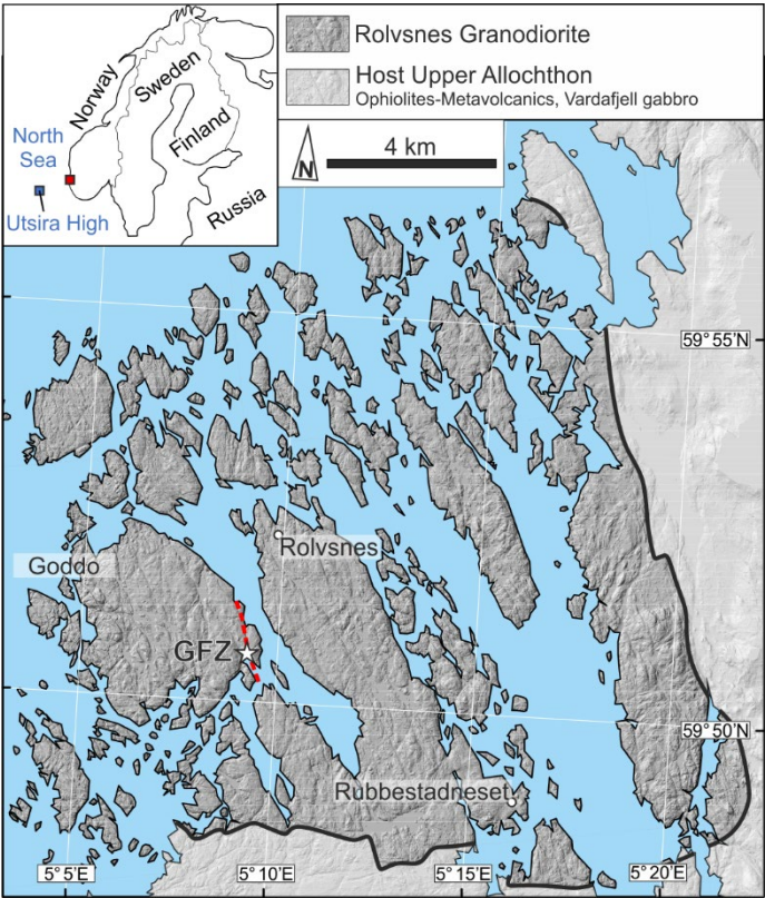
870 Figure 1. Simplified geological map of part of the Bømlo Island centered on the Rolvsnes granodiorite overlaying the Digital Terrain Model obtained from high-resolution (1 m/pxl) LiDAR survey (countresy of Norges Geologiske Undersøkelse). The inset shows the location of the study area (red square) and the location of the Utsira High within the North Sea (blue square). The trace of the exposed Goddo Fault Zone (GFZ) is indicated by the red dashed line.
