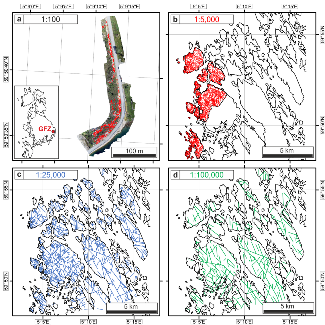
890 Figure 3. Lineament Maps produced by manual lineament picking on outcrop orthophotos (a) and DTM from LiDAR surveys (b-c-d).
