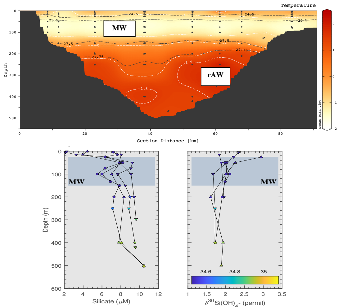
Figure 9: Top: Integrated hydrography of the Ile-de-France section for 2017-2019. Isotherms are shown in white and isopycnals in black. MW = meteoric water, rAW = recirculated Atlantic Water. Bottom panels: DSi concentrations (left) and \delta^{30}\text{Si}(\text{OH})_4 (right) for late summer 2017 (circle), 2018 (upwards triangle) & 2019 (downwards triangle) of the Ile-de-France section. Colourscale represents salinity (psu).
