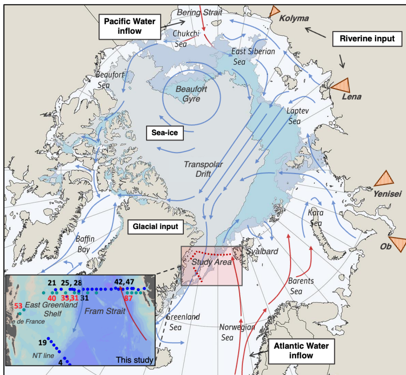
970 Figure 1: Map of the Arctic ocean showing the study area of this research and general surface circulation patterns within the Arctic ocean. Red arrows represent warm, saline currents of the Atlantic and Pacific, and blue arrows represent fresh, cold water modified within the Arctic ocean (adapted from Tremblay et al., 2005). Orange triangles show the river deltas of four rivers which constitute the largest freshwater source to the Atlantic-Arctic sector: the Ob, Yenisei, Lena & Kolyma rivers. Shaded areas of the central Arctic shows September sea ice extent for 2006 (dark blue), 2017 (light blue) and 2020 (grey-blue). Figure adapted from NSIDC, 975 2020. Inset: Nitrate isotope sample stations for this study are shown with blue dots (JR17005) and green dots (FS2018). The station numbers for silicon isotope profiles measured within this study are shown in red for FS2018 & black for JR17005.
