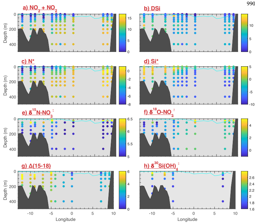
010 Figure 3: Nutrients and isotopes across Fram Strait section of late summer 2018 a) NO x (where NO x = nitrate + nitrite), b) DSi, c) N* (where N* = NO x - 16*PO 4 ), d) Si* (where Si* = Si(OH) 4 - NO x ), e) δ 15 N-NO 3 , f) δ 18 O-NO 3 , g) Δ(15-18) (where Δ(15-18) = δ 15 N-NO 3 - δ 18 O-NO 3 ), h) δ 30 Si(OH) 4 . Cyan line displays MLD for the section (calculation described in method section).
