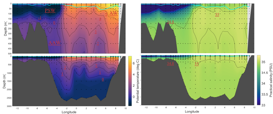
Figure 2: Hydrography of Fram Strait cruise FS2018 from August-September 2018 presented for full depth (bottom panel) and upper water column (top panel) for temperature (left) and salinity (right) . The mixed-layer depth is shown by a cyan line (calculation of MLD is described in method section below). Isotherms (left) & isohalines (right) are also displayed. Atlantic Water (AW), Polar Surface Water (PSW) & Arctic Atlantic Water (AAW) are marked.
