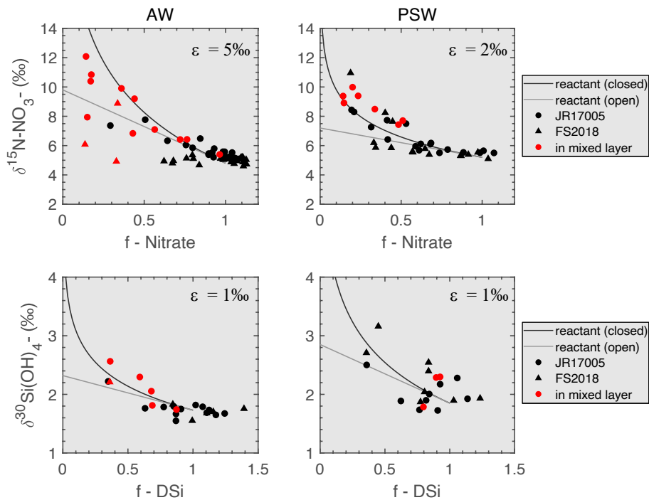
Figure 6: Top panels: nitrate utilisation vs \delta^{15}\text{N-NO}_3 for AW (left, depth < 600m) and PSW (right, depth < 150m). Bottom panels: DSi utilisation vs \delta^{30}\text{Si(OH)}_4 for AW (left, depth < 600m) and PSW (right, depth < 150m). Circles are measurements from JR17005 (spring) and triangles from FS2018 (summer). Red symbols show measurements within the mixed layer. Black line follows the closed fractionation model and grey line an open fractionation model. f is the fraction of nutrient remaining, calculated from the nutrient concentrations of water masses AW and PSW below the MLD (Table 2).
