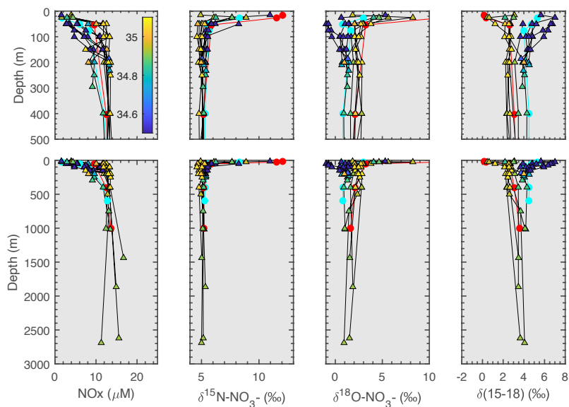
055 Figure 5: Nitrate concentrations (left), \delta^{15}\text{N-NO}_3^- (middle-left), \delta^{18}\text{O-NO}_3^- (middle-right) and \Delta(15-18) profiles (right) for FS2018 (triangles) in Fram Strait. Typical profiles for PSW (cyan) and AW (red) from JR17005 are shown in circles for comparison between studies (Tuerena et al., 2021). Colourscale represents salinity (psu).
