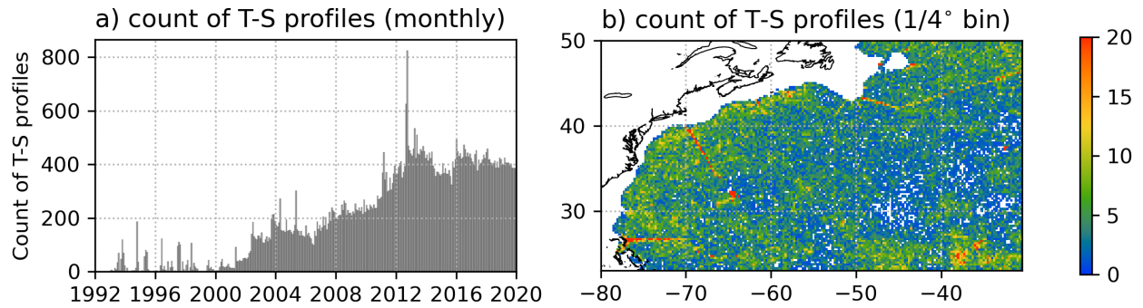
Figure 1. Count of temperature and salinity profiles extending from 25 to 1000 m for the region. The profiles are counted for 1/4^\circ bins (ab) and represented where it exceeds 0 with a truncated colorbar at 20 profiles, the maximum number of profiles for a bin is 185 profiles. The count in (ba) is by months.
