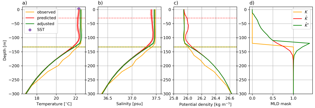
Figure 4. Example of a profile (orange) sampled the on 2012-03-03 at 35.55°W and 23.53°N, truncated at 300 m deep. We display temperature (a), salinity (b), potential density (c) and the profile K that is a mask of MLD (see equation (1)). The T-S profile predicted by the NN is in red and the adjusted using the \hat{K}^* profile (OSnet) in green (see section 3.3). The green and red bands are the confidence interval for each profiles, i.e. the standard deviation of the 15 bootstrapped models . Mixed Layer Depths (MLDs) for observed, predicted and adjusted are shown with dotted horizontal lines. SST is added with a purple dot and a horizontal bar for its mapping uncertainty.
