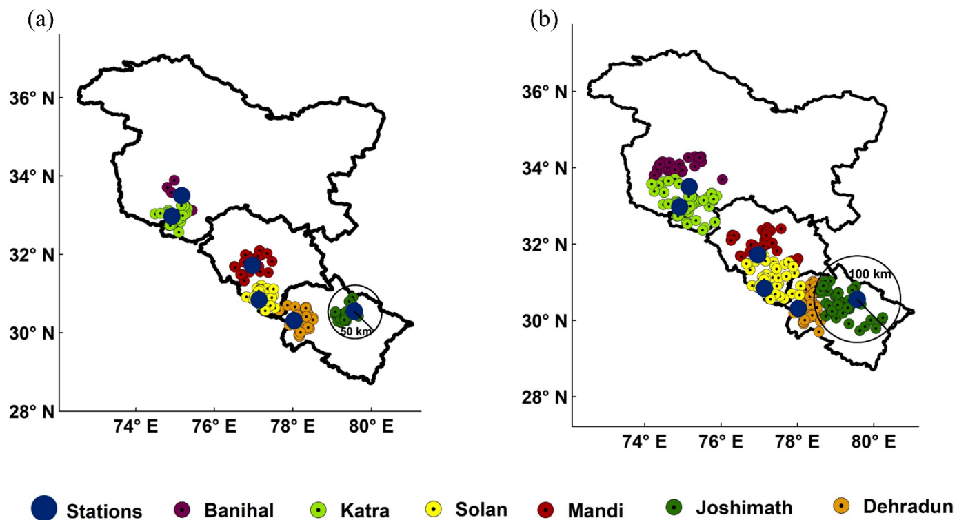
Fig. S1. Landslide events within (a) 50 km and (b) 100 km radius of selected sites.
