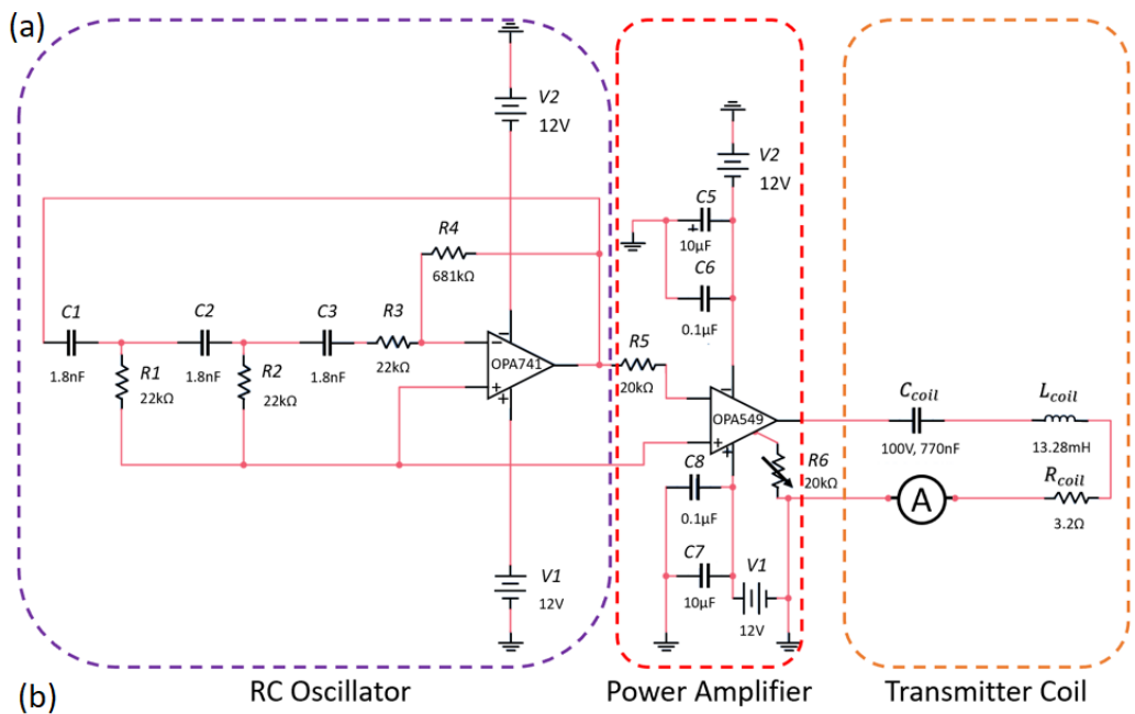
Figure 4. (a) Low-cost CSM-EM Tx system powered by two 12 V motorcycle batteries. The RC oscillator generates an AC signal at a given frequency, which is amplified by the power amplifier before being passed into the Tx coil to generate an AC signal and corresponding magnetic field. The DMM measures the alternating current passing through the Tx coil. (b) CSM-EM Tx circuit diagram that can be split into three primary modules: the RC oscillator, the power/signal amplifier, and the Tx coil (with tuning capacitor). The circuit is composed of basic electronic components along with an OPA549 power amplifier breakout board. Resistor R_5 was included to allow regenerative feedback in the circuit and is not part of a specific Tx module.
