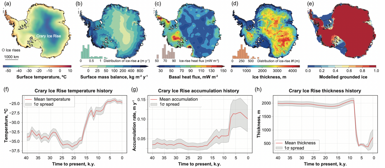
Fig. 1. Present-day distribution of key parameters affecting temperature-depth profiles in Antarctica: (a) ERA-Interim annual mean surface temperatures (Albrecht et al., 2020a). White areas in (a)-(e) indicate locations of ice rises from an Antarctic-wide inventory presented in Matsouka et al. (2015). (b) Mean surface mass balance (that is, the difference between accumulation and ablation at the ice-sheet surface) for the period 1979-2015 (Agosta et al., 2019) and distribution of approximate accumulation rates extracted for all ice-rise locations. (c) Basal geothermal heat flux reconstructed from magnetic data (Martos et al., 2017) and distribution of heat flux below ice rises. (d) Ice thickness and ice-rise thickness distribution (Fretwell et al., 2013). (e) Ensemble-score weighted grounded mask for the present-day ice-sheet reflecting possible histories of grounding line migration since deglaciation (Albrecht et al., 2020b). Red color indicates grounded areas which are covered by grounded ice in all simulations. Blue color indicates areas which are covered by few simulations with low scores;. The grounding line and coastlines are shown in black. White dot shows the location of Crary Ice Rise, where previously timing of grounding was inferred using borehole temperature measurements (Bindshadler, 1990). (f)-(h) 40 k.y. - histories of surface temperature, accumulation and thickness in the vicinity (i.e., within about 200 km) of Crary Ice Rise obtained from large-scale Parallel Ice Sheet Model (PISM) simulations (Kingslake et al., 2018; Albrecht et al., 2020a; 2020b).
