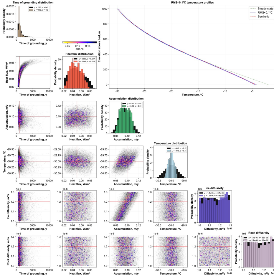
Fig. 1. Inversion of the synthetic temperature profile data based on 256000 parameter combinations, including the thermal diffusivity of ice and bedrock. Synthetic temperature-depth profile (red dotted line in upper right panel) was produced using the prescribed set of parameter values, including thermal diffusivity of ice and rock (two lower rows). The scatter plots illustrate the random walk in parameter space: in grey are the tested combinations of parameter values that yielded a less than 0.3°C RMS misfit with synthetic temperature profile, while in color are the combination of parameter values that yield best-fit with synthetic profile (i.e., <0.1°C RMS). Panels in the lower two rows shows that closely matching temperature profiles are reproduced using a wide range of thermal diffusivity values, but their effect on inferred grounding time is negligible.
