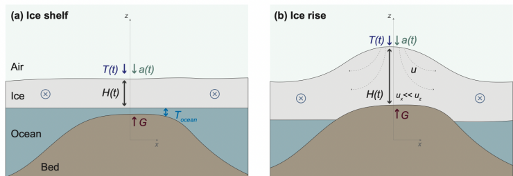
Fig. 2. Geometry of the ice shelf - ice rise heat flow model. The simple 1D vertical model is implemented along a stationary crest of hypothetical ice rise ( z axis on the figure) and bedrock beneath it. T(t) and a(t) indicate surface temperature and accumulation forcings, respectively. G is geothermal heat flux, u is ice flow velocity (along the crest of ice rise, horizontal flow velocity u_x is negligibly small comparable to its vertical component u_z , or w ).
