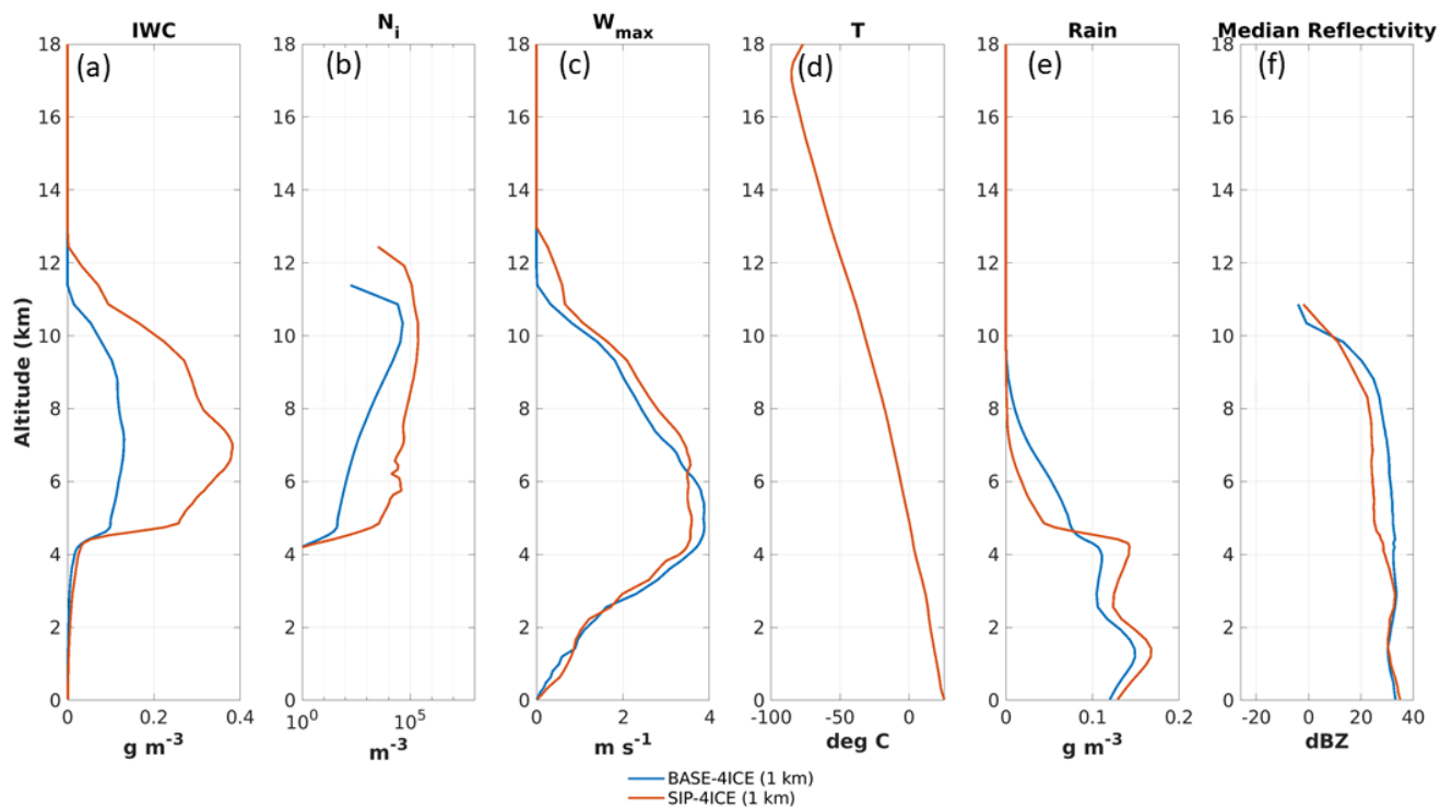
890 Figure 22: Similar to Figure 6 but for simulation at 1 km horizontal grid spacing.
