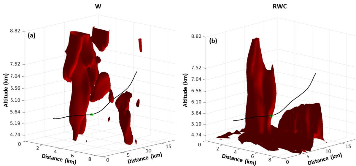
880 Figure 19: the trajectory of a specific air parcel (black line) and the location of the parcel at t = 0 min (green circle). The red surfaces in (a) show the area with w larger than 3 m/s, and in (b) with RWC larger than 0.05 \text{ g m}^{-3} , at the moment of t = 0 min.
