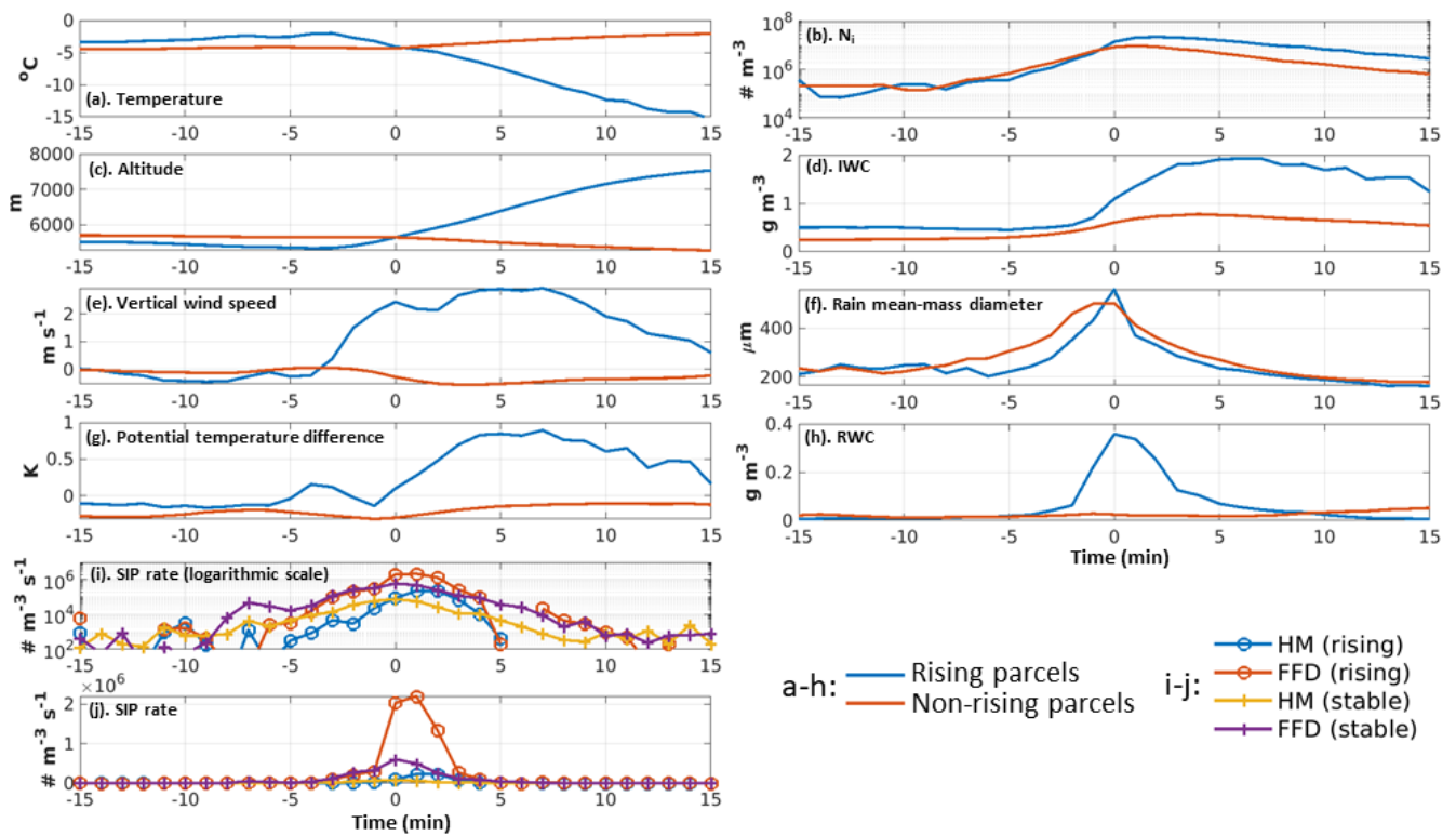
875 Figure 18: trajectory tracing of different variables for the rising parcels (blue lines in a-h) and the non-rising parcels (red lines in a-h). a: temperature, b: N_i , c: Altitude, d: IWC, e: vertical wind speed, f: rain mean-mass diameter, g: \Delta\theta , h: RWC, i: SIP tendency in logarithmic scale, j: SIP tendency in regular scale.
