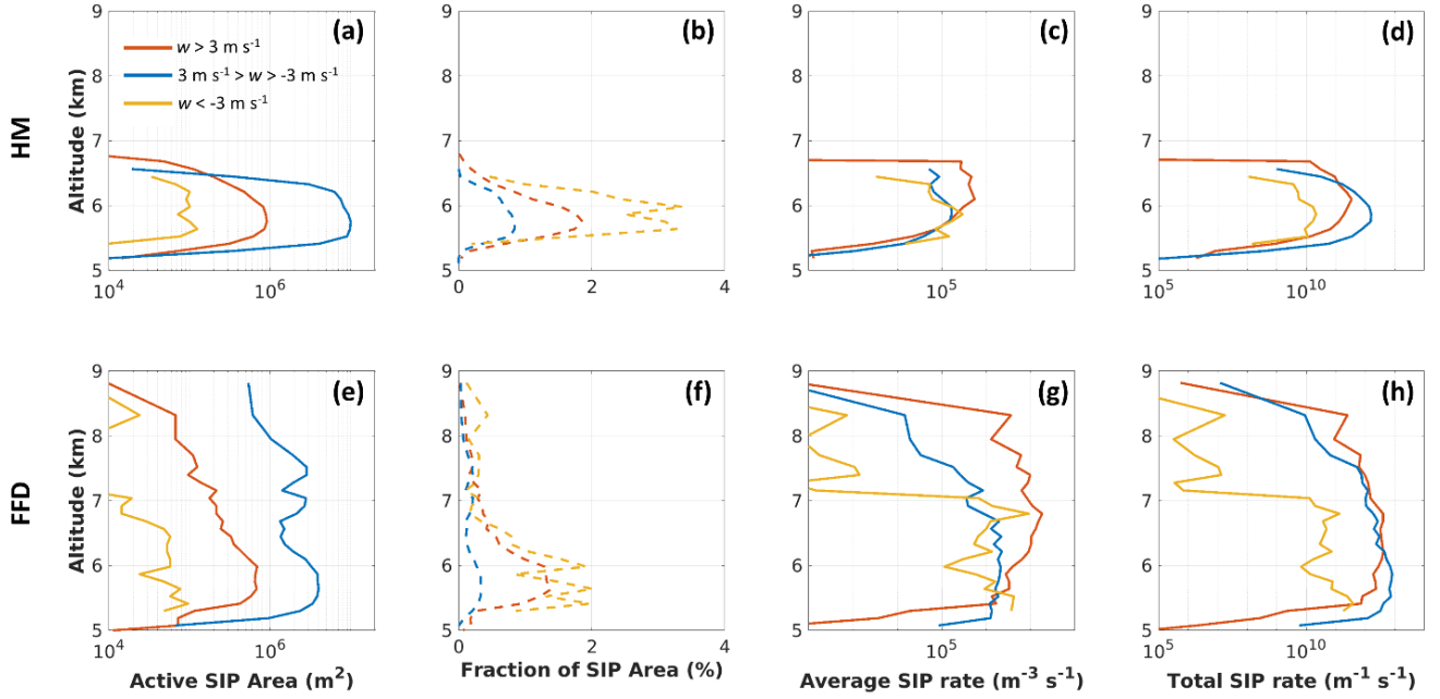
870 Figure 17. (a): area in \text{m}^2 with active HM process; (b): fraction of area with active HM process; (c): average rate of SIP by the HM process within the active area shown in (a); (d): total SIP rate, product of (a) and (c). (e) to (h): same as (a) to (d) but for the FFD process. Red lines (updrafts): SIP with w > 3 \text{ m s}^{-1} , blue lines (outside of updrafts/downdrafts): SIP with w between -3 and 3 \text{ m s}^{-1} , yellow lines (downdrafts): SIP with w < -3 \text{ m s}^{-1} . All results are temporal averages between 90 and 120 min.
