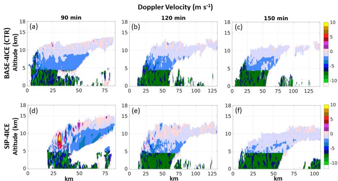
Figure 15. Simulated Doppler speed for the cross-sections indicated by the black lines in Figure 10.
