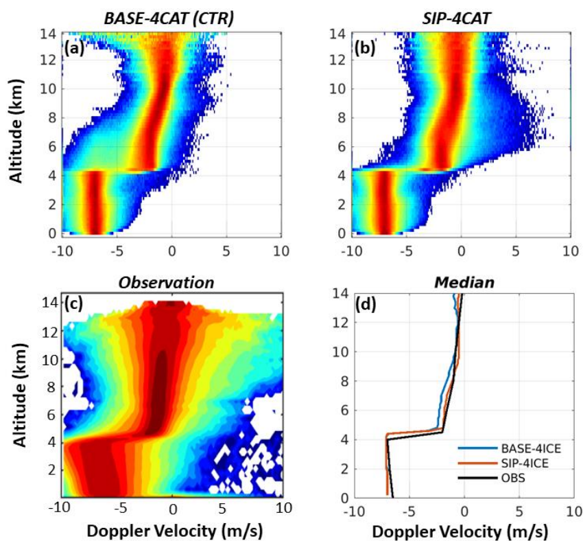
865 Figure 16. Same for Figure 12 but for the Doppler velocity.
