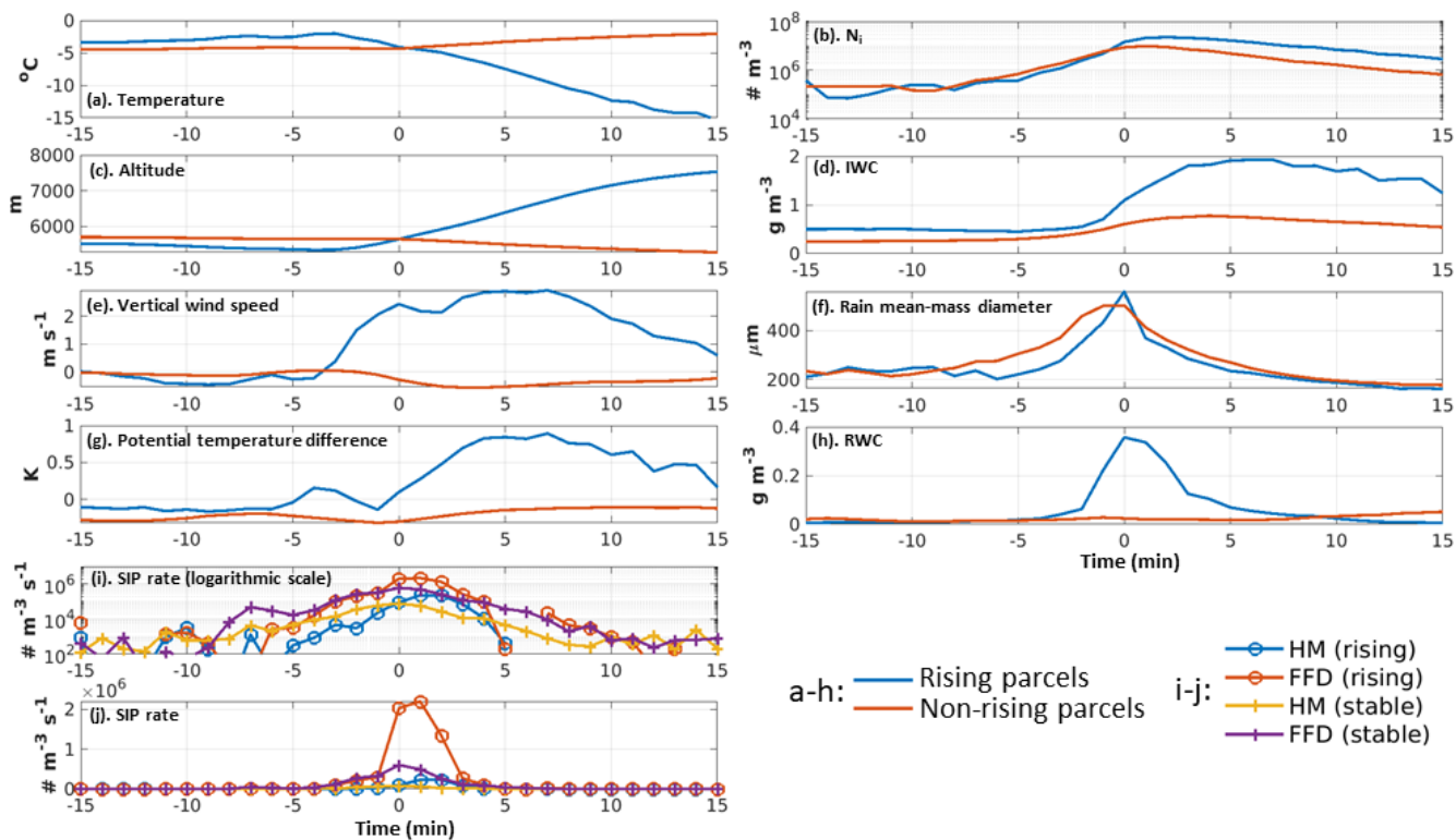
885 Figure 186: trajectory tracing of different variables for the rising parcels (blue lines in a-h) and the non-rising parcels (red lines in a-h). a: temperature, b: N_i , c: Altitude, d: IWC, e: vertical wind speed, f: rain mean-mass diameter, g: \Delta\theta , h: RWC, i: SIP tendency in logarithmic scale, j: SIP tendency in regular scale.
