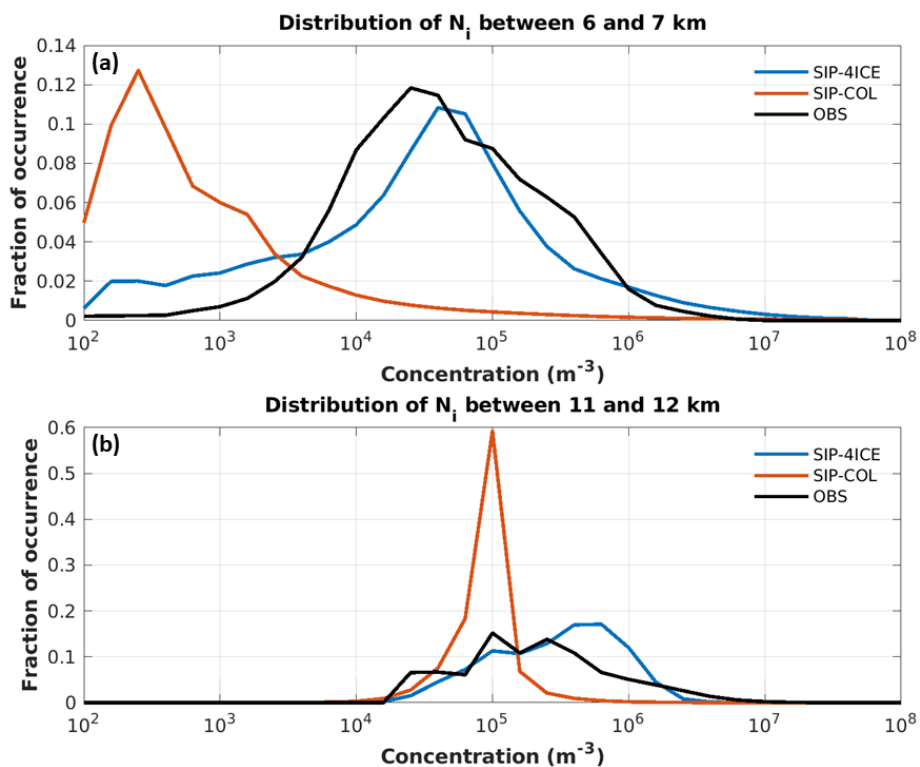
895 Figure 2048: Similar to Figure 8, but for different simulations: SIP-4ICE and SIP-COL.
