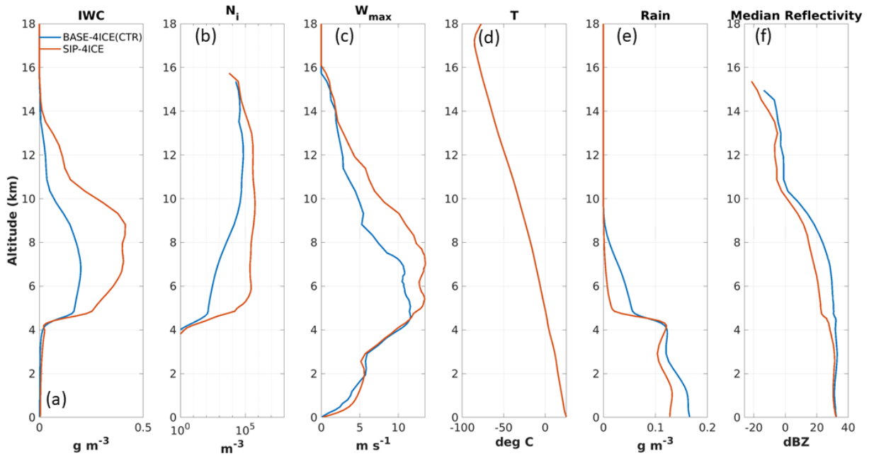
830 Figure 6: Same as Figure 4, but for baseline (CTR) simulation with 4 ice categories and the SIP simulation with 4 ice categories.
