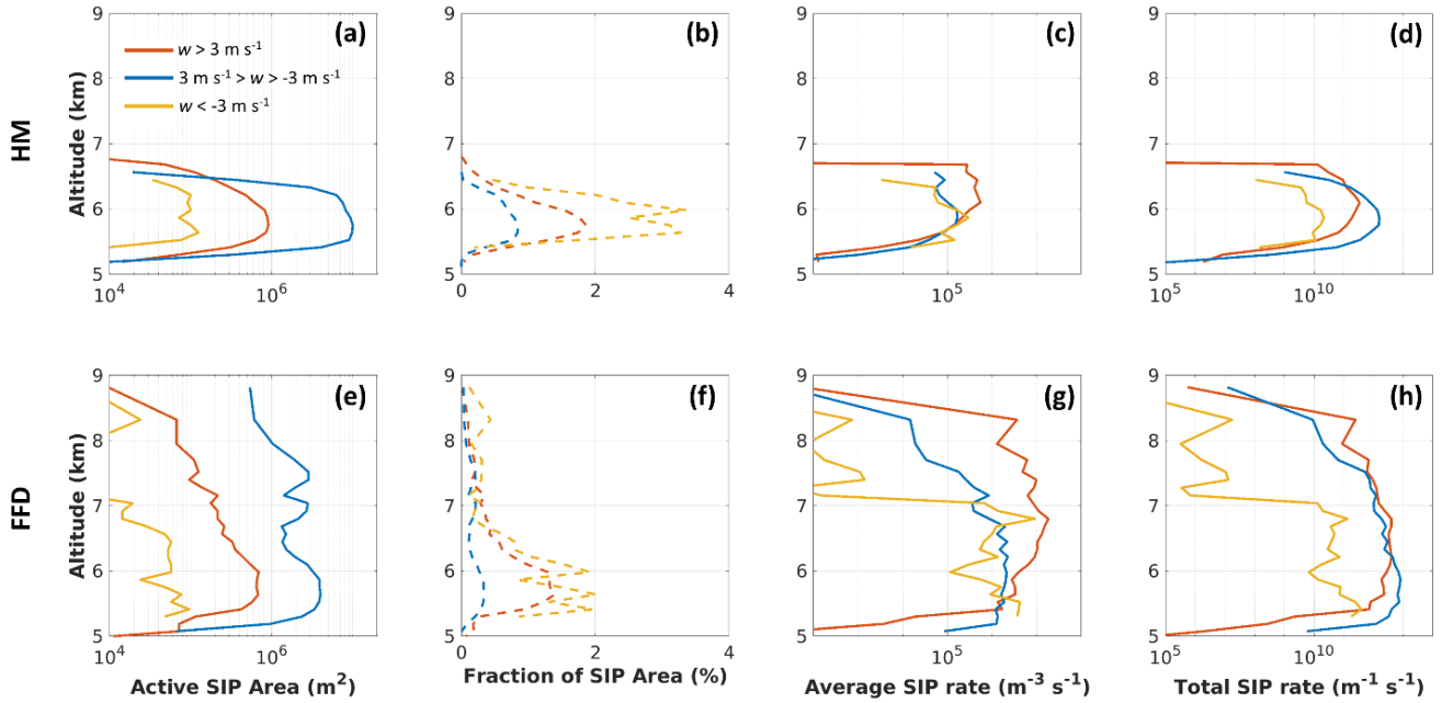
Figure 175. (a): area in \text{m}^2 with active HM process; (b): fraction of area with active HM process; (c): average rate of SIP by the HM process within the active area shown in (a); (d): total SIP rate, product of (a) and (b). (e) to (h): same as (a) to (d) but for the FFD process. Red lines (updrafts): SIP with w > 3 \text{ m s}^{-1} , blue lines (outside of updrafts/downdrafts): SIP with w between -3 and 3 \text{ m s}^{-1} , yellow lines (downdrafts): SIP with w < -3 \text{ m s}^{-1} . All results are temporal averages between 90 and 120 min.
