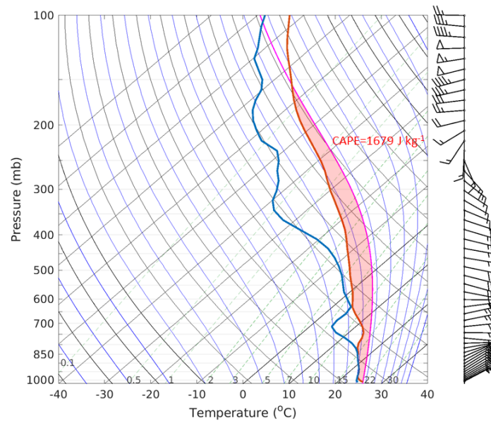
Figure 1: Initial atmospheric profiles for the idealized simulations. Blue line: dew point temperature. Red line: environment 805 sounding (temperature). Magenta line: parcel lapse rate.
