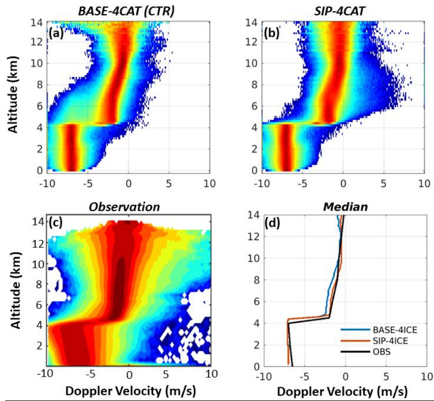
875 Figure 164. Same for Figure 12 but for the Doppler velocity.
