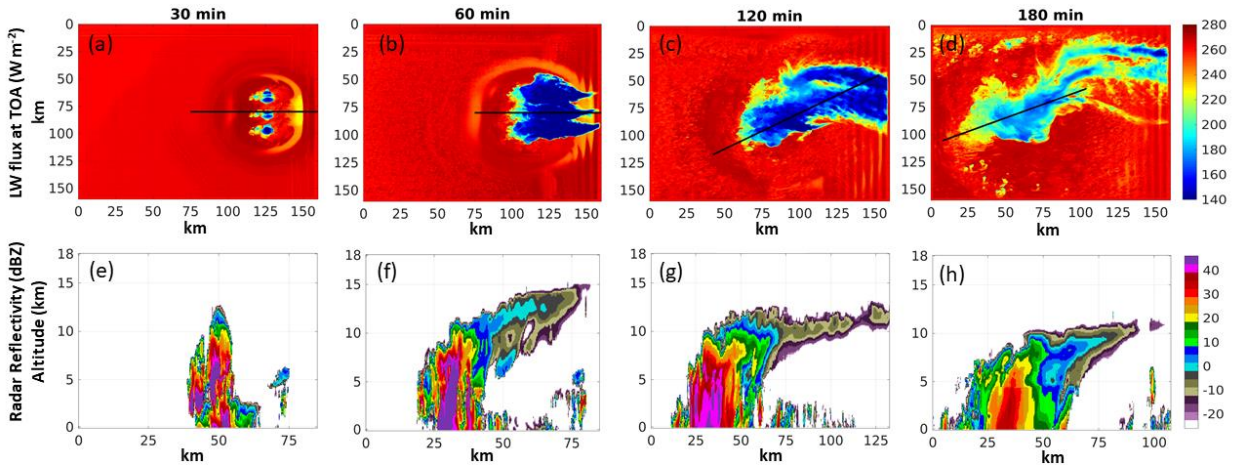
Figure 3: Simulation with a single ice category in the P3 bulk microphysics scheme. a-d: upward longwave radiative flux at the top of atmosphere at for different times (30, 60, 120, 180 min after the model initiation). e-h: the corresponding radar reflectivity of the cross-section marked by the black line in a-d.
