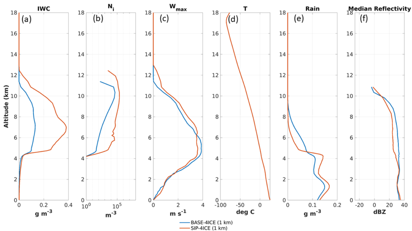
900 Figure 2220: Similar to Figure 6 but for simulation at 1 km horizontal grid spacing.
