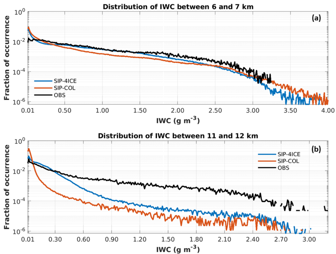
Figure 2149: Similar to Figure 9 but for different simulations: SIP-4ICE and SIP-COL.
