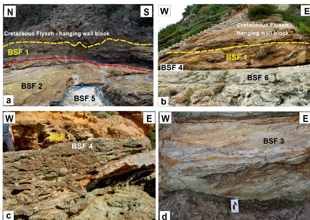
280 Figure 3: Field view of selected BSF's. a) and b) show examples of the complex internal architecture of the ZF with the tight juxtaposition of several BSF's. a) Northernmost exposed portion of the fault allowing access to an almost complete section of the fault zone. There the ZF is composed of a stack of three different BSF's and the hanging wall block on top. b) Sharp contact at Punta Zuccale between unit BSF 1 and BSF 6 separated by a thin layer of BSF 4. Note the meso-scale evidence of tectonic imbrication within BSF 1 indicating top-to-the E transport. This is not obvious in b) as the view there is in the direction of transport. c) Detail of 285 BSF 1 (above) to BSF 4 (below) contact. d) Pervasively foliated phyllonitic BSF 3.
