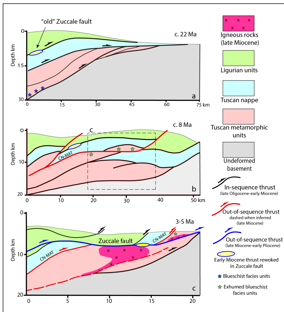
Figure 9: Cartoon illustrating the envisaged tectonic evolution of the northern Apennines belt for the early Miocene-early Pliocene time interval. Panel b) offers a zoom-in into panel a) at ca. 8 Ma ago. Panel c) zooms into panel b) and describes a possible scenario for the late Miocene-early Pliocene. Note that, for simplicity sake, the cartoons depict neither the effects of the intervening mid Miocene extensional phases nor those of the post Pliocene and still active extension. a) Early Miocene nappe stacking with development of east-vergent in-sequence thrusts. Deep metamorphic units experienced HP/LT blueschist facies metamorphism (0.9 – 1.5 GPa). b) Middle-late Miocene thrust reactivation and coeval development of east-vergent out-of-sequence thrusts that reshape the early Miocene nappe stack. Deep metamorphic units exhumed to greenschist facies conditions in the upper orogenic wedge are coupled with supracrustal non metamorphic or very low metamorphic grade units. c) Late Miocene-early Pliocene framework of central-eastern Elba island. The out-of-sequence Zuccale Fault cut the nappe stack and Porto Azzurro pluton. Musumeci and Vaselli (2012) and Papeschi et al. (2017) propose that the Porto Azzurro pluton emplaced within an overall compressional setting. Previous Tortonian out-of-sequence thrusts (e.g., the Capo Norsi – Monte Arco Thrust CN-MAT) were reactivated, cut across and displaced by the Zuccale Fault in the early Pliocene (< 4.9 Ma). The architecture of the northern Apennine belt on the Elba island was profoundly reshaped by the activity of multiple out-of-sequence thrusts spanning in age from late Miocene to early Pliocene.
