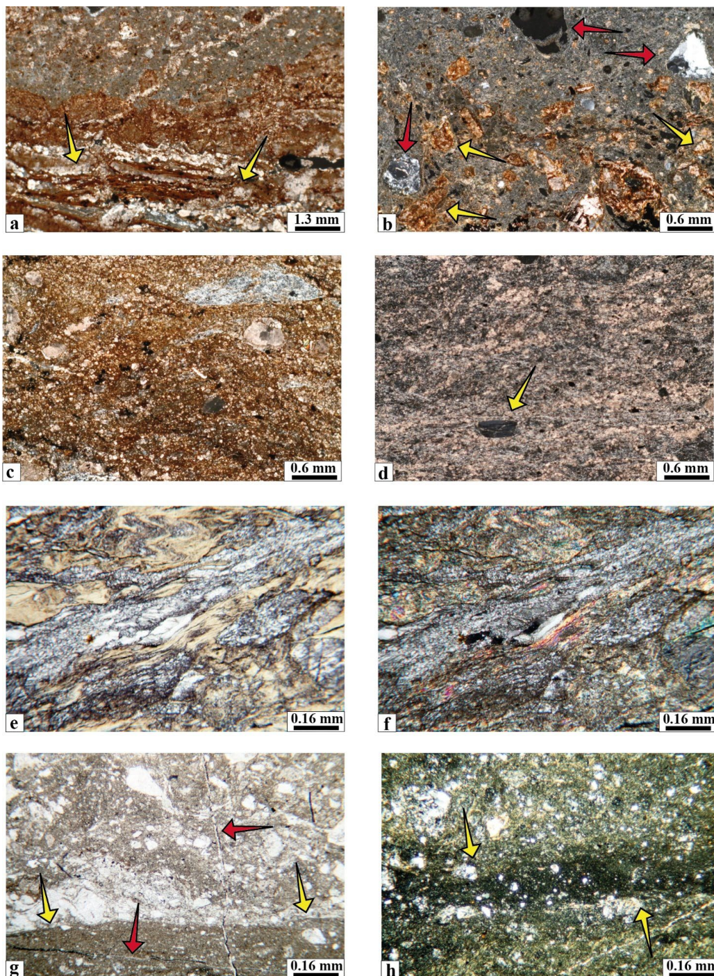
Figure 4: Microphotographs of representative examples of BSF fabrics. a – b): BSF1. a) Very fine-grained matrix with extensive crystallization of secondary calcite/dolomite with sparse embedded euhedral dolomite grains (grey layer, upper half of photo) and Fe-oxides and hydroxide alteration (reddish layer, lower half of photo). Relic foliated cataclastic domains (indicated by the yellow arrows) alternate with Fe-hydroxides bands and dolomite veins. Plane polarized light (PPL). b) Cataclasite with rare quartz-feldspar
