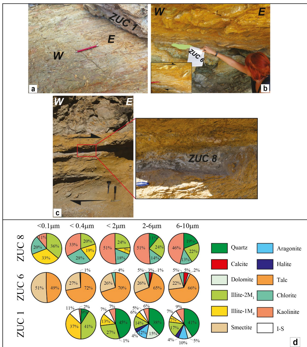
450 Figure 7: a-c) Sampled fault rocks and associated mesoscopic structures. ZUC 1 is from BSF 1 and comes from the immediate hanging wall of the ZF principal slip surface, which is decorated by pervasive E-W striae. ZUC 6 is from the uppermost part of BSF 3, which contains very clear top-to-the E kinematic indicators. ZUC 8 is from the easternmost exposed BSF 1, where clear top-to-the E kinematic indicators occur. d) Mineralogical composition of the separated grain-size fractions of the three dated samples.
