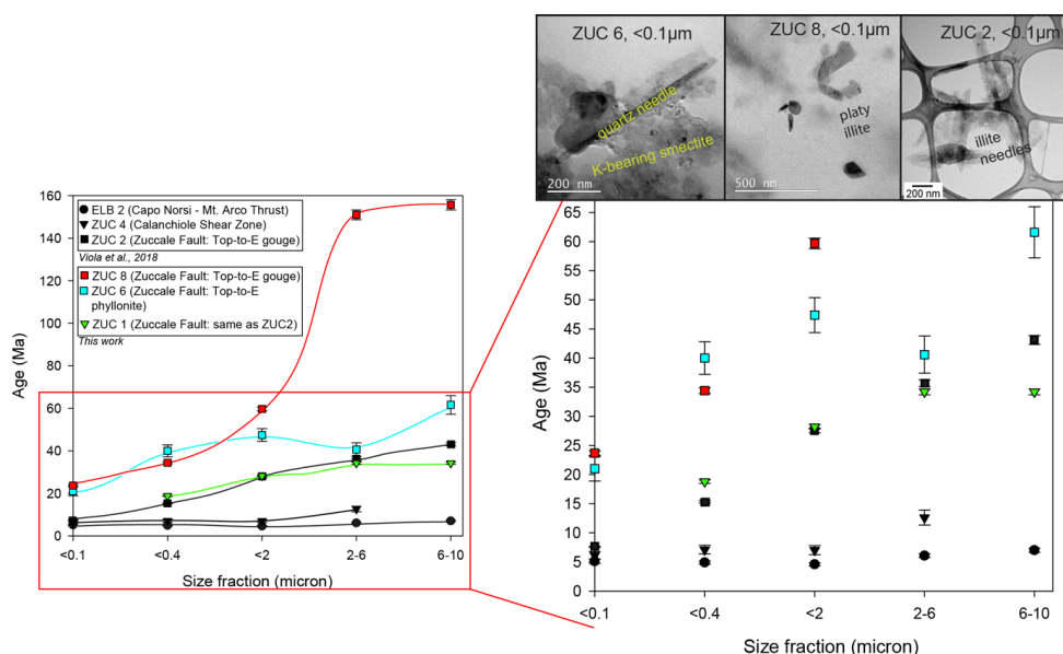
Figure 8: K-Ar age versus grain size spectra for the three dated samples (in colour) compared and contrasted with the results by Viola et al. (2018) in black. (b) Selected transmission electron microscope images of the finest dated fractions of ZUC 6 and ZUC 8 from this study. The image of ZUC 2 is from Viola et al. (2018).
