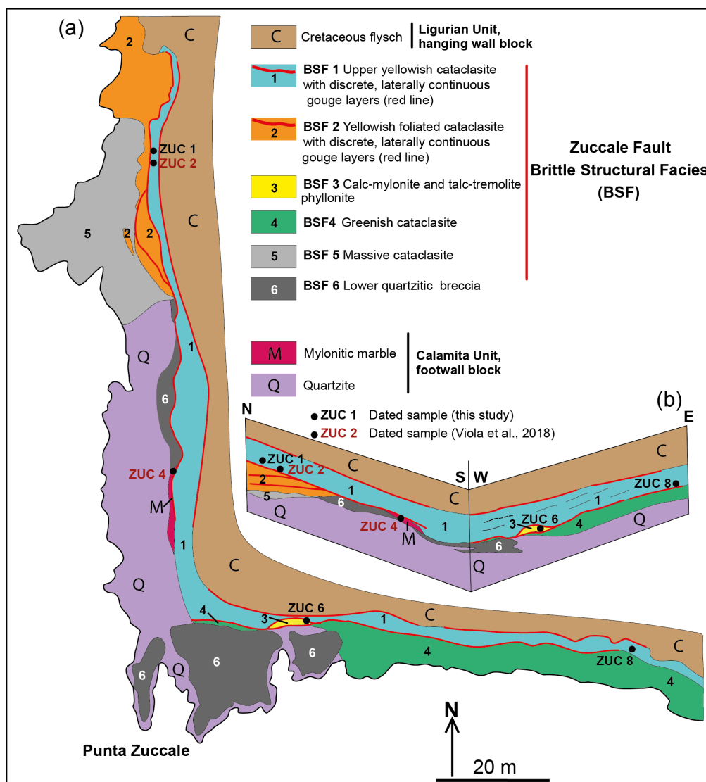
Figure 2: a) Geological map of Punta Zuccale showing the distribution of the Brittle Structural Facies (BSF) of the Zuccale Fault and the location and name of the samples dated in this study (in black) and in Viola et al. (2018; in red). b) Fence diagram illustrating fault rock distribution along the NS and EW natural cross-sections that are directly accessible along the shore line of Punta Zuccale.
