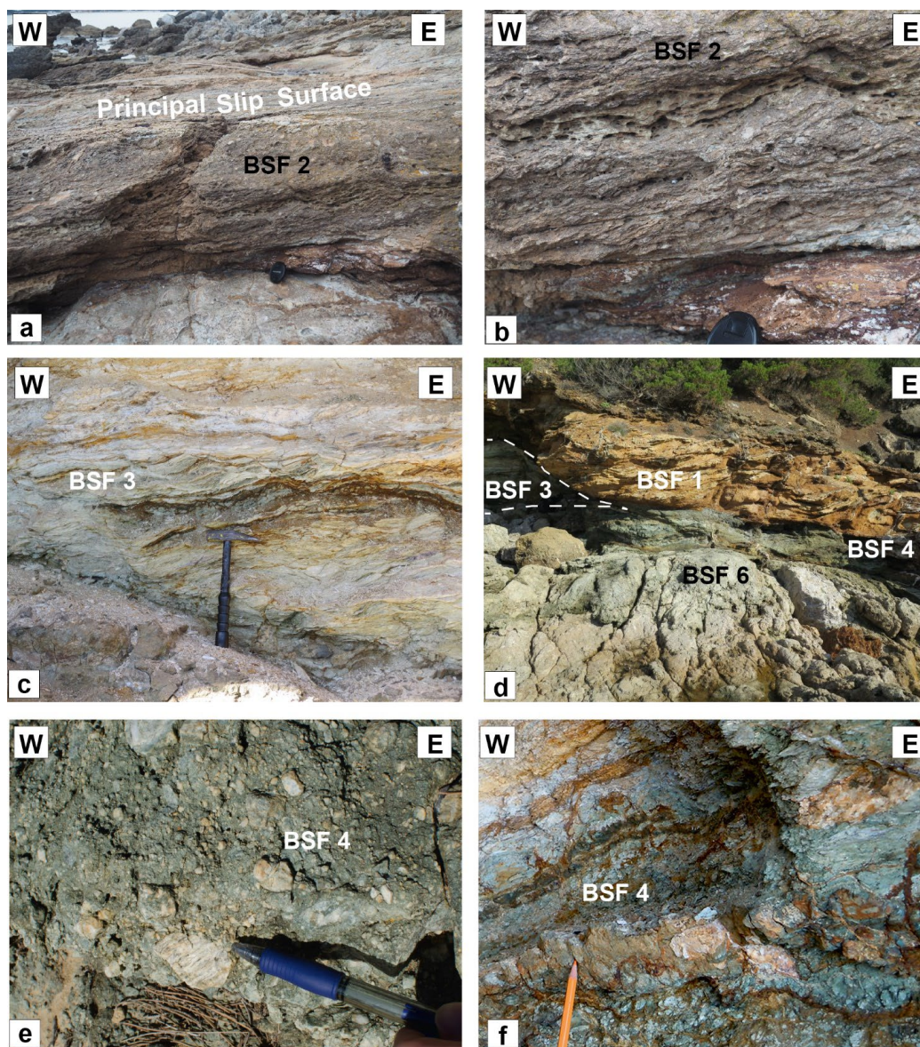
320 Figure 5: Outcrop view of fault rocks from different BSF's. a, b) BSF 2: a) upper yellowish cohesive cataclasite with W- gently dipping foliation capped by the subhorizontal ZF Principal Slip Surface. b) Detail of foliated cataclasite with oblique foliation indicating top-to-the E shearing. c) Compositionally banded phyllonite of BSF 3. Note the shear bands constraining top-to-the E along the subhorizontal foliation. d) Outcrop view of the complex spatial arrangement of four different BSF's at the western termination of the EW section at Punta Zuccale. Note the eastern lateral closure of BSF 3, which forms a metric lense in the complex architecture of the ZF (see Fig. 2). The width of the photograph corresponds to ca. 8-10 m. e) BSF 4 greenish cataclasite with millimetric angular to subrounded quartz clasts deriving from underlying Triassic quartzites, in a very fine grained matrix made up of ultracataclasite and gouges. f) Detailed view of a foliated gouge level within BSF 4. 325
