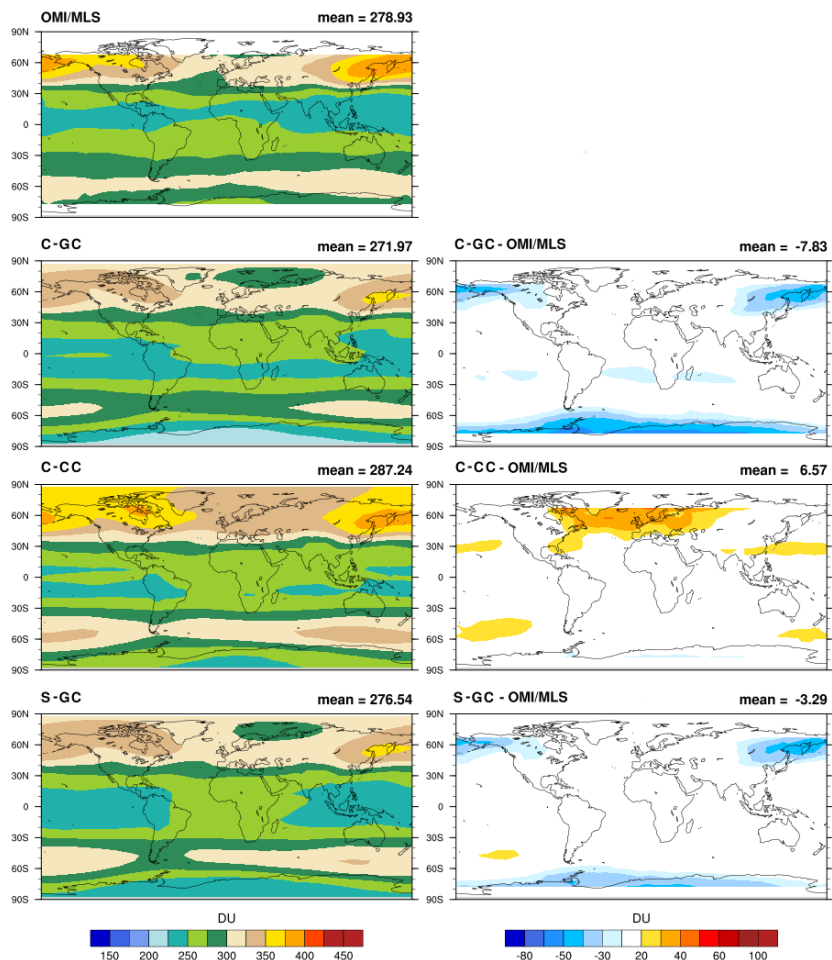
Figure 23. Total ozone column as observed by the Aura Ozone Monitoring Instrument (OMI) and Microwave Limb Sounder (MLS) for the 2004-2010 time period (1 st row), compared to the results from C-GC (2 nd row), C-CC (3 rd row), and S-GC (4 th row) for the year 2016. The measurements and model results are presented on the left, while the model biases are shown on the right.
