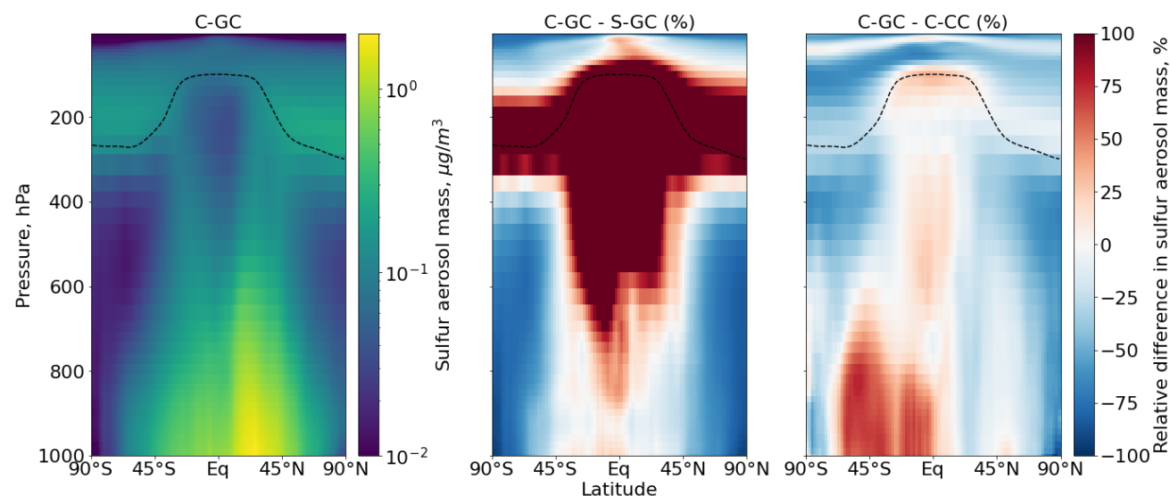
Figure 6. Comparison of sulfate aerosol mass concentration as simulated with CESM running GEOS-Chem (C-GC) to standalone GEOS-Chem (S-GC) and CESM running CAM-chem (C-CC). Left: absolute values estimated with C-GC. Center: relative difference between C-GC and S-GC. Right: relative difference between C-GC and C-CC. Red (blue) shading means that C-GC estimated a higher (lower) value than the other model. Differences are restricted to \pm 100\% for clarity.
