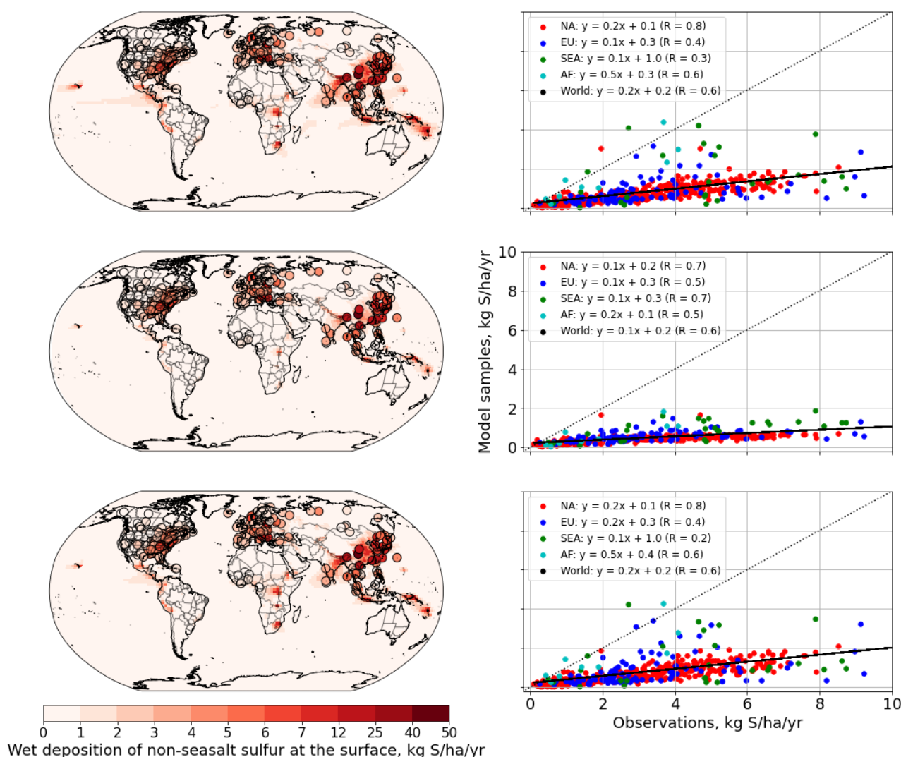
Figure 26. As in Figure 25, but now for non-sea salt sulfur. Rows: C-GC (top), S-GC (middle), and C-CC (bottom).
