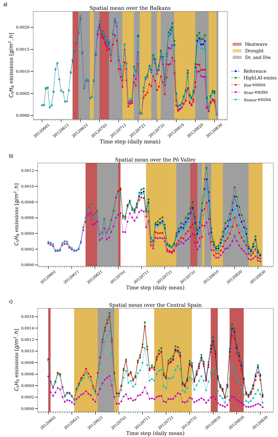
Figure 3. Daily mean C_5H_8 emissions [ g \cdot m^{-2} \cdot h^{-1} ] during the summer 2012, spatially averaged over the Balkans (a), Pô Valley (b) and Central Spain (c) for the different MEGAN experiments. The colored bands highlight periods of droughts and heatwaves.
