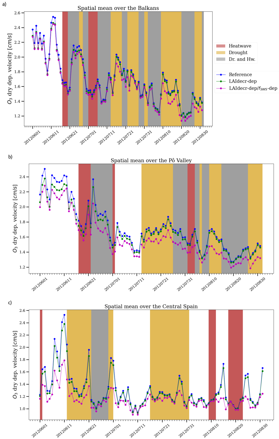
Figure 6. Daily mean O_3 dry deposition velocity [cm/s] during the summer 2012, spatially averaged over the Balkans (a), Pô Valley (b) and Central Spain (c) for the different CHIMERE experiments.
