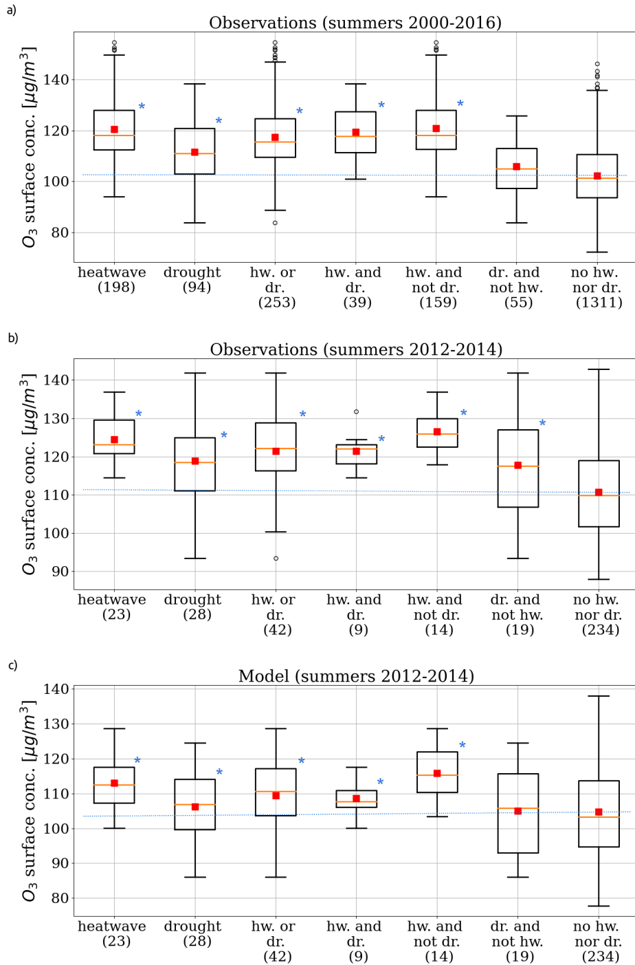
Figure 12. Same as Figure 10 with the observed surface O_3 concentration [ \mu\text{g}/\text{m}^3 ] over the summers 2000-2016 (a) and 2012-2014 (b), and with the simulated surface O_3 ("all-emiss-dep" experiment) over the summers 2012-2014 (c).
