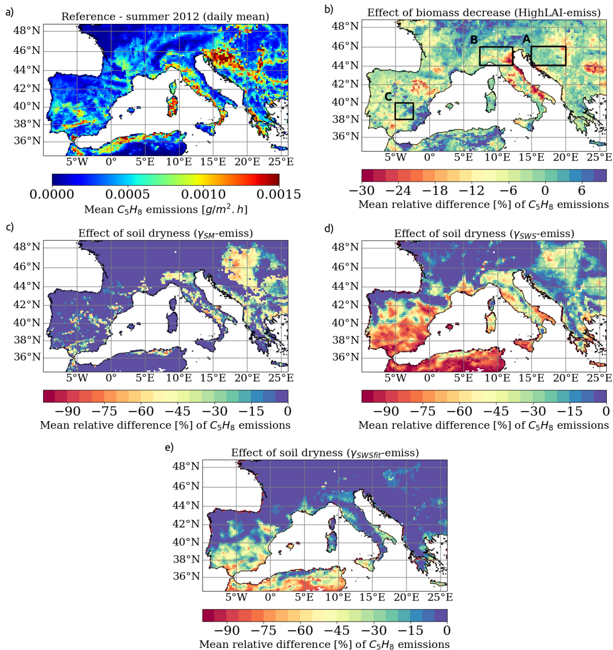
Figure 2. Summer mean (JJA) of daily mean C_5H_8 emissions [ g \cdot m^{-2} \cdot h^{-1} ] for 2012 from the "Reference" simulation (a). Mean relative difference [%] of C_5H_8 emissions due to biomass decrease and soil dryness. The relative difference is computed between the "Reference" and "HighLAI-emiss" simulation to quantify the biomass decrease effect (b) and the " \gamma_{SM} -emiss" (c), " \gamma_{SWS} -emiss" (d), " \gamma_{SWSfit} -emiss" (e) simulation to quantify the soil dryness effect (for each configuration). For diagnostic purposes, areas of interest are designated within the dashed rectangles: here named as the "Balkans" (A), "Pô Valley" (B) and "Central Spain" (C).
