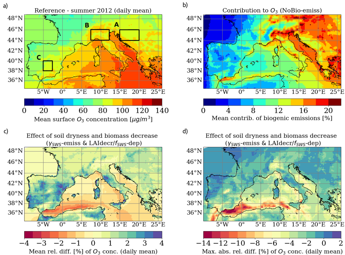
Figure 8. Summer mean (JJA) of daily mean O_3 surface concentration [ \mu g/m^3 ] for 2012 from the "Reference" simulation (a). Mean contribution of biogenic emissions to O_3 surface concentration based on the "NoBio-emiss" experiment (b). Mean (c) and maximum absolute (d) relative difference [%] of O_3 surface concentration due to biomass decrease and soil dryness. The relative difference is computed between the "Reference" and " \gamma_{SWS-emiss} & LAI_{decr}/f_{SWS-dep} " simulation from CHIMERE.
