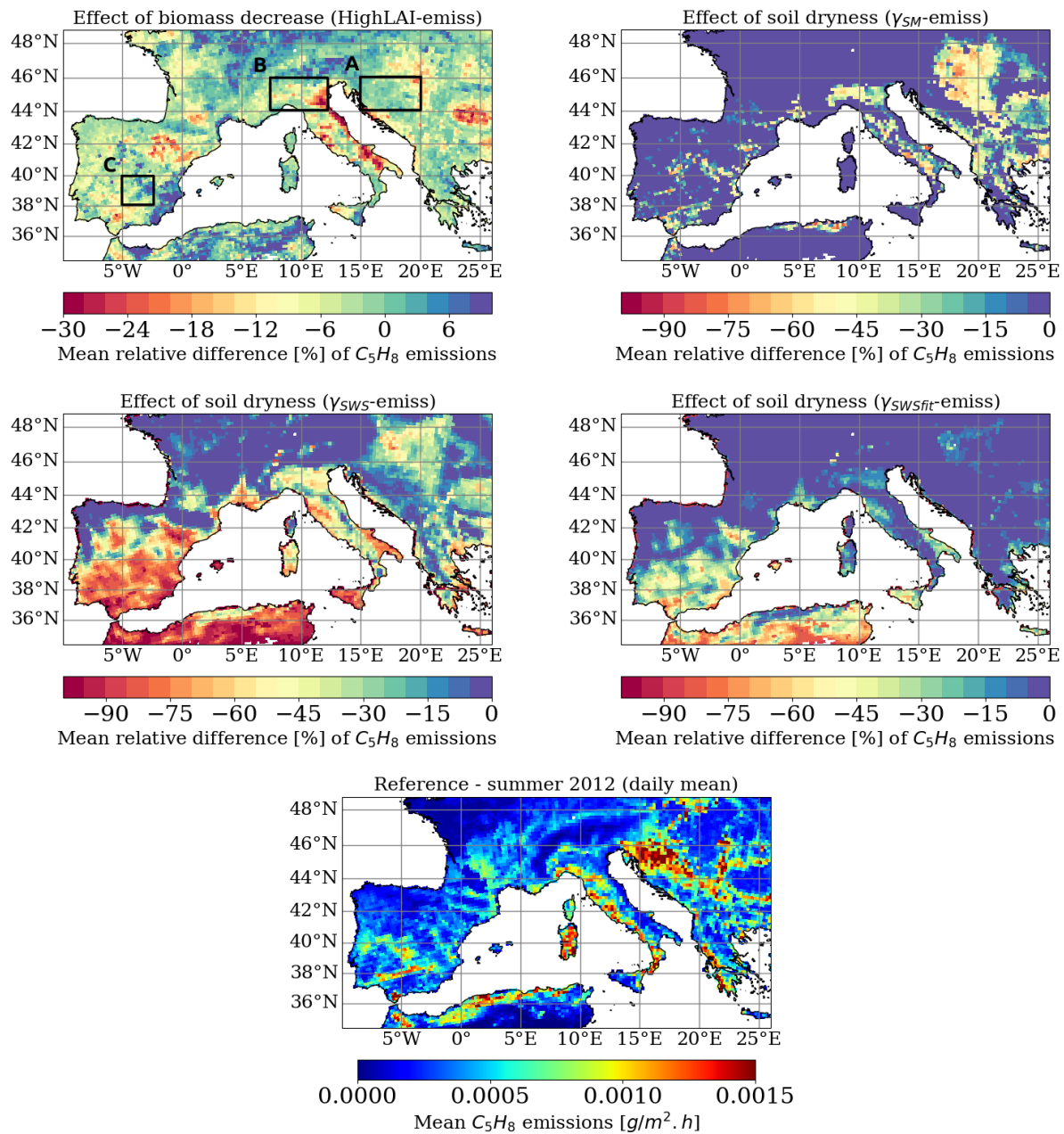
Figure 2. Summer mean (JJA) of daily mean C_5H_8 emissions [ g \cdot m^{-2} \cdot h^{-1} ] for 2012 from the "Reference" simulation (lower panel). Mean relative difference [%] of C_5H_8 emissions due to biomass decrease and soil dryness. The relative difference is computed between the "Reference" and "HighLAI-emiss" simulation to quantify the biomass decrease effect (upper left panel), and " \gamma_{SM} -emiss"/" \gamma_{SWS} -emiss"/" \gamma_{SWSfit} -emiss" to quantify the soil dryness effect. For diagnostic purposes, areas of interest are designated within the dashed rectangles: here named as the "Balkans" (A), "Pô Valley" (B) and "Central Spain" (C).
