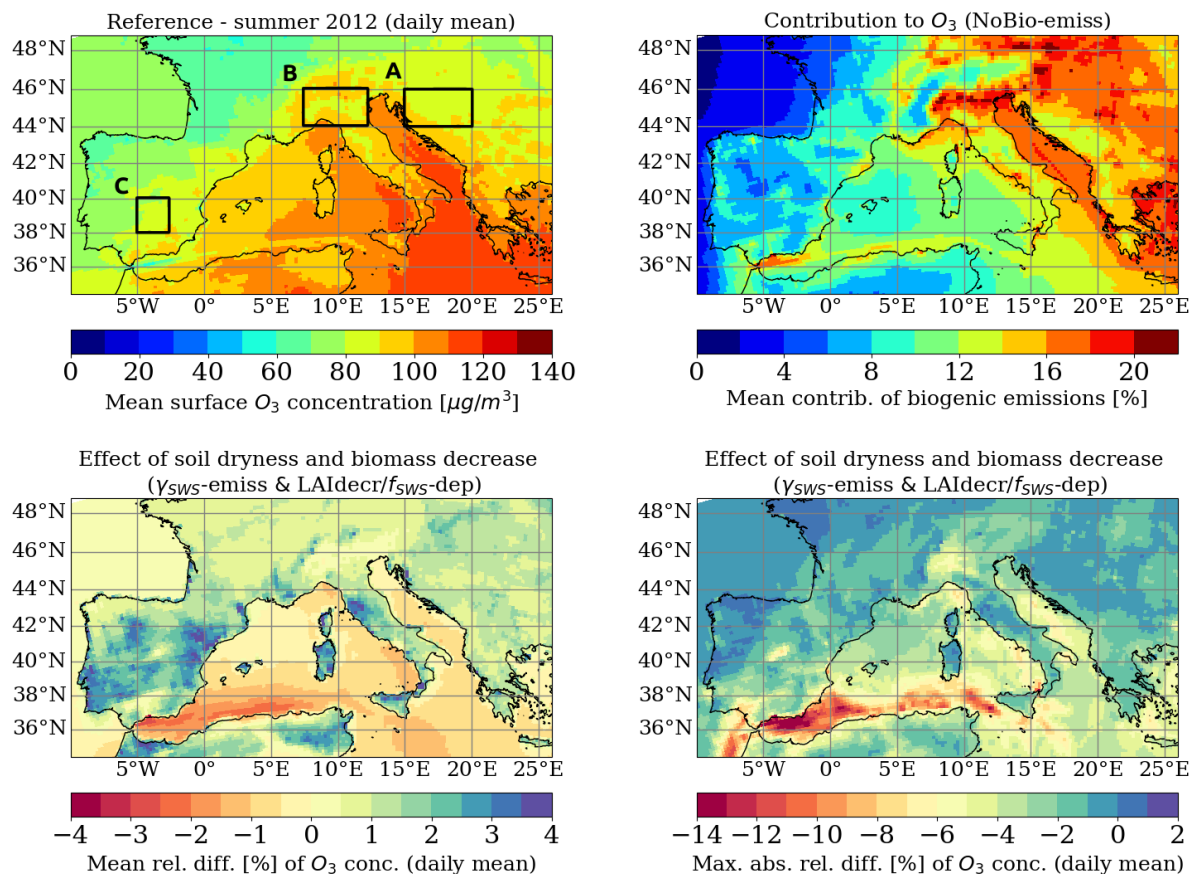
Figure 8. Summer mean (JJA) of daily mean O_3 surface concentration [ \mu\text{g}/\text{m}^3 ] for 2012 from the "Reference" simulation (upper left panel). Mean contribution of biogenic emissions to O_3 surface concentration based on the "NoBio-emiss" experiment (upper right panel). Mean (lower left panel) and maximum absolute (lower right) relative difference [%] of O_3 surface concentration due to biomass decrease and soil dryness. The relative difference is computed between the "Reference" and " \gamma_{SWS} -emiss & LAIdecr- f_{SWS} -dep" simulation from CHIMERE.
