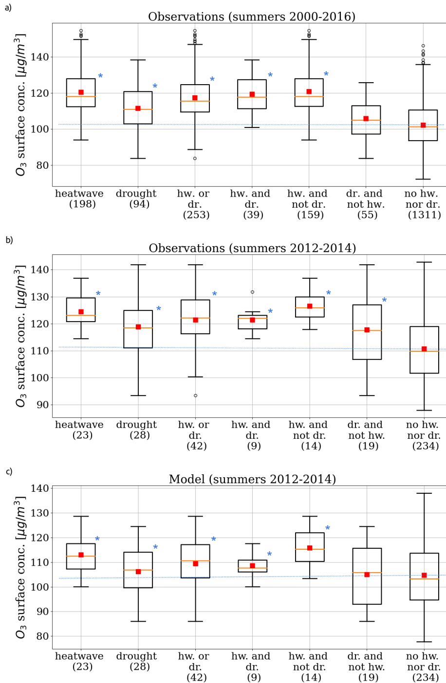
Figure 12. Same as Figure 10 with the observed surface O_3 concentration [ \mu g/m^3 ] over the summers 2000-2016 (upper-panel a) and 2012-2014 (middle-panel b), and with the simulated surface O_3 ("all-emiss-dep" experiment) over the summers 2012-2014 (lower-panel c).
