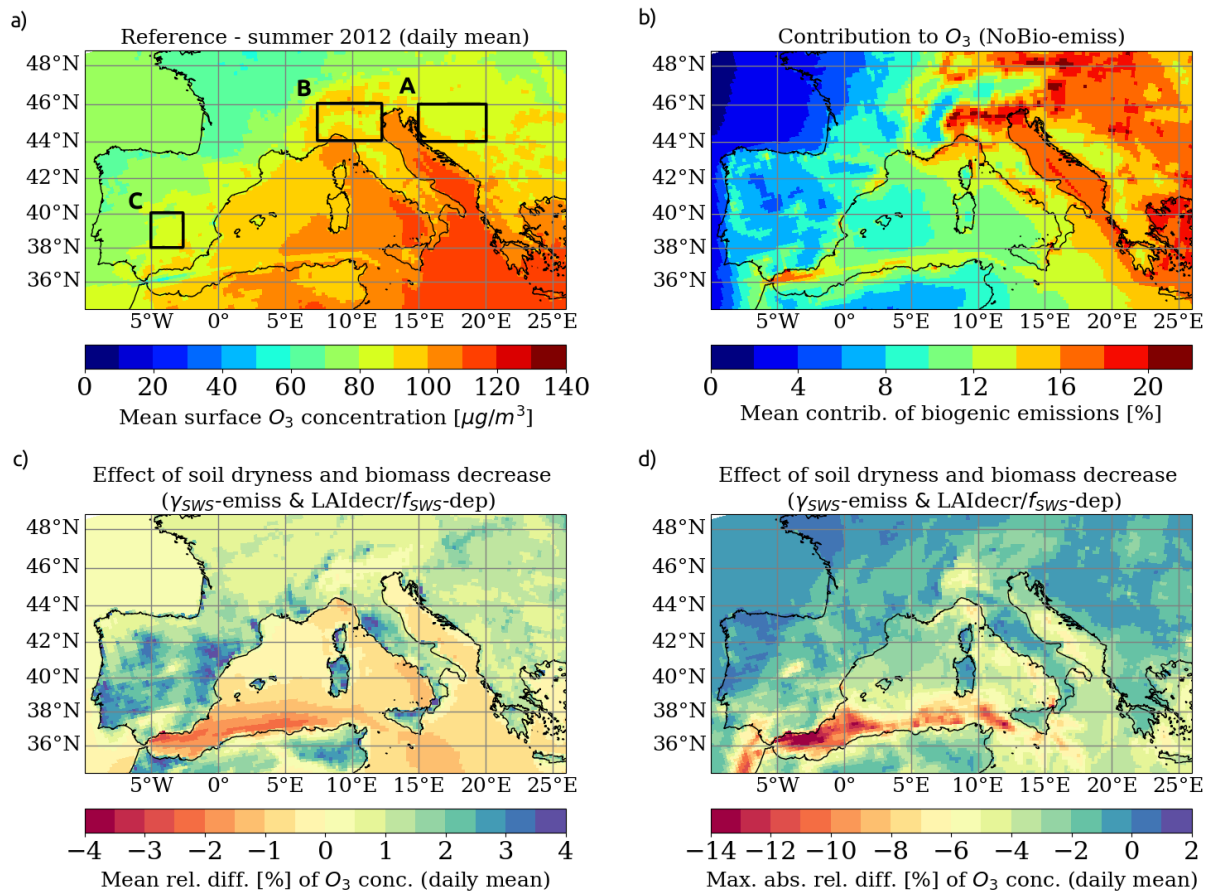
Figure 8. Summer mean (JJA) of daily mean O_3 surface concentration [ \mu g/m^3 ] for 2012 from the "Reference" simulation (upper-left panela). Mean contribution of biogenic emissions to O_3 surface concentration based on the "NoBio-emiss" experiment (upper-right panelb). Mean (lower-left panelc) and maximum absolute (lower-right panel d) relative difference [%] of O_3 surface concentration due to biomass decrease and soil dryness. The relative difference is computed between the "Reference" and " \gamma_{SWS-emiss} & LAIdecr/ f_{SWS-dep} " simulation from CHIMERE.
