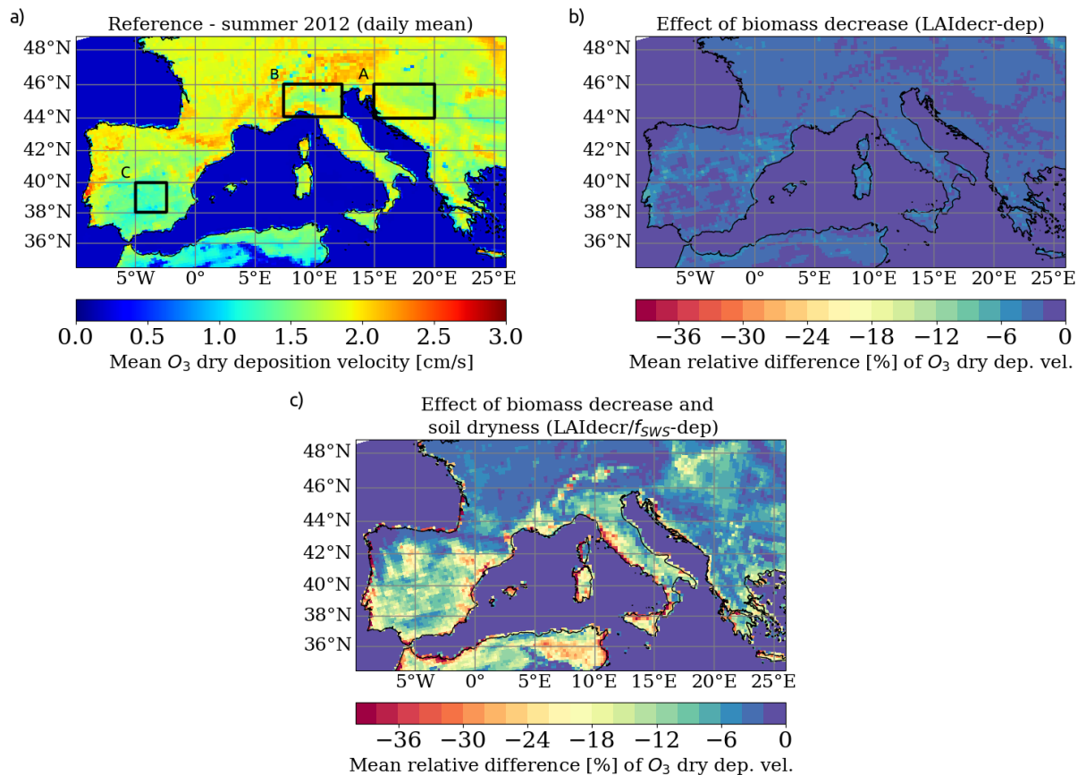
Figure 5. Summer mean (JJA) of daily mean O_3 dry deposition velocity [ cm/s ] for 2012 from the "Reference" simulation ( upper-left panel ). Mean relative difference [%] of O_3 dry deposition velocity due to biomass decrease and soil dryness. The relative difference is computed between the "Reference" and "LAIdcr-dep" simulation to quantify the biomass decrease effect ( upper-right panel ) and "LAIdcr-dep/ f_{SWS} -dep" to quantify combined biomass decrease and soil dryness effect ( lower panel ).
