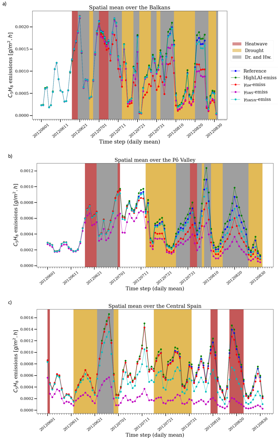
Figure 3. Daily mean C_5H_8 emissions [ g \cdot m^{-2} \cdot h^{-1} ] during the summer 2012, spatially averaged over the Balkans (upper-panel a), Pô Valley (middle-panel b) and Central Spain (lower-panel c) for the different MEGAN experiments. The colored bands highlight periods of droughts and heatwaves.
