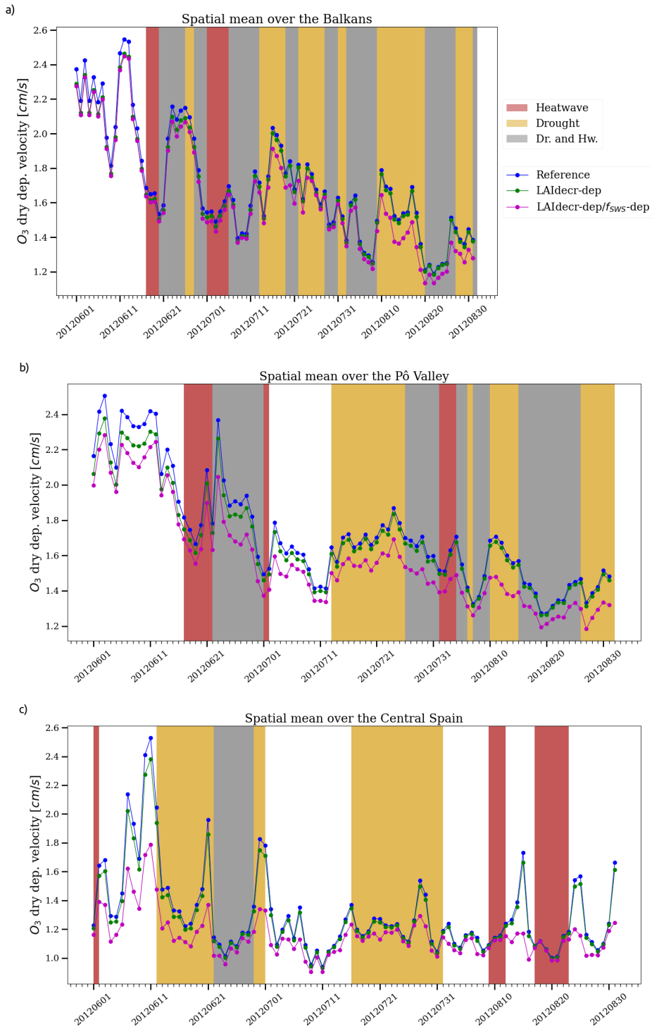
Figure 6. Daily mean O_3 dry deposition velocity [cm/s] during the summer 2012, spatially averaged over the Balkans (upper-panel a), Pô Valley (middle-panel b) and Central Spain (lower-panel c) for the different CHIMERE experiments.
