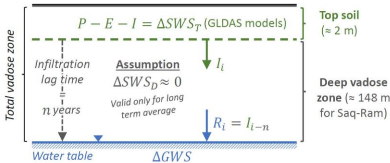
640 Figure 6: Conceptual representation of the treatment of the vadose zone in the GRACE-GLDAS water budget approach.
