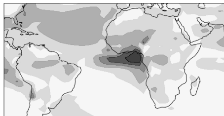
(b) O 3 inter-model SD
