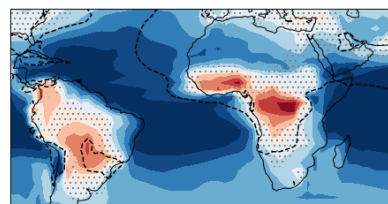
(e) MRI O 3
