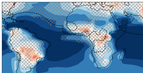
(a) O 3 due to climate change
