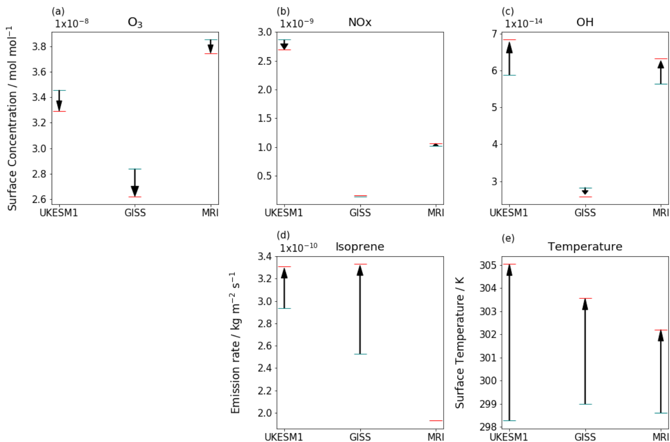
Figure 2: The change in surface concentration of (a) O 3 , (b) NO x , (c) OH, and the change in (d) isoprene emission rate and (e) surface temperature from experiment ssp370pdSST with no climate change (blue line) to experiment ssp370SST with climate change (red line) for the three climate models in this study. Variables have been averaged over the African and South American continents between 12° N–30° S for the period 2090–2100. The change due to climate change is significant at the 5% level for all variables and models except isoprene in MRI (which is prescribed so does not change).
