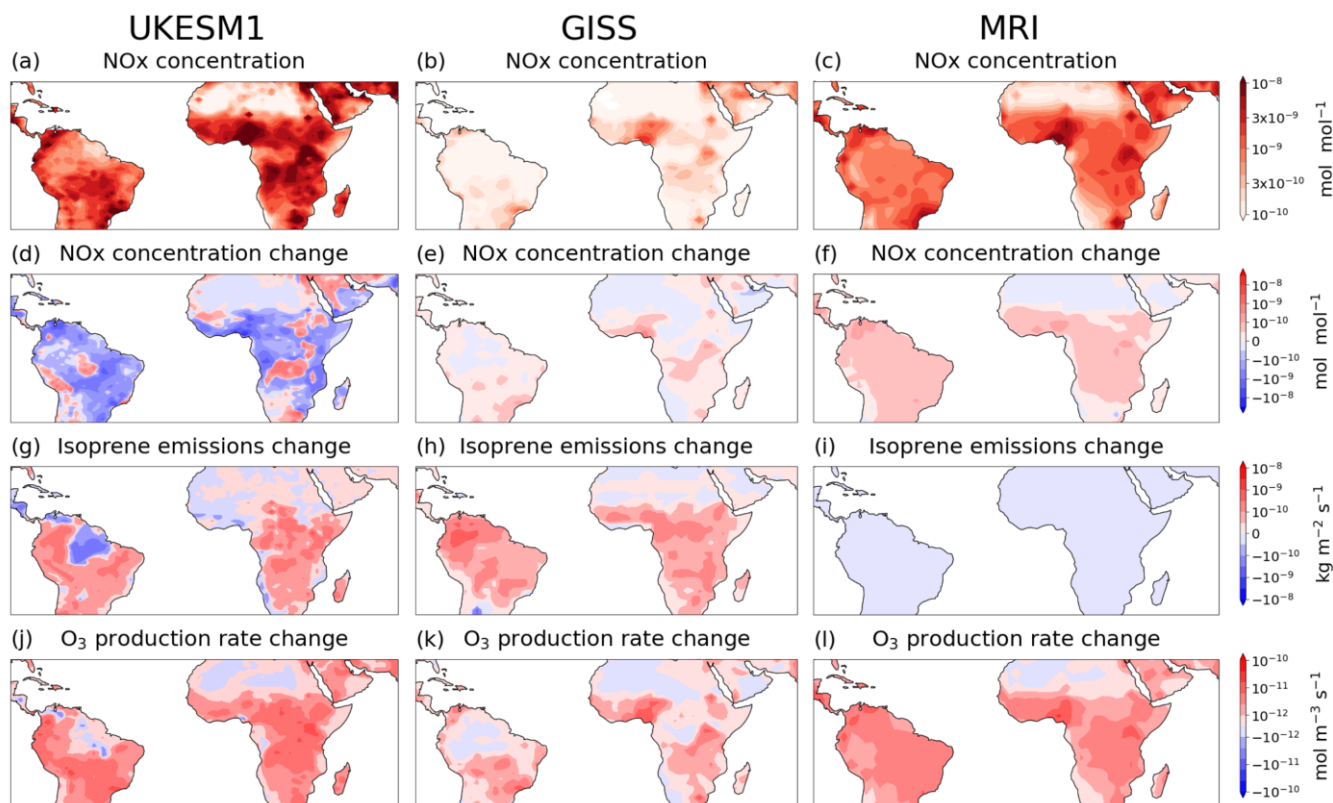
465 Figure 6: (a), (b), (c) Surface NO x concentrations in the absence of climate change and the average change due to climate change in (d), (e), (f) NO x concentration, (g), (h), (i) isoprene emission rate and (j), (k), (l) O 3 production rate for the period 2090–2100 for (column 1) UKESM1, (column 2) GISS and (column 3) MRI.
