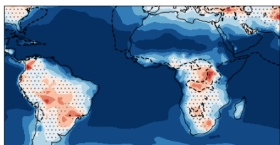
(c) UKESM1 O 3
