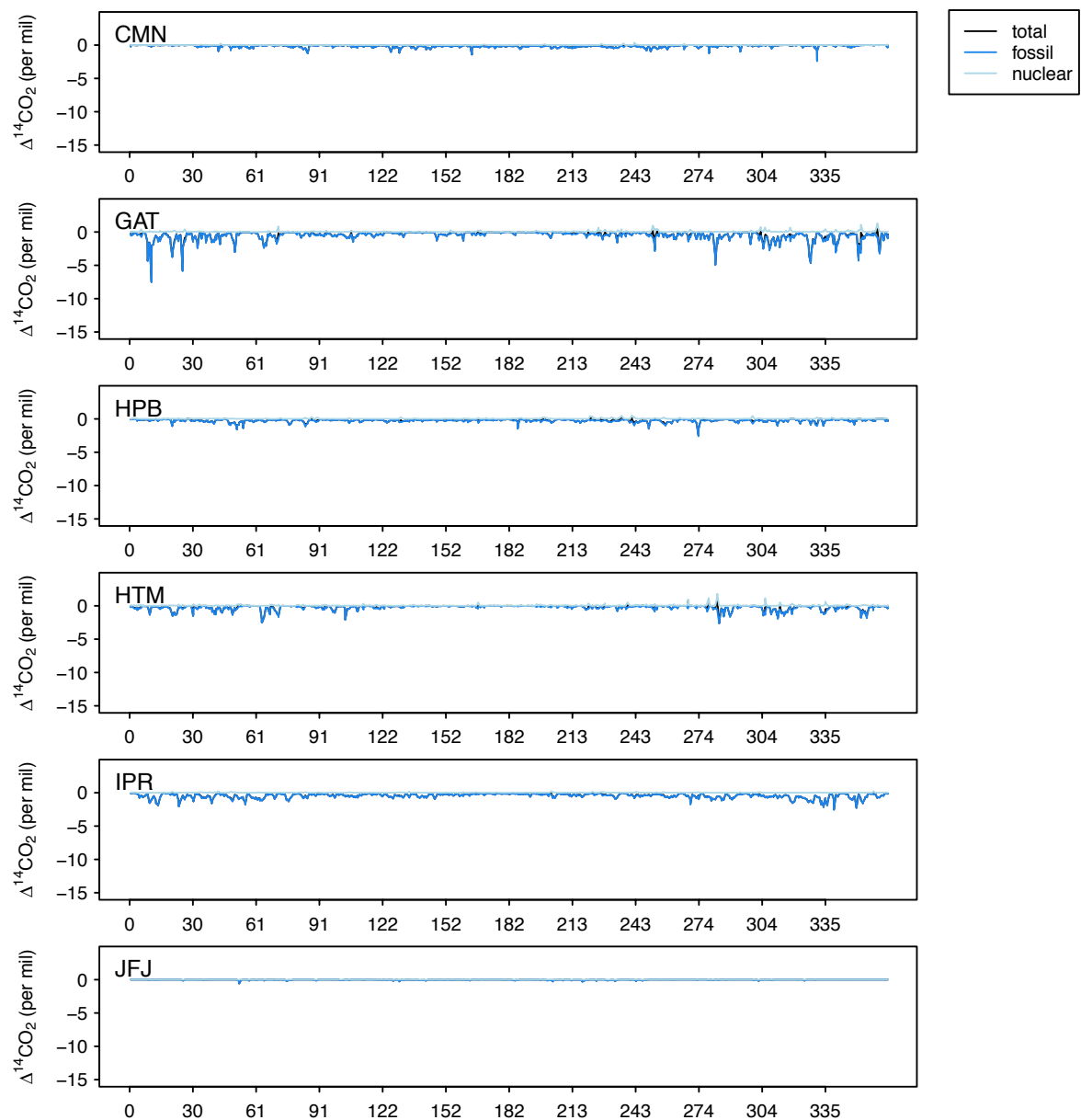
Figure S1. \Delta^{14}\text{CO}_2 variations at each site in the ICOS network simulated hourly from 12:00 to 15:00 every day for one year (the x-axis is day of the year).
