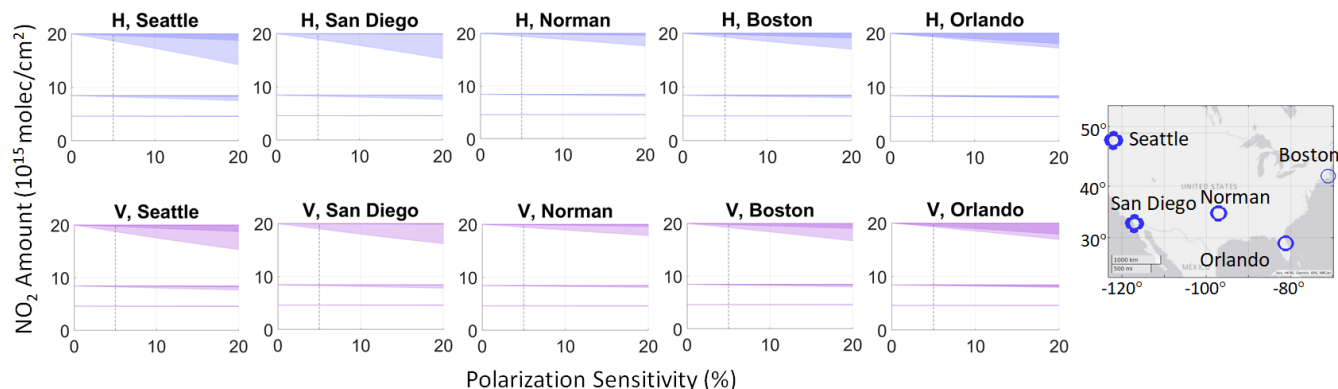
Figure 8. (Left) The retrieved amount is shown as a function of polarization sensitivity (PS) for two different orientations (H - horizontal, V - vertical) for selected US locations and \text{NO}_2 total vertical amounts: 5.0, 8.6, and 20 \times 10^{15} molecules/cm 2 . The edge of the darker (lighter) shading shows the retrieved \text{NO}_2 amount with a solar zenith angle of 30° (70°). The vertical dotted line shows the current PS requirement for reference. (Right) The locations are shown on the map with thicker circles representing higher \text{NO}_2 errors. (See Table 3, Simulation C for more details)
