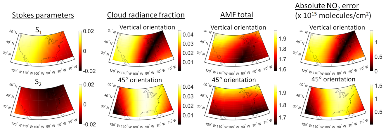
Figure 6. Derived parameters for \text{NO}_2 amount of 20 \times 10^{15} \text{ molecules/cm}^2 , water scenes, and 5% PS in a vertical and 45^\circ orientation. (See Table 3, Simulation A for more details).
