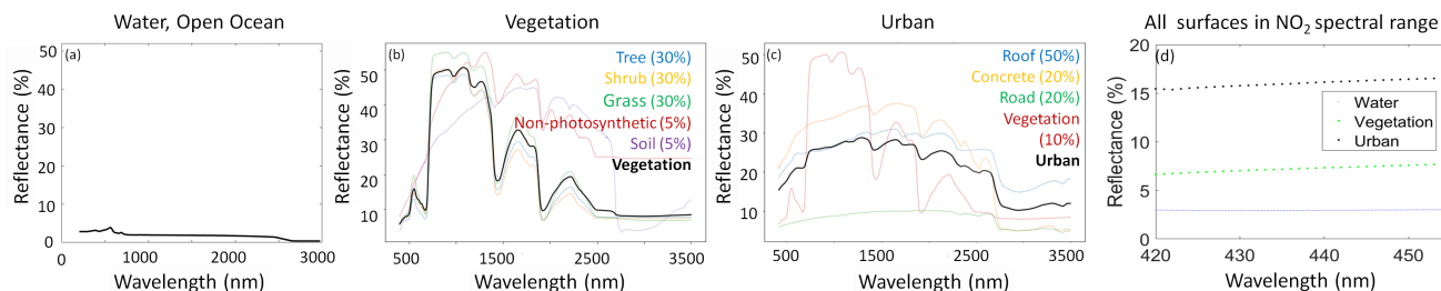
Figure 2. Basic surfaces reflectance spectra used in radiative transfer simulations: (a) water, (b) vegetation and (c) urban. (d) Spectra in the NO 2 retrieval spectral range.
