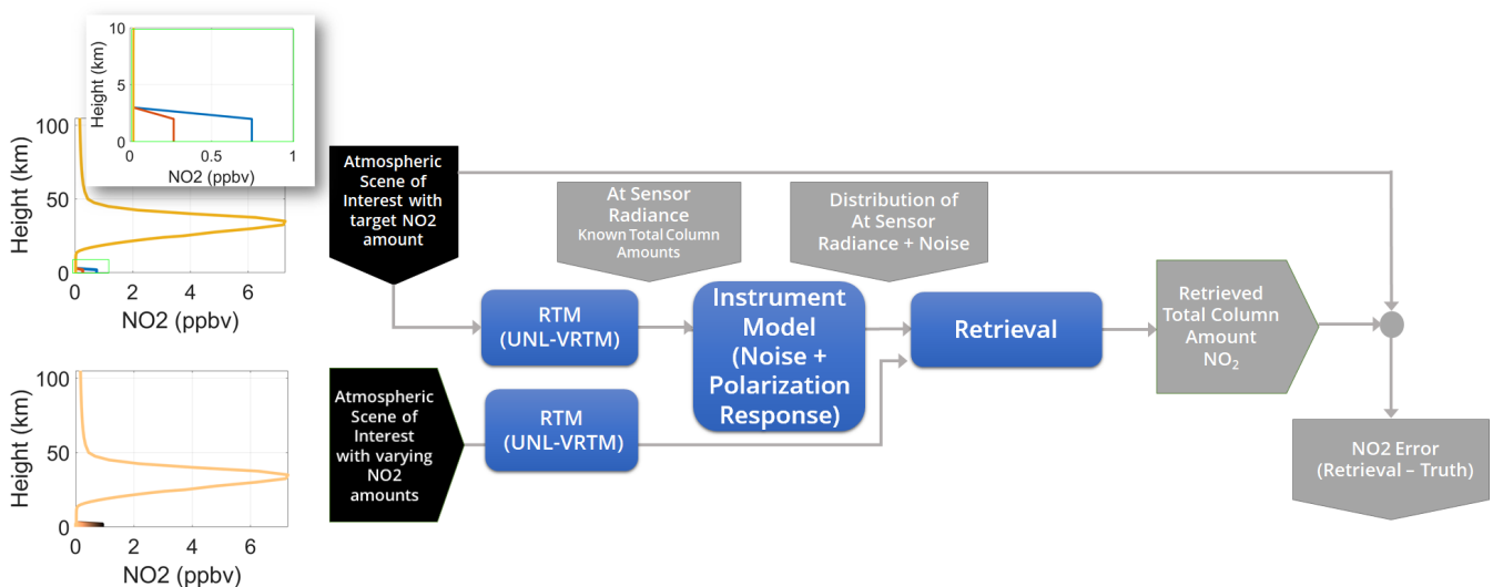
Figure 1. Simulation method for retrieving \text{NO}_2 in clear scenes: The scenes of interest consist of selected custom \text{NO}_2 profiles to represent low, medium, and high \text{NO}_2 cases shown at the upper left (including a zoomed-in view) corresponding to total vertical \text{NO}_2 amounts of 4.60, 5.93, and 8.44 \times 10^{15} molecules/cm 2 , respectively. The lower left profiles contain all profiles used in the retrieval process. The profiles are used in the radiative transfer model (RTM) called the Unified Linearized Vector Radiative Transfer Model (UNL-VRM) to generate at-sensor radiance.
