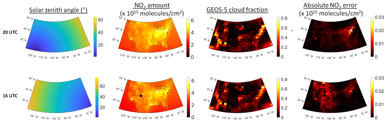
Figure 9. Solar zenith angles, total \text{NO}_2 column amount, GOES-5 cloud fraction, and resulting \text{NO}_2 errors at 20 UTC (top) and 16 UTC (bottom). GEOS-5 \text{NO}_2 profiles were used assuming 5% PS with vertical orientation, all water scenes, and clouds at a 2 km altitude. (See Table 3, Simulation D for more details)
