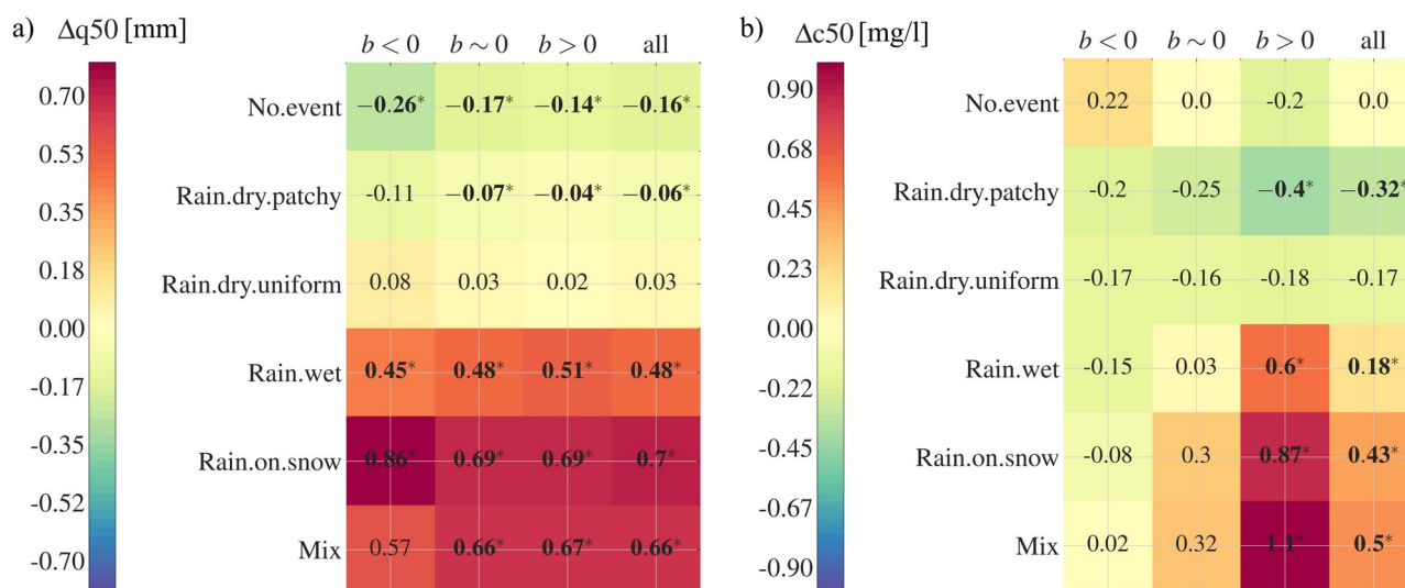
Figure S3. Heatmaps of differences between samples taken during different event types or No.event and all samples (analogous to Figure 5) for a) discharge and b) concentration of nitrate, averaged across different groups of catchments, considering all nitrate data for each event type and No.event. The three first columns of the heatmap correspond to one of the long-term export patterns (i.e., dilution (slope b < 0 ), neutral (slope b \sim 0 ) and enrichment (slope b > 0 )) and the fourth column corresponds to all study catchments. Bold font and * indicates significant differences (Kruskal-Wallis test, p < 0.05 ).
