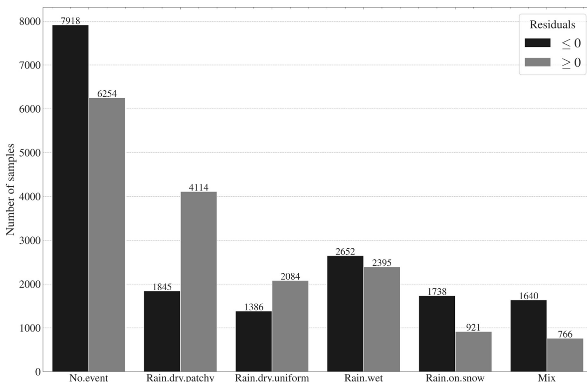
Figure S2: Number of nitrate samples from all catchments with positive and negative residuals for each event type.
