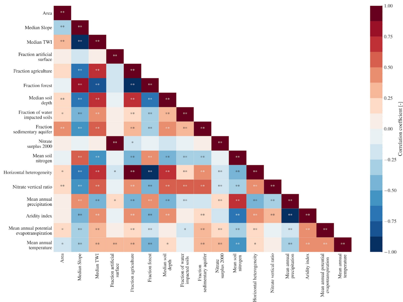
Figure S4. Spearman rank correlation coefficient between catchment descriptors. Significant correlations are indicated as * for p < 0.05 and ** for p < 0.01 .
