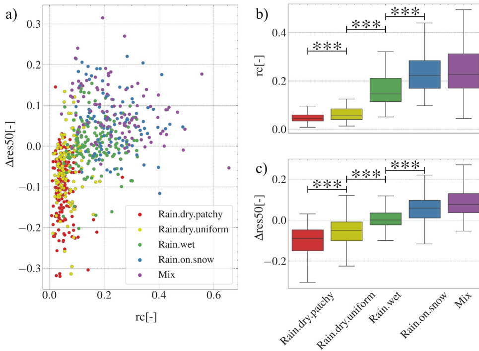
575 Figure 7: (a) Relationship between \Delta\text{res50} for each catchment and event type and median runoff coefficient (rc); runoff coefficient is not defined for No.event. (b) Variability of runoff coefficients (rc) for each event type and (c) median residuals for each event type. Significance of median differences between adjacent boxplots was estimated using Kruskal-Wallis test (displayed as *** for p < 0.001 ).
