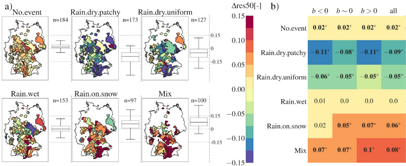
Figure 5: Median deviations of nitrate concentrations from the long-term C-Q relationships ( \Delta\text{res50} ) a) \Delta\text{res50} values of different event types for each catchment. On the right-hand side of each map, boxplots show the distribution of \Delta\text{res50} values across catchments for each event type (box limits represent the interquartile range and whiskers correspond to the 5th and 95th percentiles). b) Heatmap of \Delta\text{res50} values averaged across different groups of catchments, considering all nitrate data for each event type and No.event. The three first columns of the heatmap correspond to one of the long-term export patterns (i.e., dilution (slope b < 0 ), neutral (slope b \sim 0 ) and enrichment (slope b > 0 )) and the fourth column corresponds to all study catchments. Bold font and * indicates significant differences (Kruskal-Wallis test, p < 0.05 ) between median deviations across catchments for each event type and median deviation across catchments of all nitrate samples.
