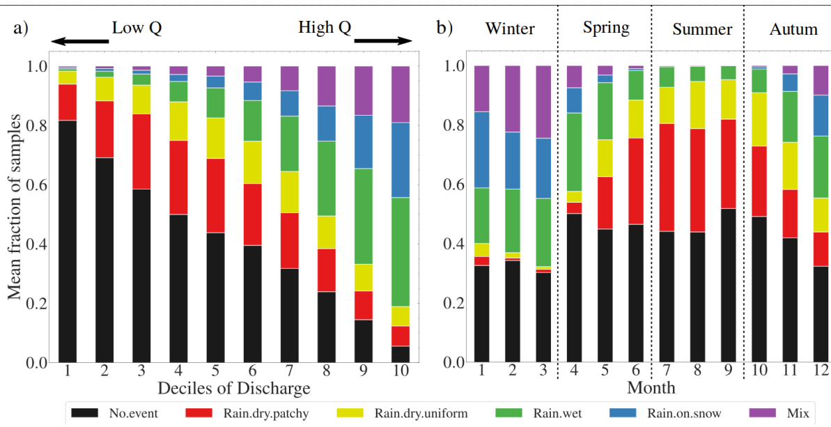
Figure 4: a) Mean fraction of samples linked to each event type according to each catchment decile of discharge, and b) seasonal distribution of mean fraction of samples linked to each event type in the study catchments.
