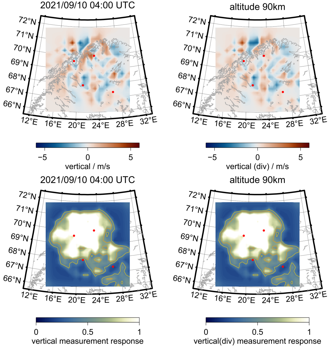
Figure 9. Corresponding vertical wind velocities (upper two panels) (left: compressible/non-stationary solution ) and measurement response (lower two panels) obtained by the 3DVAR+DIV algorithm for the same period as Figure 7. Note that the measurement response of the compressible/non-stationary vertical wind solution is dominated by the incompressible solution, which is used in all iterations due to the implemented horizontal divergence constraint.
