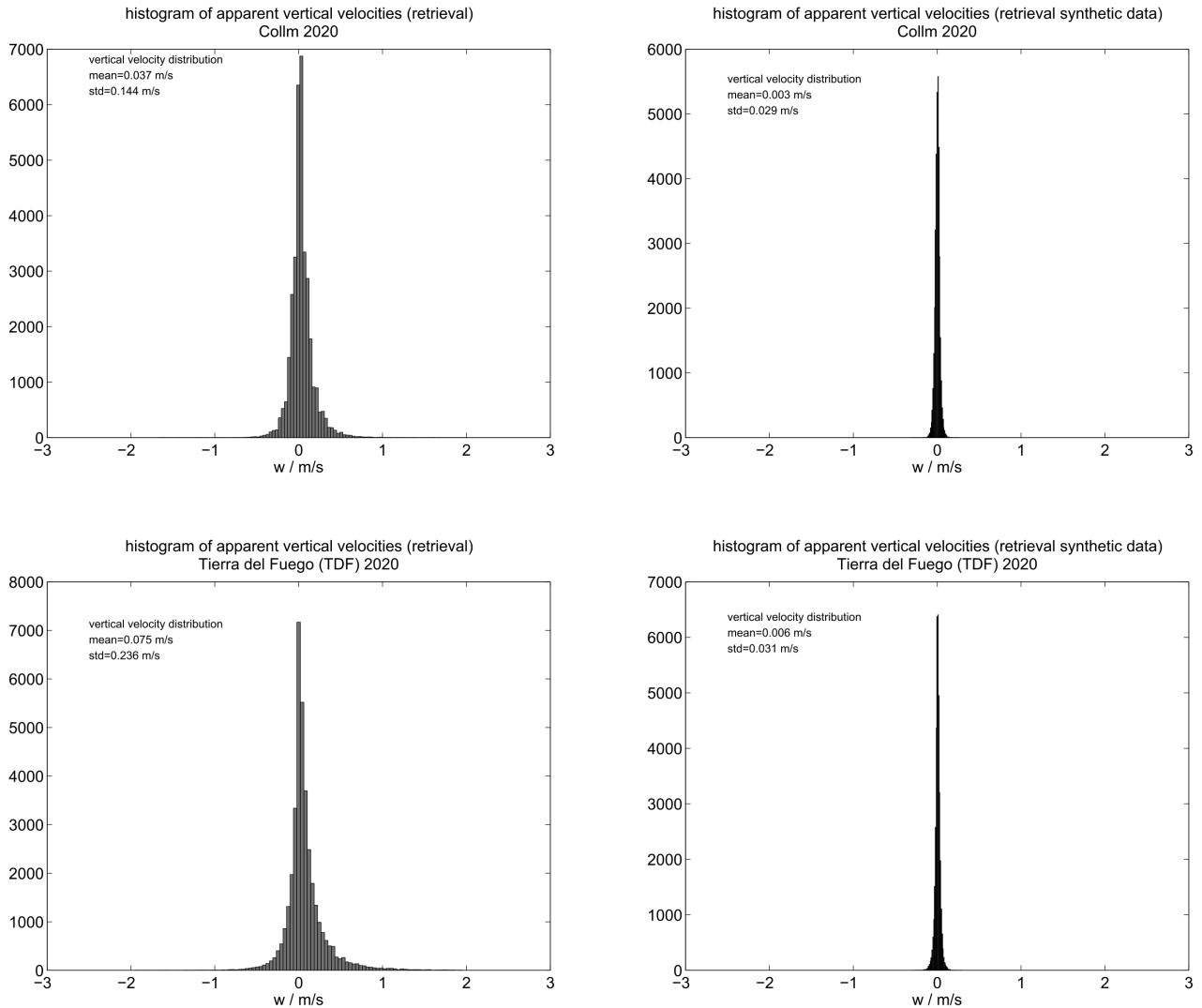
Figure 5. The same as Figure 1, but the hourly vertical winds are obtained by applying the retrieval algorithm including the spatio-temporal Laplace algorithm. The x-axis scale or w -axis scale was reduced to show the remaining variability.
