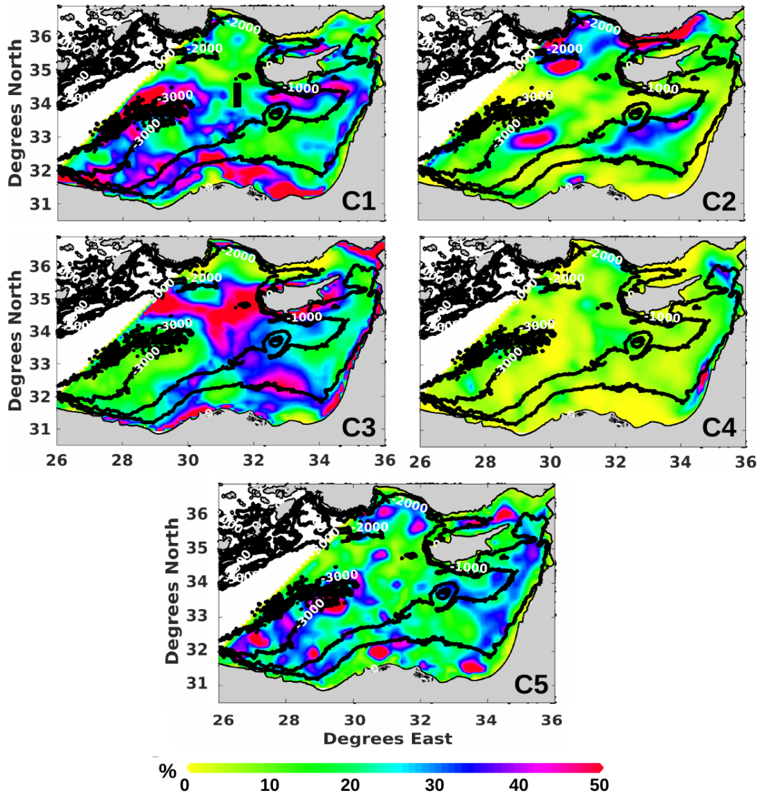
Figure 7. Percentage of C1, C2, C3, C4, and C5 occurrence between 1993 and 2018, overlayed on the main bathymetric iso-lines of -1000, -2000, and -3000 m . The dark line in the C1 subplot shows the position of the Hovmoller diagram in sec. 3.3.
