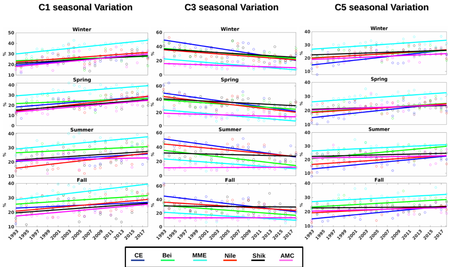
Figure 6. The seasonal variation of the C1 (high kinetic energy), C5 (high vorticity), and C3 (low KE and low vorticity) average in each box and their resulting linear regression.
