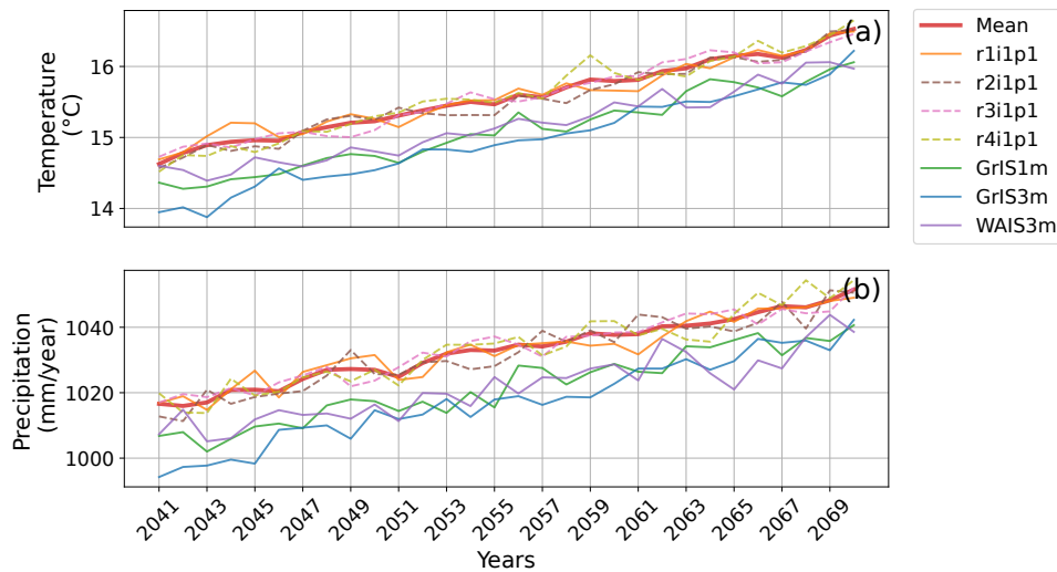
Figure A2. Temporal evolution of a) temperature and b) precipitation over the future period for the different RCP8.5 runs (r1i1p1, r2i1p1, r3i1p1, r4i1p1) and for the different ice melt simulations (GrIS1m, GrIS3m, WAIS3m). The solid orange line depicts the simulation used in the study. The thick red line shows the ensemble mean of all RCP8.5 simulations from r1i1p1 to r4i1p1
