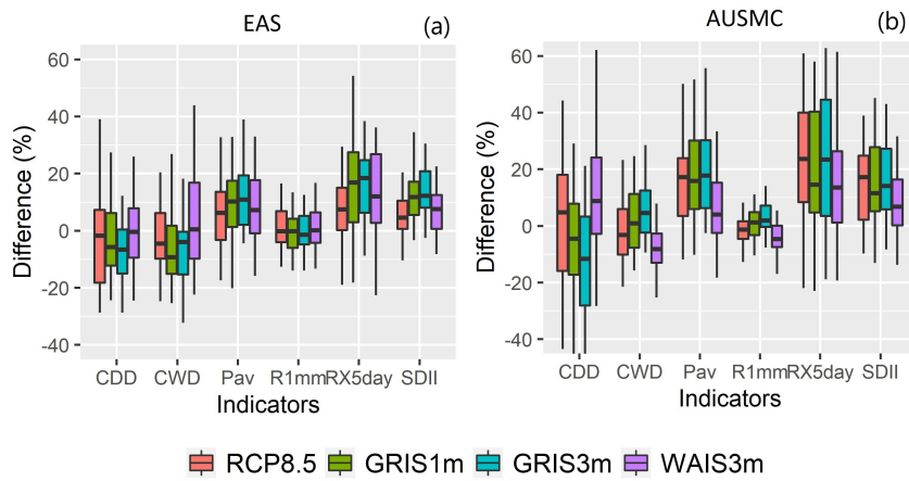
Figure C3. Comparison of the interannual variability of each monsoon index for the period 2041-2070 with the average of the historical period (1976-2005) for each monsoon system a) EAS, b) AUSMC.
