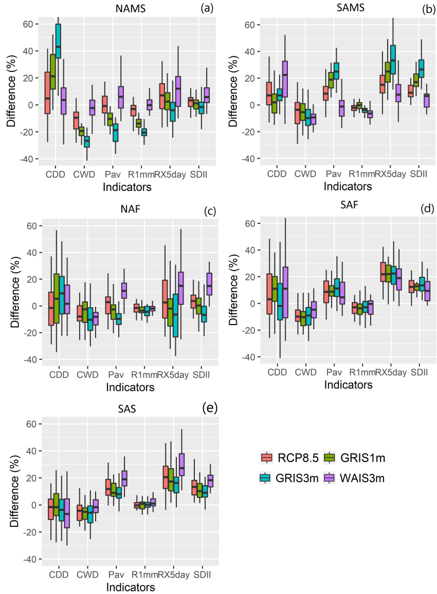
Figure 10. Comparison of the interannual variability of each land monsoon index for the period 2041-2070 with the average of the historical period (1976-2005) for a) NAMS, b) SAMS, c) NAF, d) SAF, e) SAS and for each simulation. RCP8.5 is shown in red, GrIS1m in green, GrIS3m in blue and WAIS3m in purple.
