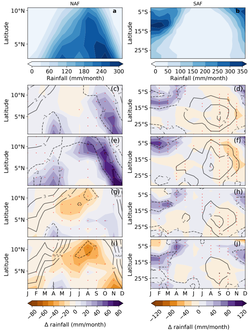
Figure 8. Hovmöller Diagrams the African continent domains. The left column corresponds to the NAF domain (a,c,e,g,i) and the right column to the SAF domain (b,d,f,h,j). a,b) correspond to the precipitation values in \text{mm month}^{-1} over the historical period (1976-2005). All other diagrams correspond to the precipitation difference (colors) and the MSE difference (black contours, dashed lines for negative values) between the future scenario (2041-2070) with c,d) RCP8.5, e,f) WAIS3m, g,h) GrIS1m and i,j) GrIS3m and the historical period (1976-2005), in \text{mm month}^{-1} . Please note that the colour bar values do not correspond to the same values from one column to another. Significant differences at the 95 % confidence interval are depicted by red dots according to the Wilcoxon-Mann-Whitney test (see Sect. 2.3).
