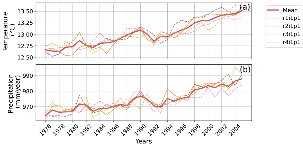
Figure A1. Temporal evolution of a) temperature and b) precipitation over the historical period for the different ensemble members. The solid orange line depicts the simulation used in the study. The thick red line shows the ensemble mean of all simulations from r1i1p1 to r4i1p1
