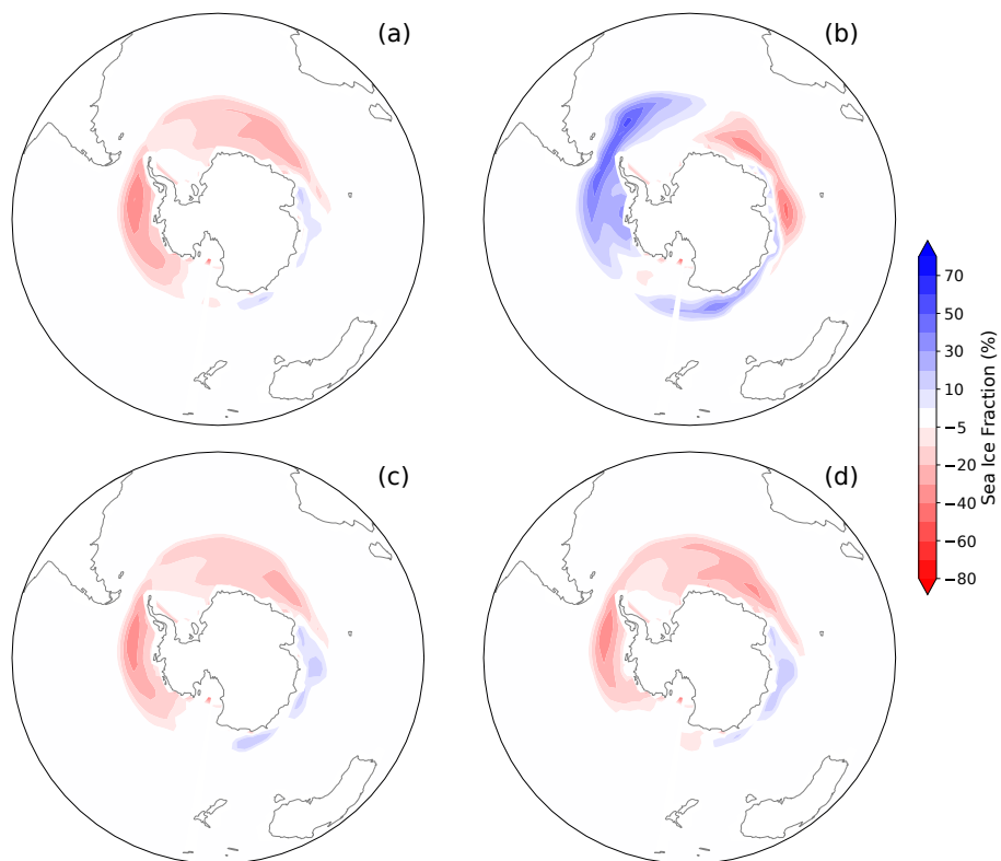
Figure B4. Sea ice fraction difference (%) between future scenario (2041-2070) a) RCP8.5 b) WAIS3m c) GrIS1m d) GrIS3m and historical simulation (1976-2005) for Southern Hemisphere in MJJAS.
