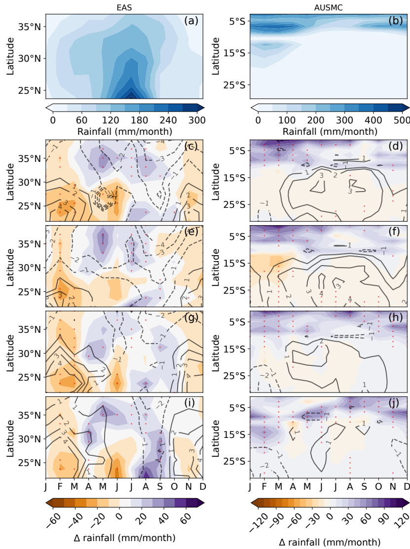
Figure C1. Hovmöller Diagrams. The left column corresponds to the EAS domain (a,c,e,g,i) and the right column to the AUSMC domain (b,d,f,h,j). a,b) correspond to the precipitation values in \text{mm month}^{-1} over the historical period (1976-2005). All other diagrams correspond to the precipitation difference (colors) and the MSE difference (black contours, dashed lines for negative values) between the future scenario (2041-2070) with c,d) RCP8.5, e,f) WAIS3m, g,h) GrIS1m and i,j) GrIS3m and the historical period (1976-2005). Significant differences at the 95 % confidence interval are depicted by red dots according to the Wilcoxon-Mann-Whitney test (see 2.3).
