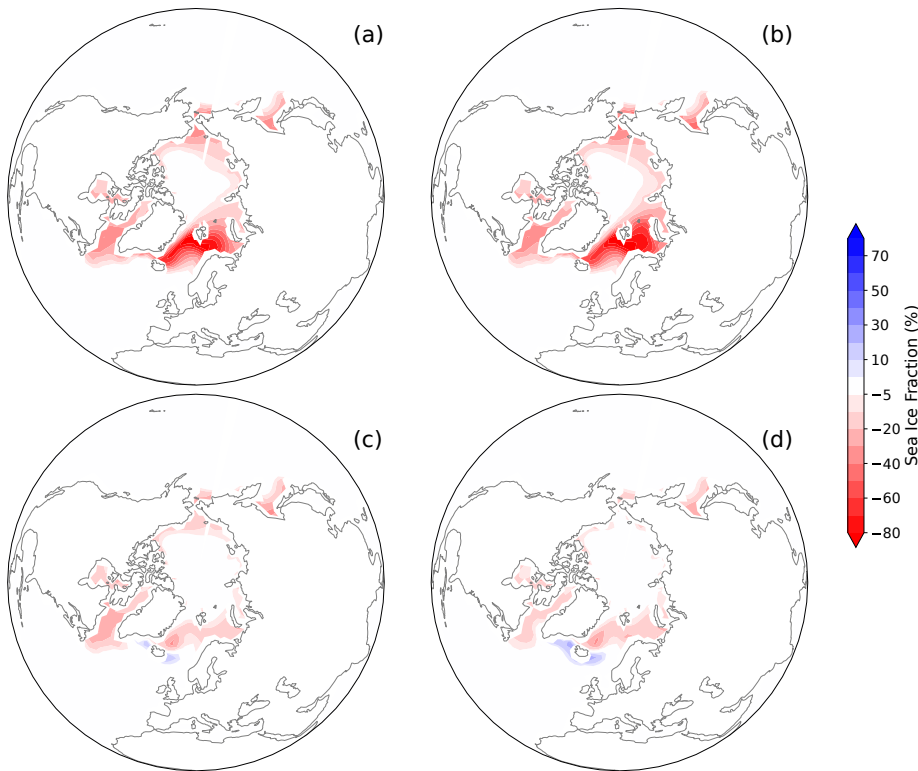
Figure B3. Sea ice fraction difference (%) between future scenario (2041-2070) a) RCP8.5 b) WAIS3m c) GrIS1m d) GrIS3m and historical simulation (1976-2005) for Northern Hemisphere in NDJFM.
