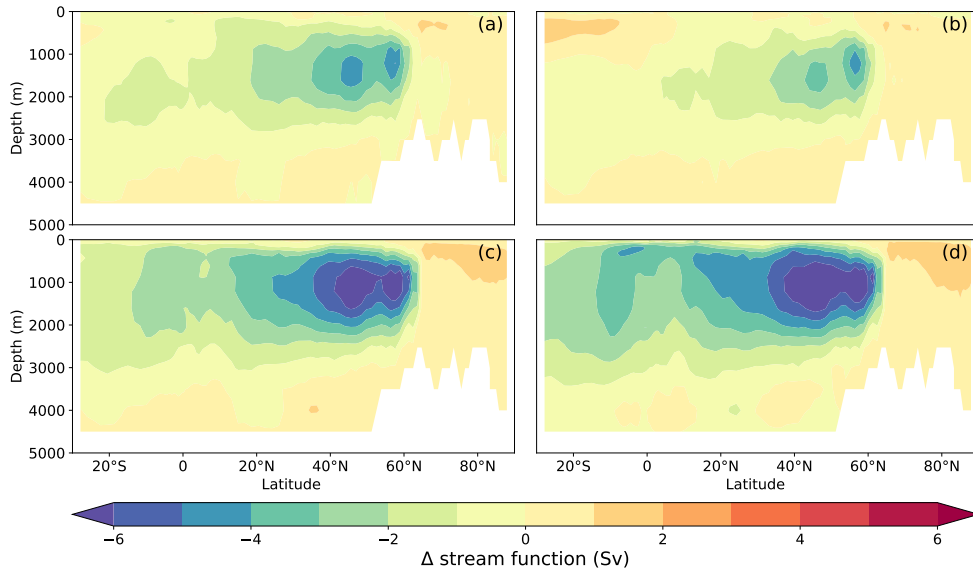
Figure B1. Stream function difference between future scenarios (2041-2070) and historical simulation (1976-2005) for MJJAS season. The future scenarios are a) RCP8.5, b) WAIS3m, c) GrIS1m and d) GrIS3m.
