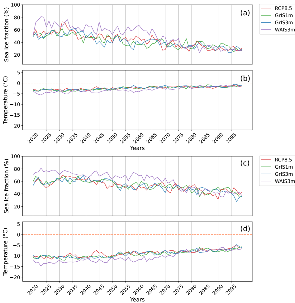
Figure B6. Temporal evolution of a-c) sea ice fraction (%) and b-d) temperature (°C) in the Southern Hemisphere for a-b) NDJFM and c-d) MJJAS. The orange dotted line represents the 0°C isotherm.
