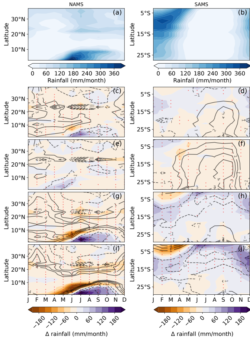
Figure 7. Hovmöller Diagram Diagrams for the domains-of-the domains of the American continent. The left column corresponds to the NAMS domain (a,c,e,g,i) and the right column to the SAMS domain (b,d,f,h,j). a-b correspond to the precipitation values in \text{mm month}^{-1} over the historical period (1976-2005). All other diagrams correspond to the precipitation difference (colors) and the \Delta MSE anomaly (black contours, dashed lines for negative values) between the future scenario (2041-2070) with e,d-c-d RCP8.5, e,f-e-f WAIS3m, g,h-g-h GrIS1m and i,j-i-j GrIS3m and the historical period (1976-2005), in \text{mm month}^{-1} . Significant differences at the 95 % confidence interval are depicted by red dots according to the Wilcoxon-Mann-Whitney test (see Sect. 2.3).
