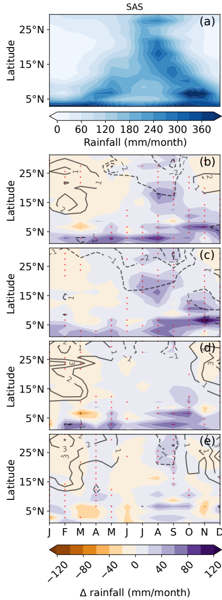
Figure 9. Hovmöller Diagram Diagrams for the domains-of-the SAS domain. a) correspond to the precipitation values in \text{mm month}^{-1} over the historical period (1976-2005). All other diagrams correspond to the precipitation difference (colors) and the \Delta MSE anomaly (black contours, dashed lines for negative values) between the future scenario (2041-2070) with b) RCP8.5, c) WAIS3m, d) GrIS1m and e) GrIS3m and the historical period (1976-2005), in \text{mm month}^{-1} . Significant differences at the 95 % confidence interval are depicted by red dots according to the Wilcoxon-Mann-Whitney test (see Sect. 2.3).
