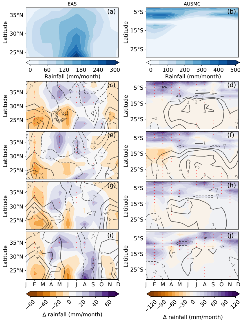
Figure C1. Hovmöller Diagram Diagrams . The left column corresponds to the EAS domain (a,c,e,g,i) and the right column to the AUSMC domain (b,d,f,h,j). a-b correspond to the precipitation values in \text{mm month}^{-1} over the historical period (1976-2005). All other diagrams correspond to the precipitation difference (colors) and the \Delta MSE anomaly (black contours, dashed lines for negative values) between the future scenario (2041-2070) with e,d - d ) RCP8.5, e,f - f ) WAIS3m, g,h - h ) GrIS1m and i,j - j ) GrIS3m and the historical period (1976-2005). Significant differences at the 95 % confidence interval are depicted by red dots according to the Wilcoxon-Mann-Whitney test (see Sect. 2.3 ).
