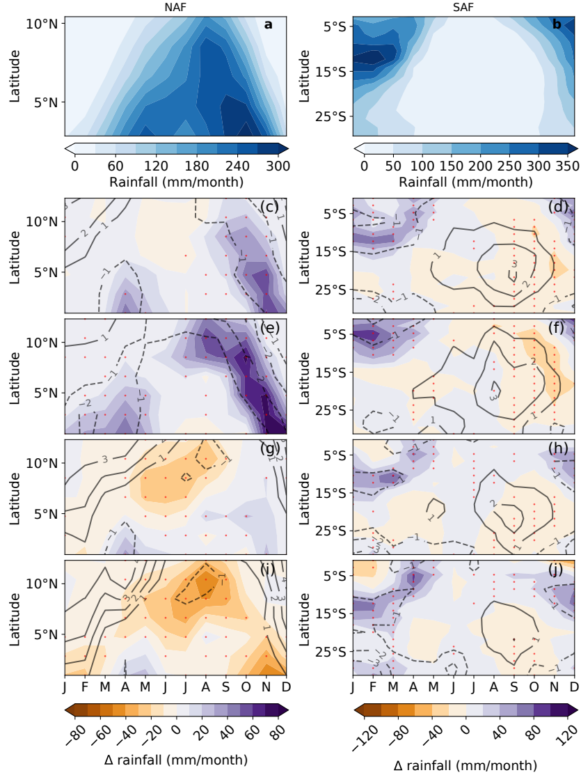
Figure 8. Hovmöller Diagram-Diagrams for the domains-of-the-African continent domains . The left column corresponds to the NAF domain (a,c,e,g,i) and the right column to the SAF domain (b,d,f,h,j). a-ba-b ) correspond to the precipitation values in \text{mm month}^{-1} over the historical period (1976-2005). All other diagrams correspond to the precipitation difference (colors) and the \Delta MSE anomaly (black contours, dashed lines for negative values) between the future scenario (2041-2070) with e,d-c-d RCP8.5, e,fe-f WAIS3m, g,hg-h GrIS1m and i,ji-j GrIS3m and the historical period (1976-2005), in \text{mm month}^{-1} . Please note that the colour bar values do not correspond to the same values from one column to another. Significant differences at the 95 % confidence interval are depicted by red dots according to the Wilcoxon-Mann-Whitney test (see Sect. 2.3).
