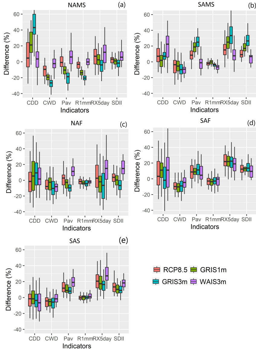
Figure 10. Comparison of the interannual variability of each land monsoon index for the future period (2041-2070) with the average of the historical period (1976-2005) for each monsoon system a) NAMS, b) SAMS, c) NAF, d) SAF, e) SAS and for each simulation. RCP8.5 is shown in red, GRIS1m in green, GRIS3m in blue and WAIS3m in purple.
