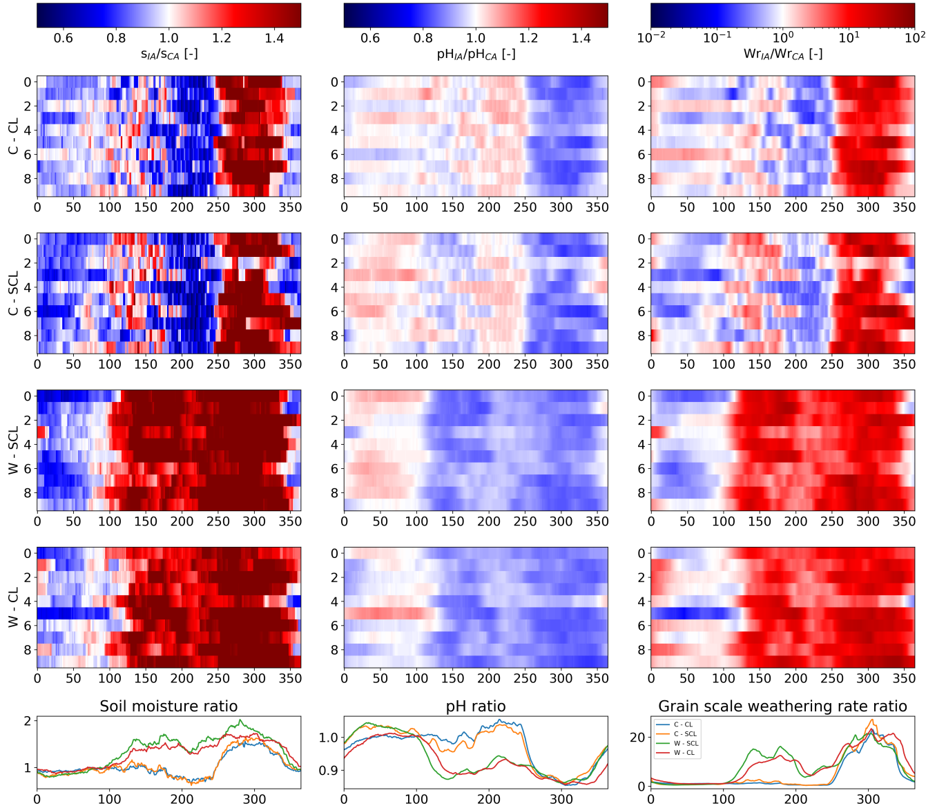
Figure 6. Time-series heatmaps of the ratio between soil moisture ( s ), pH and weathering rate ( Wr ) achieved in the case of Iowa (IA) and those related to California (CA) computed within 10 years after olivine addition. These are related to corn planted in a clay loam soil (C - CL, panels in the first row of the figure), corn planted in a silty clay loam soil (C - SCL, panels in the second row of the figure), wheat planted in a silty clay loam soil (W - SCL, panels in the third row of the figure) and wheat planted in a clay loam soil (W - CL, panels in the fourth row of the figure). The average daily ratios of the three considered variables are shown in the last panel of the figure.
