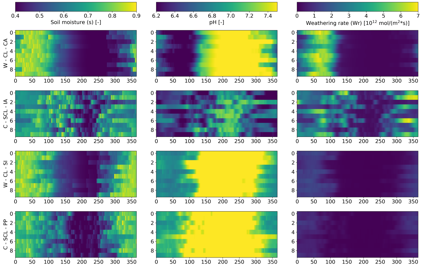
Figure 11. Time-series heatmaps of soil moisture ( s ), pH and weathering rate ( Wr ) computed within 10 years after olivine addition. These are related to wheat planted in clay loam soil for California ( W - CL - CA , panels in the first row of the figure), and corn in silty clay loam soil for Iowa ( C - SCL - IA , panels in the second row of the figure), wheat in clay loam soil for Sicily (W - CL - SI, panels in the third row of the figure) and corn in silty clay loam soil for the Padan plain (C - SCL - PP, panels in the last row of the figure).
