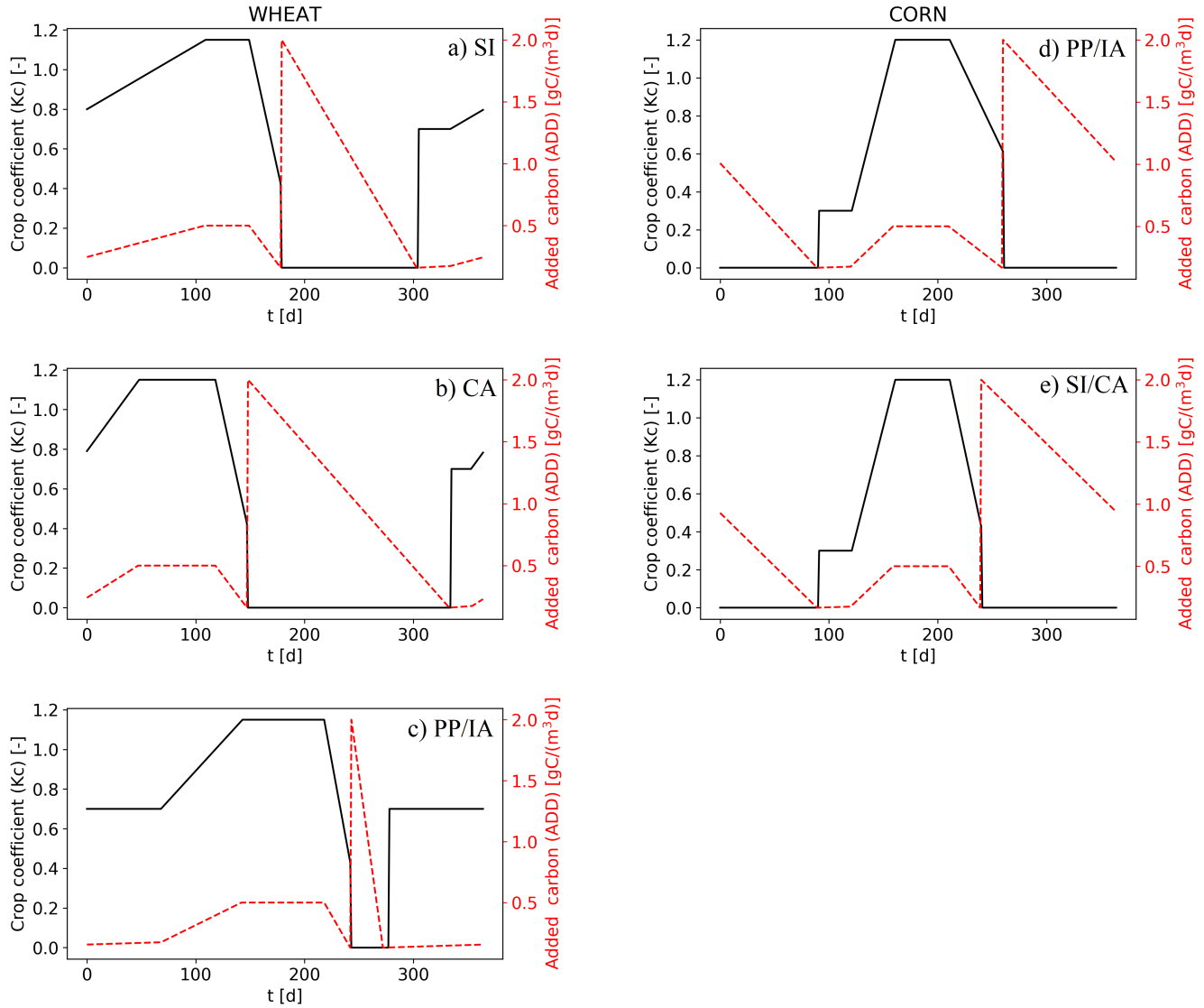
Figure 5. Seasonal variability of the crop coefficient ( Kc ) and the added carbon from vegetation ( ADD ) for a) wheat in Sicily, b) wheat in California, c) wheat in the Padan plain and Iowa, d) corn in Padan plain and Iowa and e) corn in Sicily and California. The reader is referred to Section 2.2.3 for more details.
