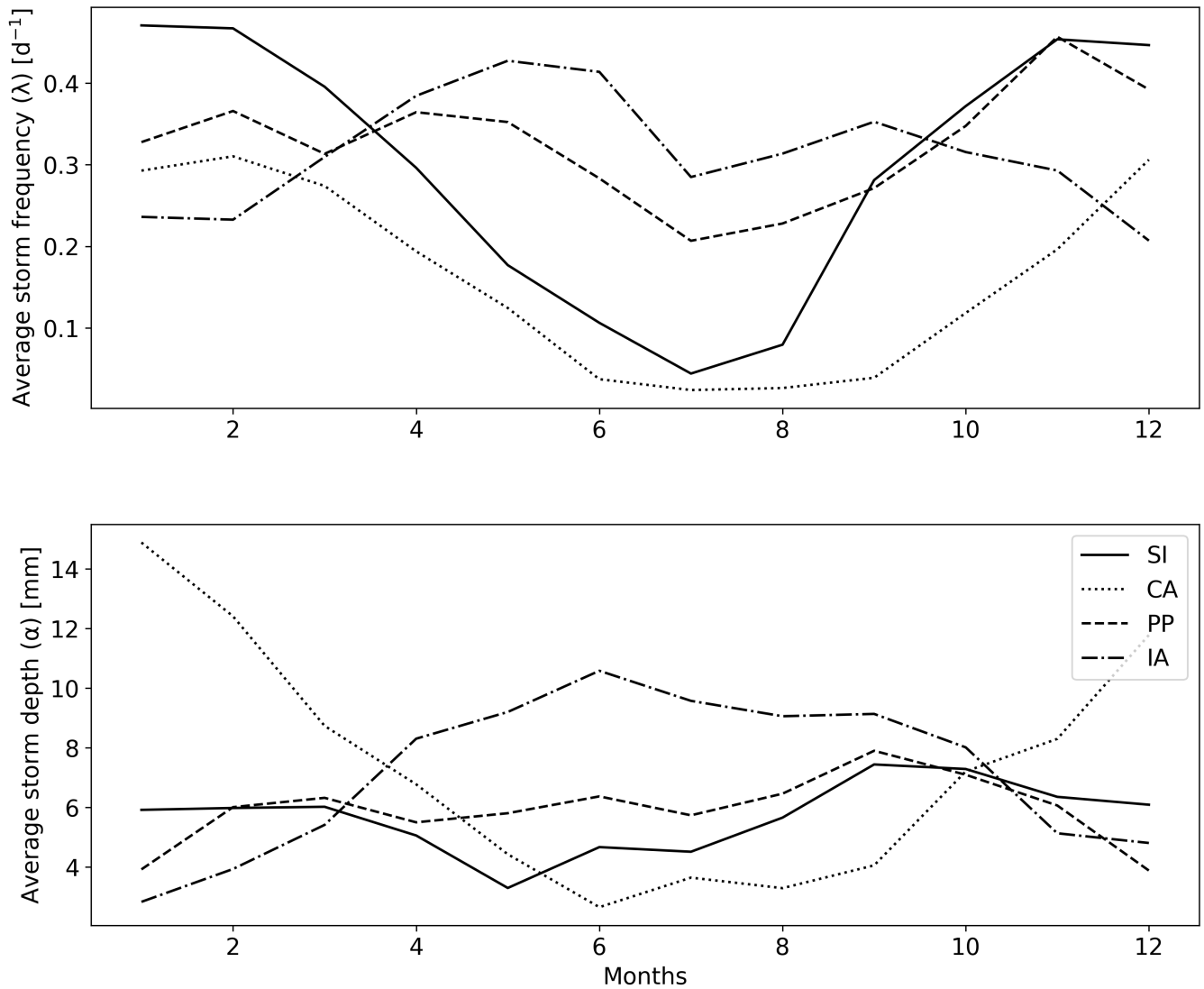
Figure 3. Values of the average rainfall depth ( \alpha ) and frequency ( \lambda ) rainfall parameters from January (i.e., month indicated with 1) to December (i.e., month indicated with 12). The reader is referred to Section 2.2.1 for more details for a) Sicily, b) California, c) Padan plain and d) Iowa.
