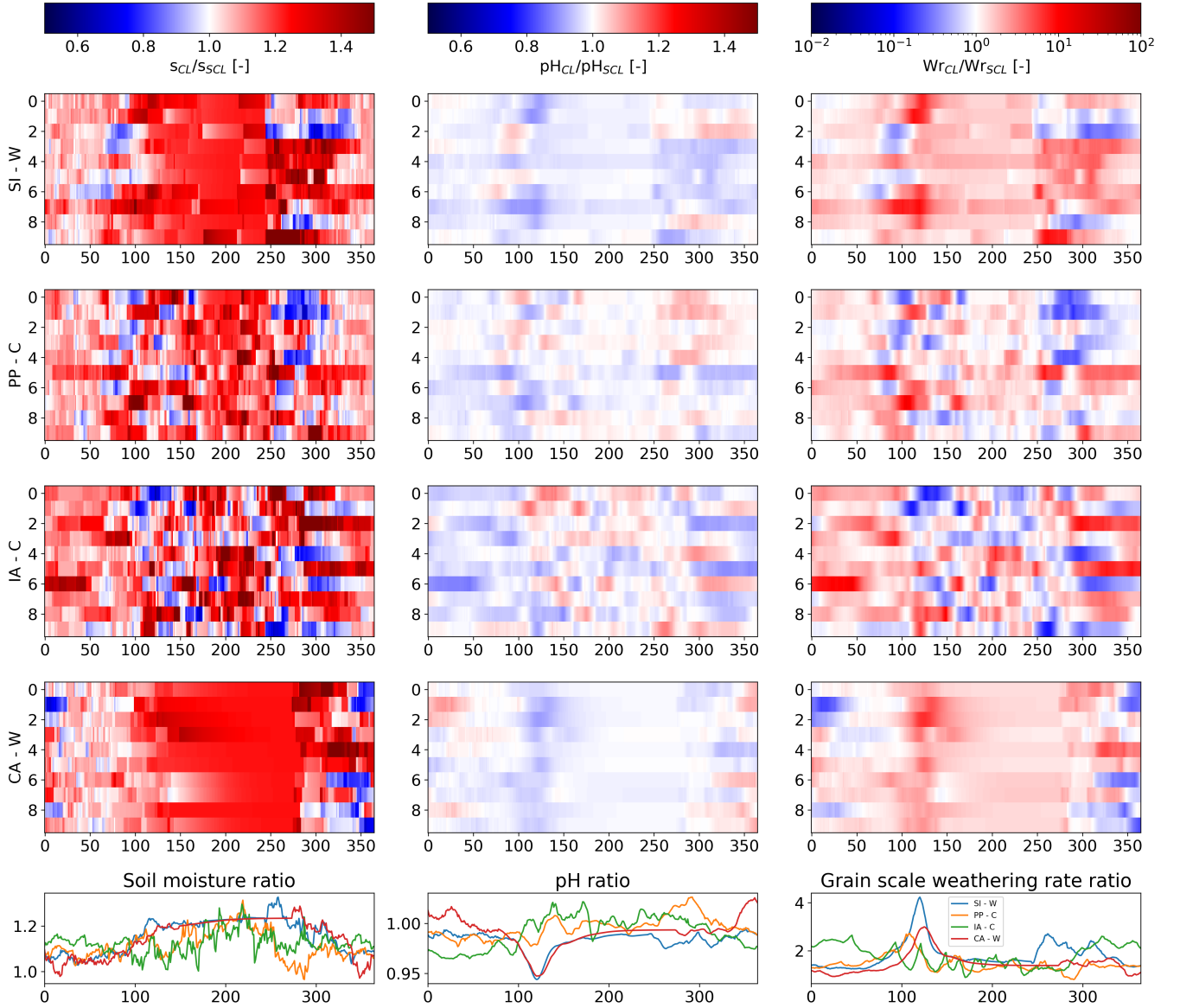
Figure 8. Time-series heatmaps of the ratio between soil moisture ( s ), pH and weathering rate ( Wr ) achieved considering the clay loam soil ( CL ) and those related to the silty clay loam soil ( SCL ). The heatmaps are related to a period of 10 years after olivine addition. These are related to Sicily with wheat ( SI - W , panels in the first row of the figure), Padan plain with corn ( PP - C , panels in the second row of the figure), Iowa with corn ( IA - C , panels in the third row of the figure) and California with wheat ( CA - W , panels in the fourth row of the figure). The average daily ratios of the three considered variables are shown in the last panel of the figure.
