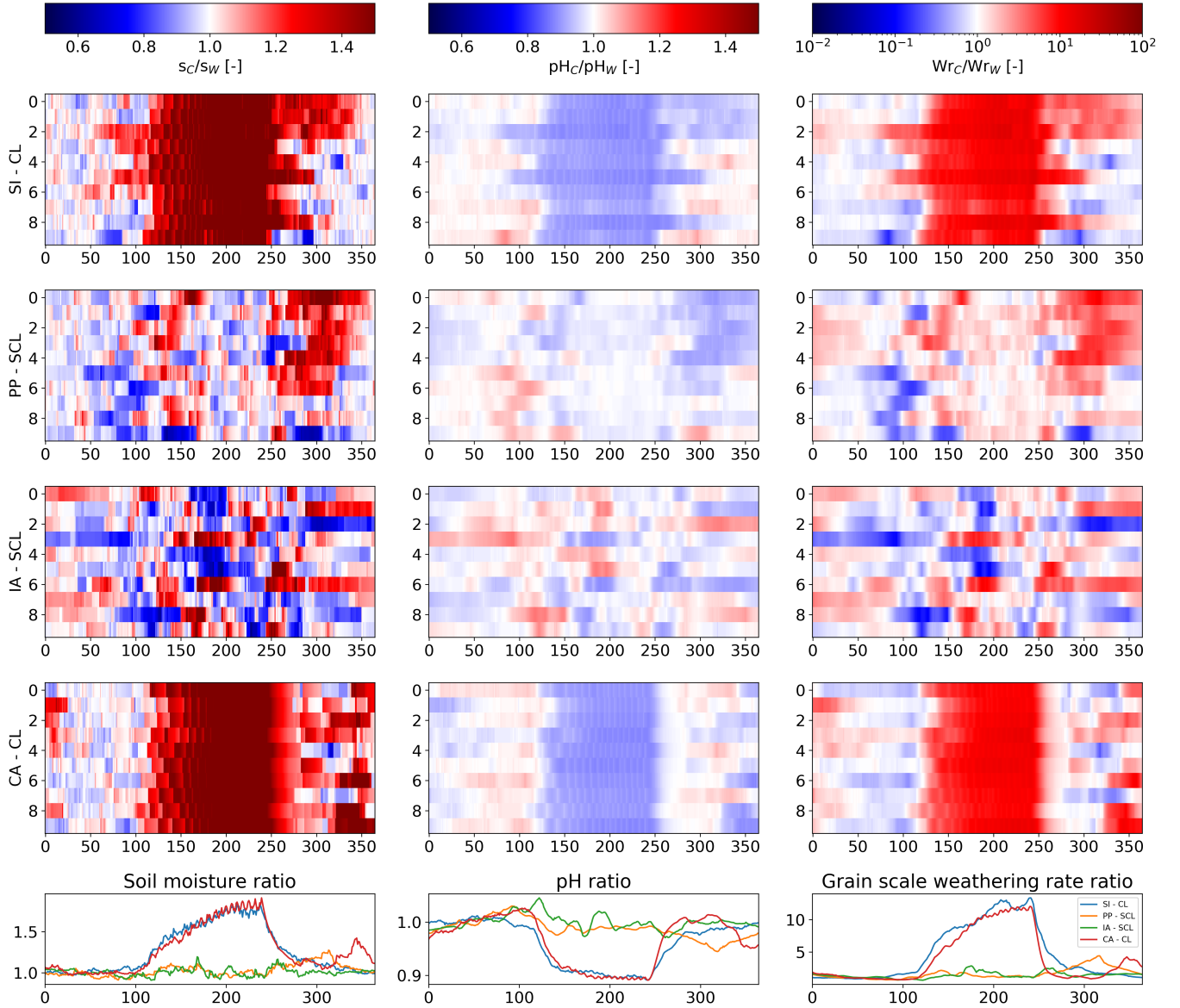
Figure 9. Time-series heatmaps of the ratio between soil moisture ( s ), pH and weathering rate ( Wr ) achieved considering the corn ( C ) and those related to wheat ( W ). The heatmaps are related to a period of 10 years after olivine addition. These are related to Sicily with clay loam ( SI - CL , panels in the first row of the figure), Padan plain with silty clay loam ( PP - SCL , panels in the second row of the figure), Iowa with silty clay loam ( IA - SCL , panels in the third row of the figure) and California with clay loam soil ( CA - CL , panels in the fourth row of the figure). The average daily ratios of the three considered variables are shown in the last panel of the figure.
