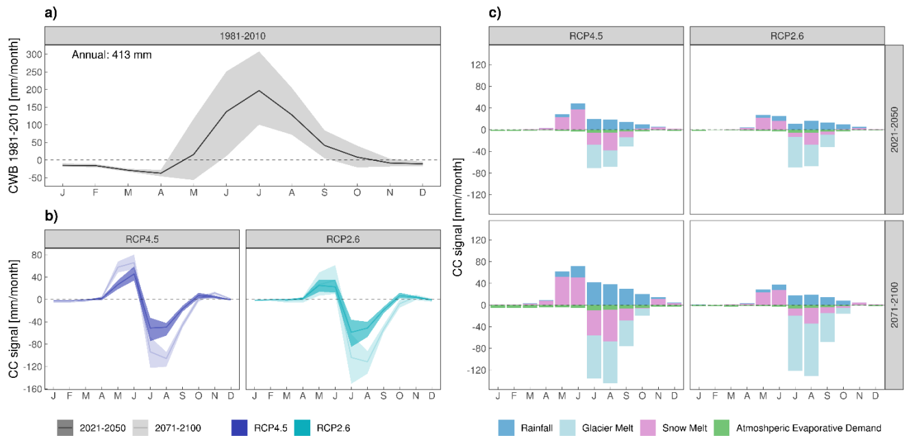
420 Figure 6: Monthly climate change signal of the CWB for the high alpine areas; (a) observed average monthly CWB in the reference period 1981-2010, where the shading denotes for the spatial variability of the CWB climatology, (b) ensemble median monthly climate change signal of the CWB for RCP4.5 (blue) and RCP2.6 (turquoise) for the near future in bold colour and the far future in pale colour, the shading denotes for the ensemble spread given by the 10th and 90th, (c) ensemble median monthly climate change signal of the individual CWB terms; rainfall: blue, snow melt: magenta, AED: green.
