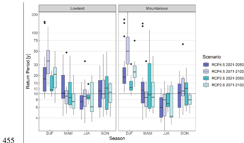
Figure 7: Change in return period of a CWB 10-year event in the reference period (1981-2010) for lowlands (left) and mountainous areas (right) under RCP4.5 (blue) and RCP 2.6 (turquoise) for the near future (2021-2050, bold colours) and the far future (2071-2100, pale colours), the boxplot denote for the ensemble spread of the individual climate model runs.
