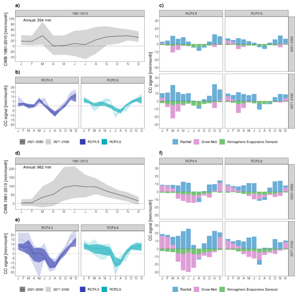
330 Figure 4: Monthly climate change signal of the CWB for lowlands in the upper panel and mountainous areas in the lower panel; (a,d) observed average monthly CWB in the reference period 1981-2010, where the shading denotes for the spatial variability of the CWB climatology, (b, e) ensemble median monthly climate change signal of the CWB for RCP4.5 (blue) and RCP2.6 (turquoise) for the near future in bold colour and the far future in pale colour, the shading denotes for the ensemble spread given by the 10th and 90th. (c, f) ensemble median monthly climate change signal of the individual CWB terms; rainfall: blue, snow melt: magenta, AED: green. Monthly climate change signal of the CWB for lowlands (upper panel, a-c) and mountainous areas (lower panel, d-f); (a, d) observed average monthly CWB in the reference period 1981-2010 (shading denotes for the spatial variability of the CWB
