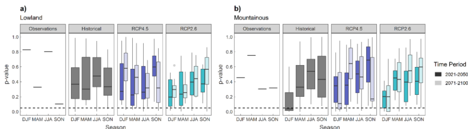
Figure 2: p-values of the Shapiro-Wilk test for normality considering seasonal CWB values for a) lowland and b) mountainous areas for observations (based on SPARTACUS and ARET data) shown as short segments and the historical runs of the selected RCMs as well as for scenarios RCP4.5 and RCP2.6 for the near future (2021-2050) and the far future (2071-2100) displayed as boxplots denoting for the distribution among the different model realizations.
