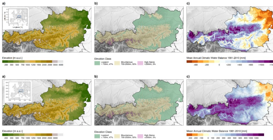
Figure 1: (a) Topography of Austria, (b) altitudinal classification, (c) long term mean (1981-2010) annual climatic water balance
