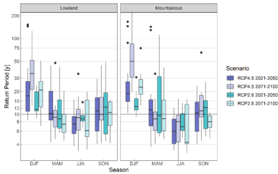
480 Figure 7: Change in return period of a CWB 10-year event in the reference period (1981-2010) for lowlands (left) and mountainous areas (right) under RCP4.5 (blue) and RCP 2.6 (turquoise) for the near future (2021-2050, bold colours) and the far future (2071-2100, pale colours), the boxplot denote for the ensemble spread of the individual climate model runs.
