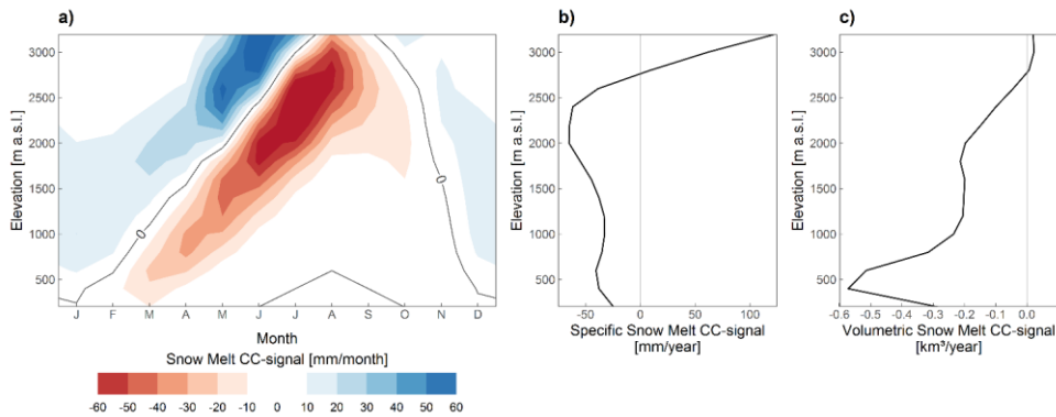
400 Figure 5: (a) Snow melt CC signal depending on time of the year (month) and elevation for RCP4.5, 2071-2100, (b) averaged over all months (c) given as volumetric change (multiplied by area of elevation class).
