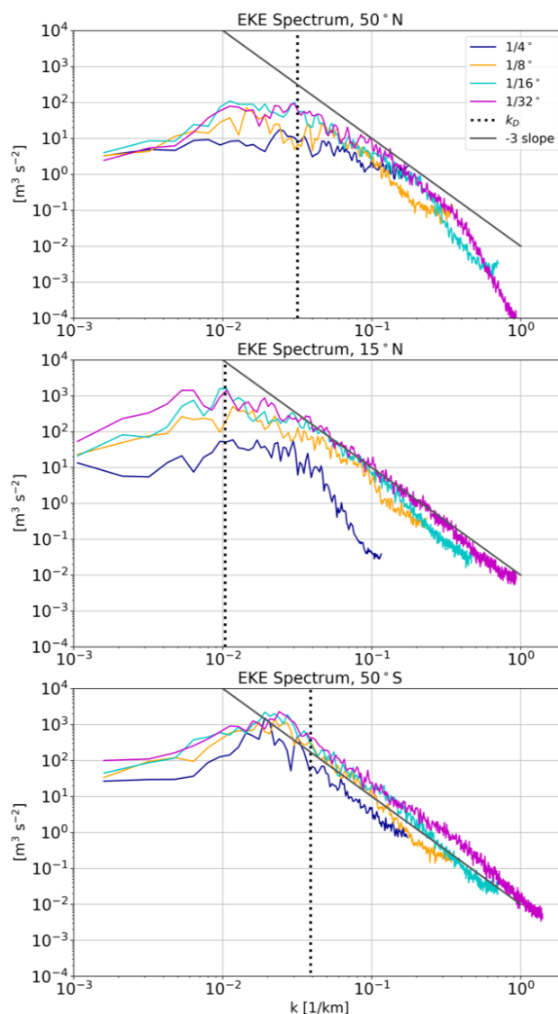
Figure 13. 100-day averaged spectra of surface EKE for all resolutions at three latitudes (top to bottom): 50^{\circ}N (weak mean flow region), 15^{\circ}N (mid-latitude gyre), and 50^{\circ}S (ACC). Spectra are computed from the surface meridional eddy velocity fields, defined as deviations from a 100-day averaged meridional velocity (linear detrending and a Hann smoothing window are applied). The wavenumber k_D corresponding to the deformation radius for the 1/32^{\circ} simulation is shown as a dotted black line, and a -3 spectral slope is shown in grey.
