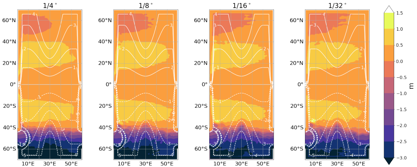
Figure 7. Time-mean sea surface height (SSH, m) averaged over the last 500 days of each simulation. White contours denote f/H ( \times 10^{-8} \text{ m}^{-1} \text{ s}^{-1} ).
