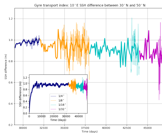
Figure 5. Time series of the gyre transport index, defined here as the difference in sea-surface height (m) at 10^{\circ}E between 50^{\circ}N and 30^{\circ}N for each of the model horizontal grids during spin-up and equilibration. Thin lines are 5-day means (where available), thicker lines are 100-day means.
