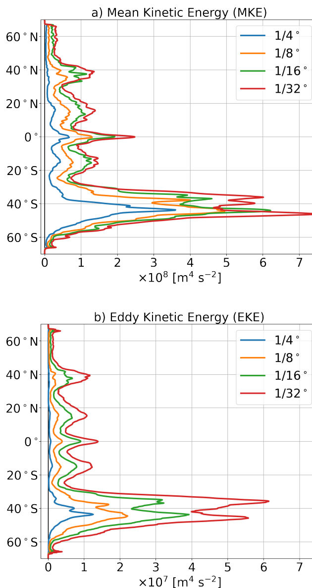
Figure 12. 500-day averaged, zonally- and depth-integrated a) mean kinetic energy (MKE, (8)) and b) eddy kinetic energy (EKE, (9)) for the four simulations in our model hierarchy. To compute MKE and EKE, we used a spatial filter with filter scale 1/4^\circ in all four cases. Note that the x-axis in b) has been stretched by an order of magnitude compared to a).
