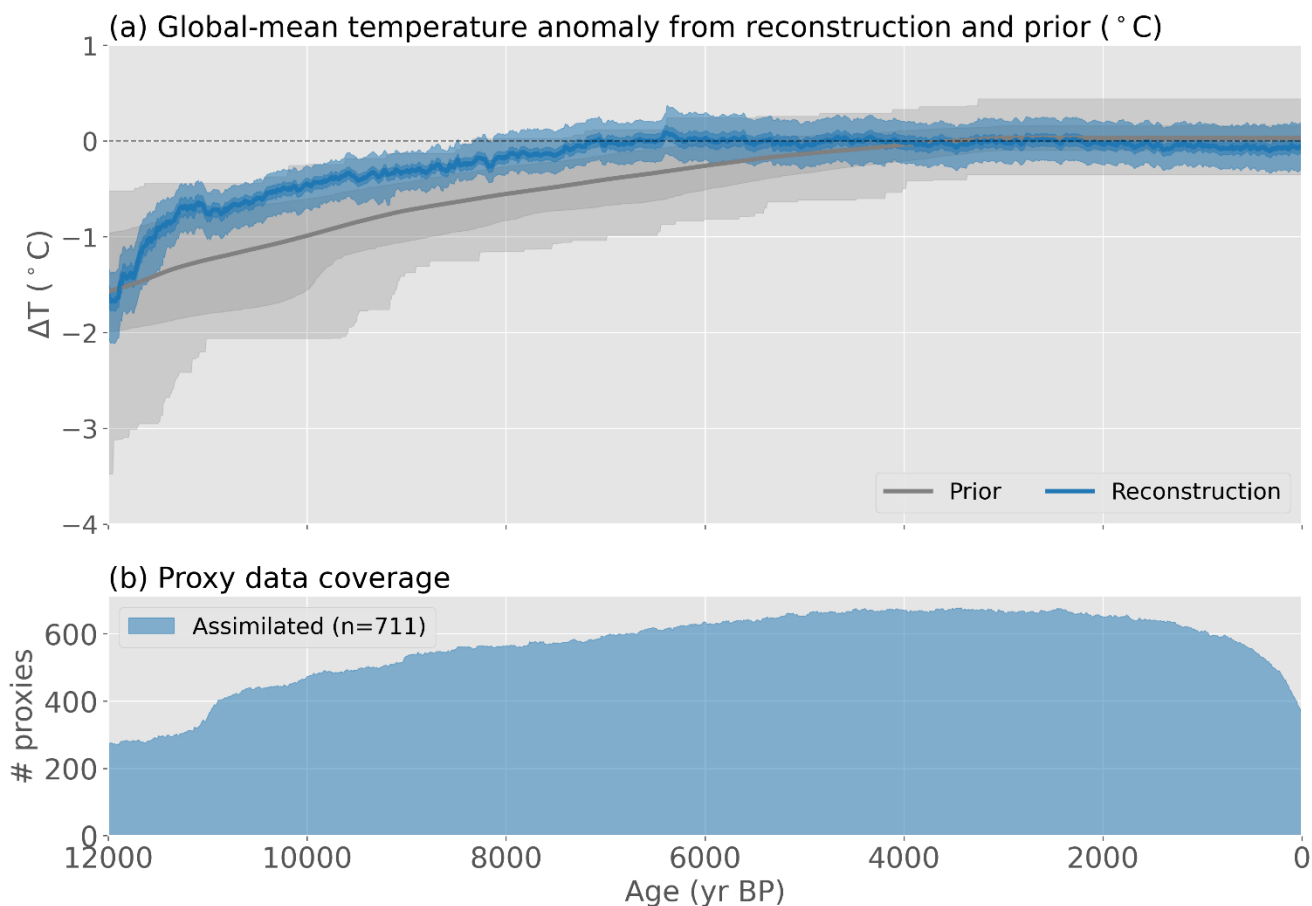
Figure 4. Reconstructed global mean temperature. (a) Global mean temperature in the prior (gray) and reconstruction (blue). Lines show the ensemble mean and colored bands show the 1-sigma and full ranges of the ensemble. The reconstruction uses 3-5 ka as the reference period, as most records overlap with that period. (b) The temporal proxy coverage, showing the number of assimilated observations at each time step.
