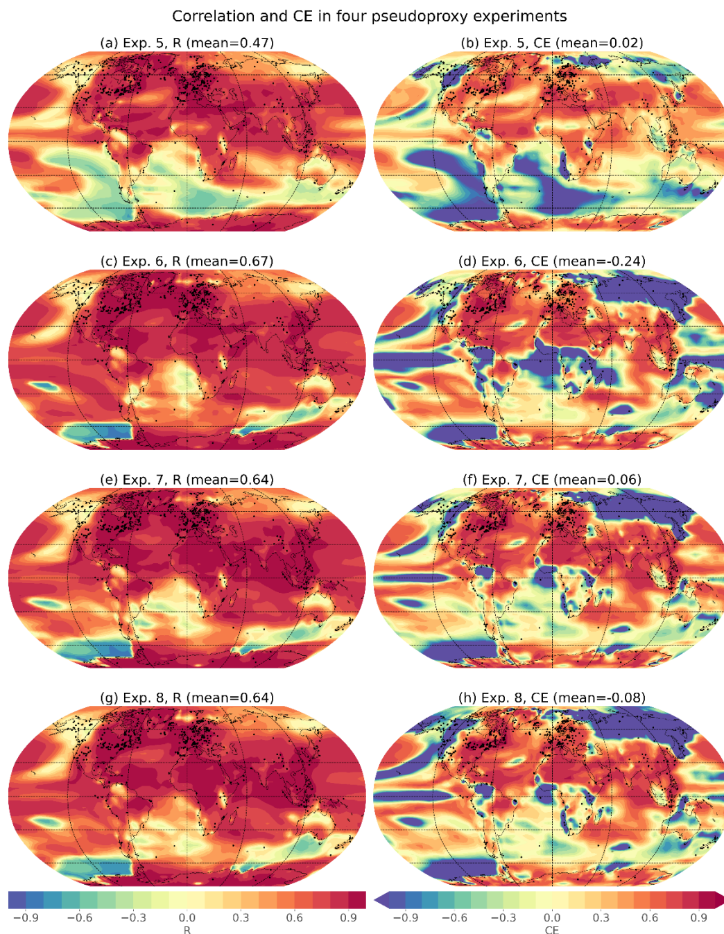
765 Figure B3. Spatial skill of more pseudoproxy experiments. Spatial correlations ( r ) and coefficients of efficiency (CE) for four additional pseudoproxy experiments, as in Fig. A2. Experiments are the same as the default experiment but use a localization radius and/or a time-varying prior. Exp. 5 uses a time-varying prior 5010 years long, as in the main experiment, but with the mean value set to 0 for every period. Exp. 6 uses a time-constant prior consisting of all climate states centered on 0.5 to 12.5 ka. Exp. 7 uses a localization radius of 25,000 km. Exp. 8 uses a time-varying prior of 3010 years, rather than 5010 years in the default experiment. More details about these experiments are given in Table 2.
