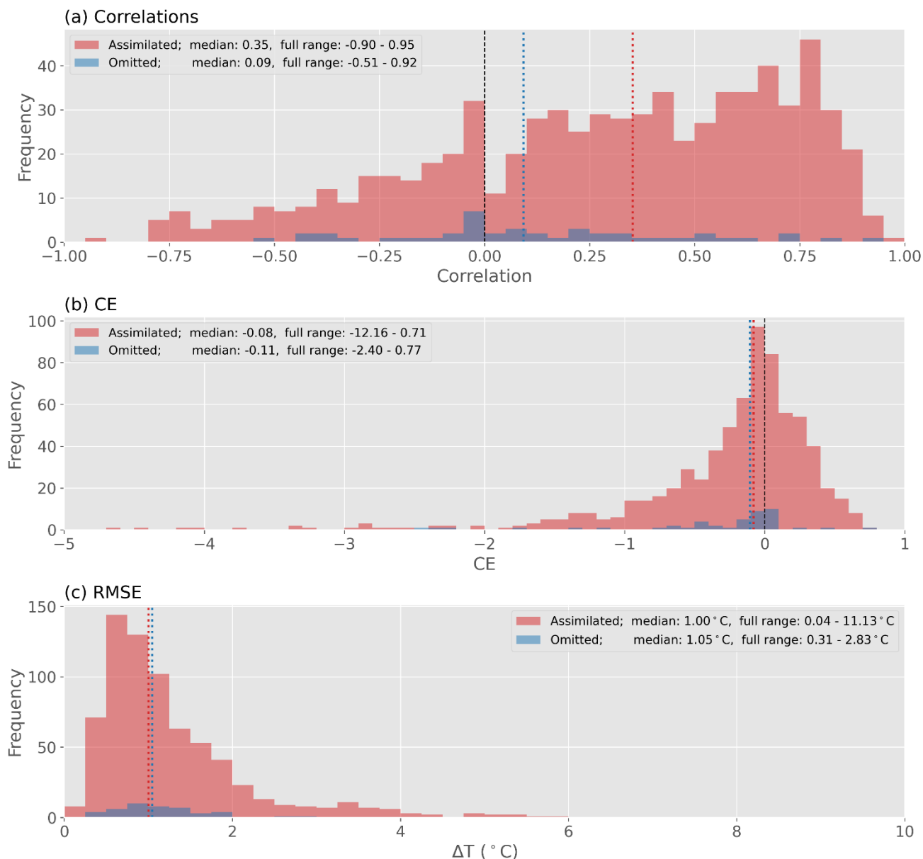
700 Figure A3. Agreement between proxy records and reconstructed proxy values. Distributions of (a) Pearson's correlation coefficient, (b) coefficient of efficiency (CE), and (c) root mean square error for each calibrated proxy compared to reconstructed temperature at the same location and season. Comparisons are made on a decadal timescale. Distributions show assimilated records (red) and records which were omitted due to a lack of uncertainty values ( n=44 , blue). Median values are shown as vertical lines.
