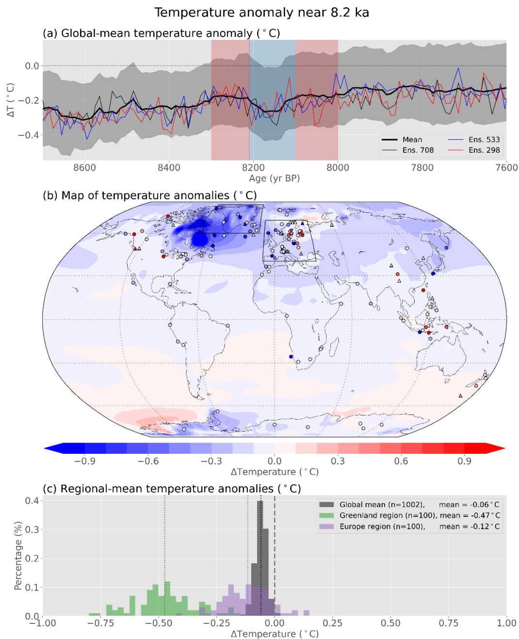
485 Figure 11. Cooling at 8.2 ka. (a) Reconstructed temperature anomalies ( ^{\circ}\text{C} ) for (a) the global mean, (b) spatial patterns for the 8.2 490 ka event in the reconstruction (shading) and proxies (symbols), and (c) global and regional means at the 8.2 ka event calculated across ensemble members. The periods used for the calculations used in (b,c) are shown in (a), with the anomaly period shown in blue and the reference periods shown in red. Proxies are only shown in (b) if they have at least one value in each of the three periods shown in (a), which is 169 of the 711 assimilated proxies. Proxy seasonality is annual (circles), summer (upward-pointing triangles), or winter (downward-pointing triangles). The spatial extent of the Greenland and Europe regions in (c) are shown in (b). In (c), all ensemble members are shown for the global mean while a randomly selected group of 100 ensemble members are shown for the other two regions.
