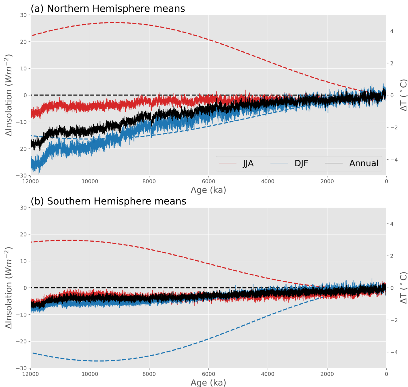
Figure 2. Modeled hemispheric insolation and temperature in different seasons. Insolation ( W m^{-2} , dashed) and temperature ( ^{\circ}C , solid) from the HadCM3 deglacial simulation, averaged for the annual mean (black), June-August (red), and December-February (blue) for the (a) Northern Hemisphere and (b) Southern Hemisphere. Throughout this paper, original monthly data is used from models, with no adjustment to account for the calendar effect (Joussaume and Braconnot, 1997).
