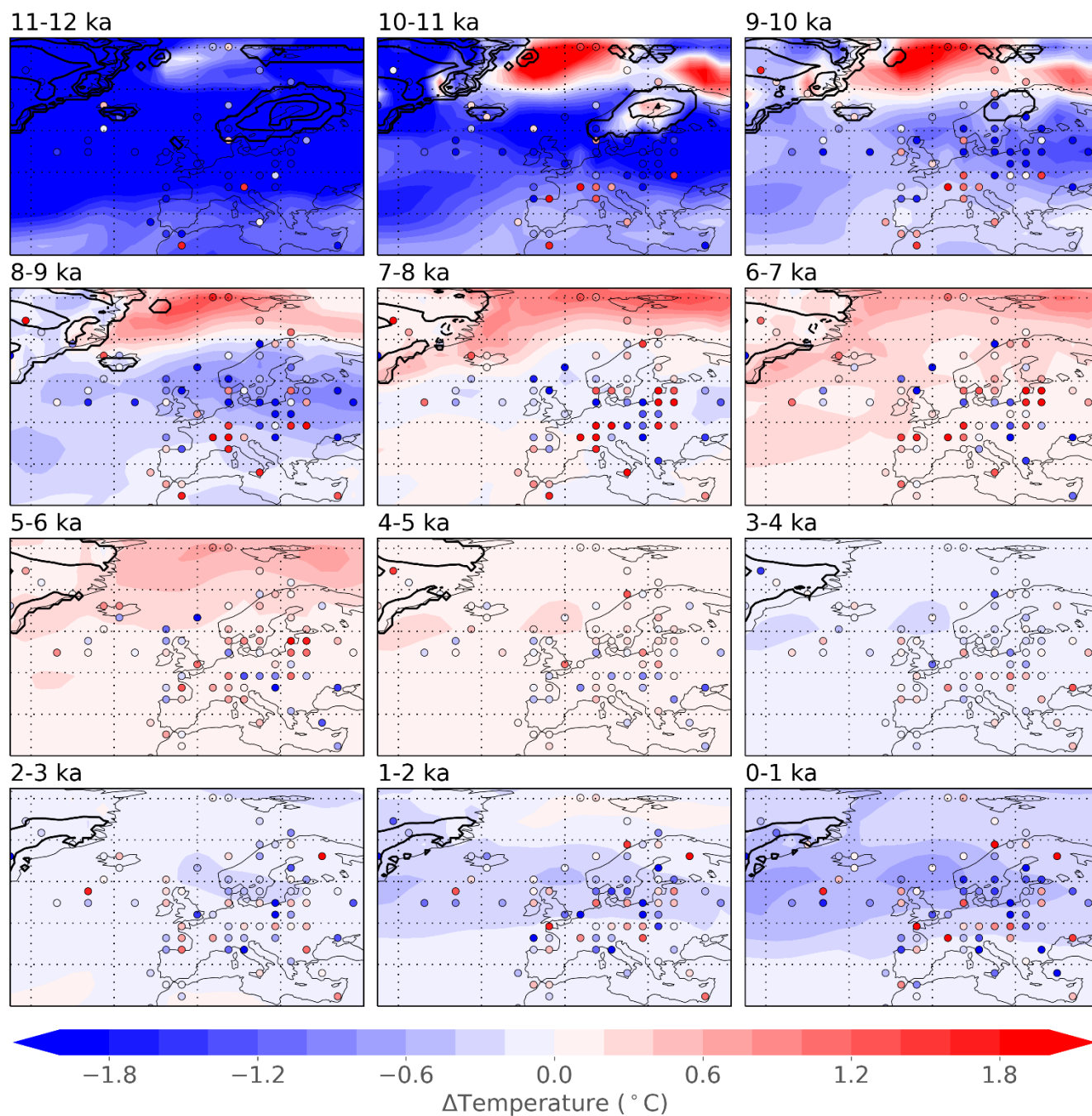
Figure 10. Temperature and ice sheets in Europe. Millennial anomalies for reconstructed temperature (shaded, ^{\circ} C), gridded annual mean proxy records (dots, ^{\circ} C), and ice sheets from the ICE-6G_C reconstruction (contours, 500 m interval), as in Fig. 9.
