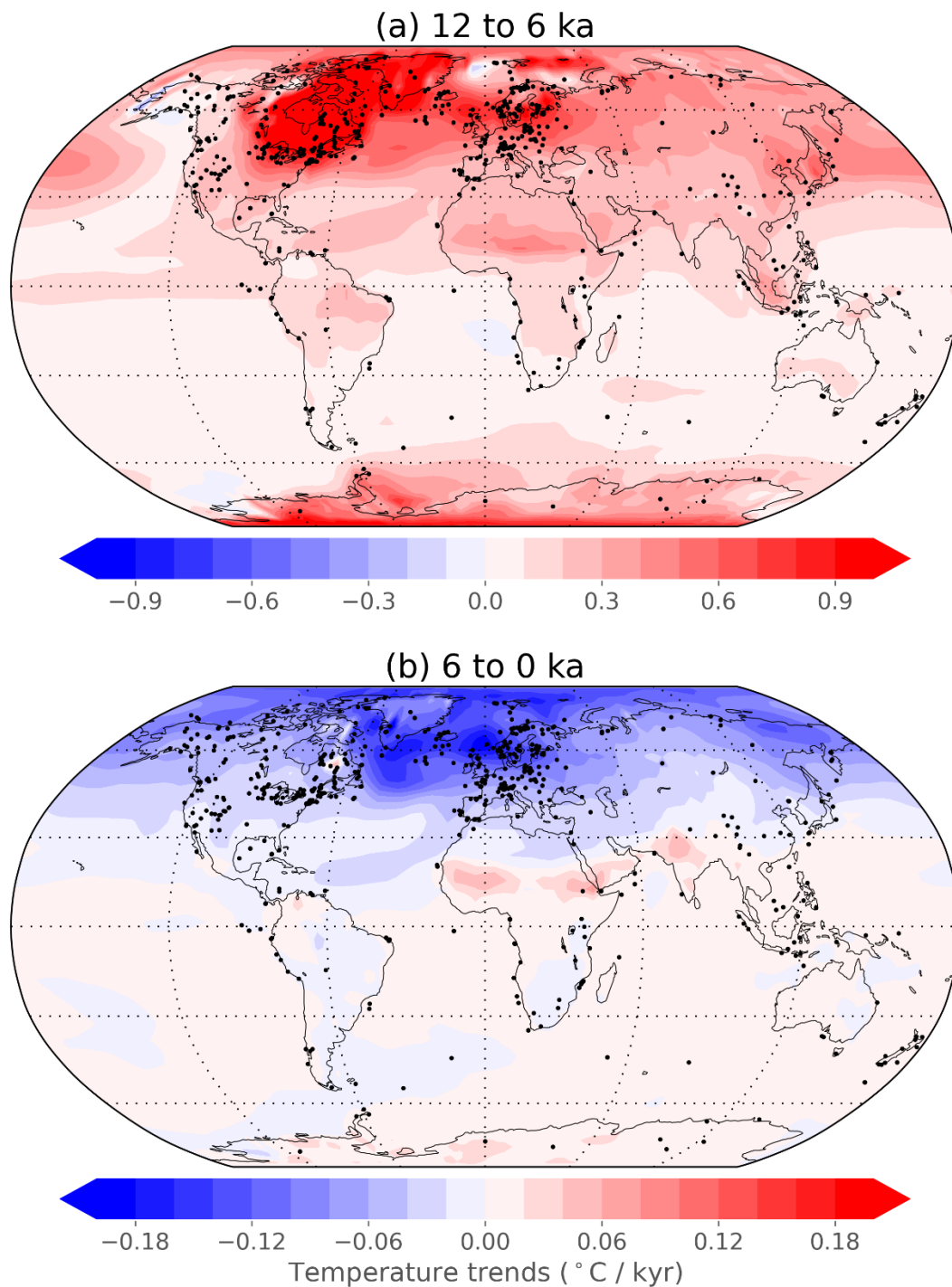
Figure 5. Temperature trends. Temperature trends ( ^{\circ}\text{C} \text{ kyr}^{-1} ) at every location for the periods (a) 12 to 6 ka and (b) 6 to 0 ka. Dots show locations of assimilated proxy records during each period. Note the different scales between the two panels.
