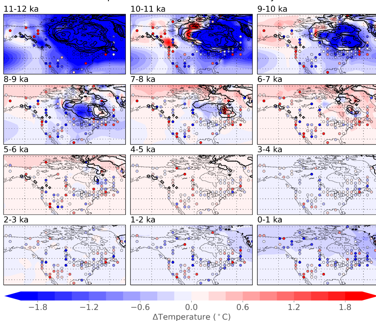
Figure 9. Temperature and ice sheets in North America. Millennial anomalies for reconstructed temperature (shaded, °C), gridded annual mean proxy records (dots, °C), and ice sheets from the ICE-6G_C reconstruction (contours, 500 m interval; Peltier et al., 2015). All values, including ice sheets, are shown for 1000 year means relative to the period 3000-5000 years before present. Proxy values are binned and averaged to the same spatial resolution as the data assimilation for clarity. Summer and winter-biased proxy records—which make up 21% and 1% of the assimilated records, respectively—are not shown, as seasonal records are not directly comparable to the annual reconstruction. The temperature reconstruction is based on proxy values and model covariances, without knowing the specific timing of ice sheet changes.
