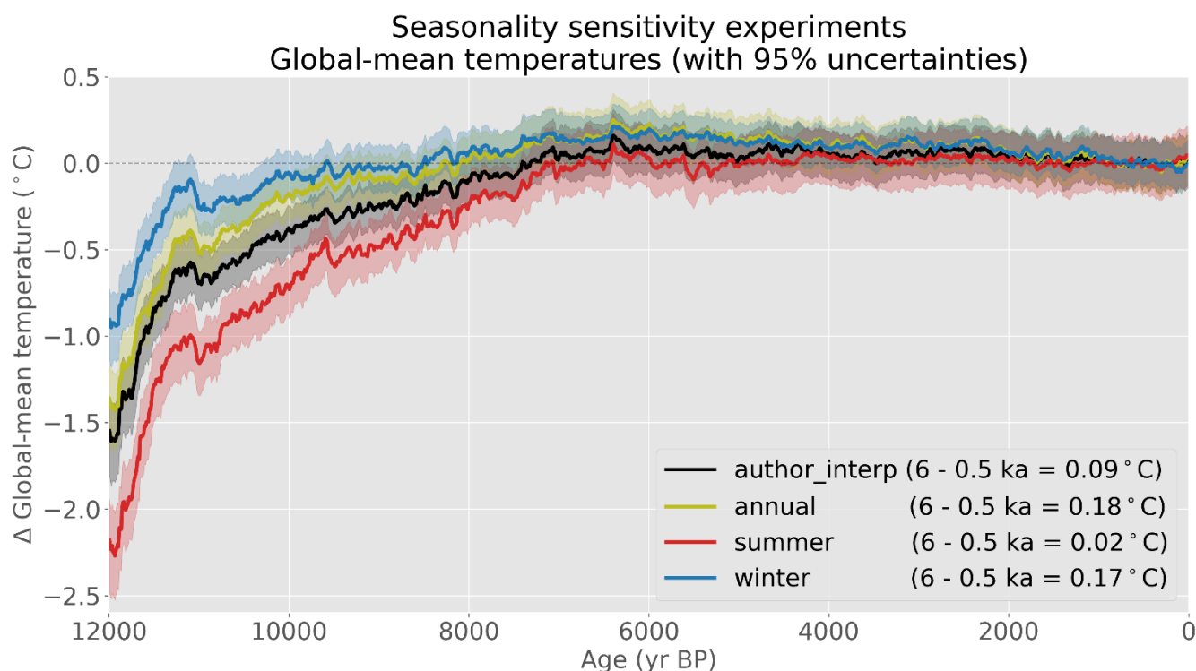
415 Figure 8. Global mean temperature composites created using different assumptions for proxy seasonality. “author_interp” is the default experiment, where proxy seasonality metadata from the Temperature 12k proxy database is used. In the other experiments, all proxies are assimilated as if they represent annual, summer, or winter means. Temperature anomalies are shown relative to 0-1 ka.
