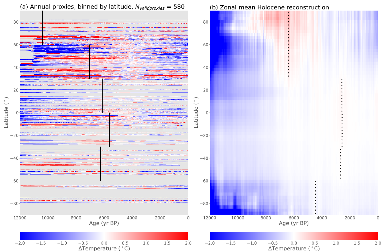
365 Figure 7. Comparison of annual records and zonal mean Holocene Reconstruction. (a) Annual Temperature 12k proxy records binned into 0.5° latitude bands, showing temperatures relative to 3-5 ka. (b) Zonal mean annual temperatures in the Holocene Reconstruction. Panel (a) is like Fig. 1, but only annual records are selected and they are binned by latitude and averaged when multiple records occupy the same latitude band. Panel (a) does not represent zonal means, whereas (b) shows the zonal mean of the 370 reconstruction. Black lines or dots show the timing of the warmest period, calculated by standardizing all latitude bands and finding the warmest mean of each 30° latitude zone where at least 25% of the bands have values.
