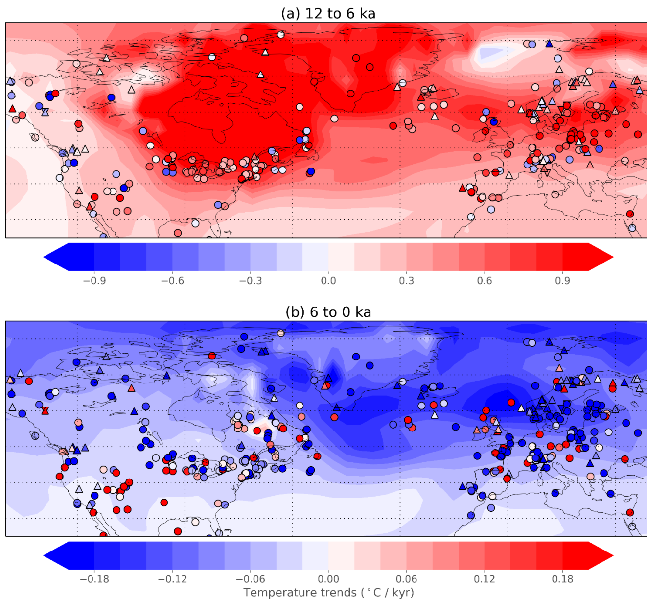
360 Figure 6. Temperature trends in the reconstruction and proxy records for North America and Europe. Temperature trends ( ^{\circ}\text{C} \text{ kyr}^{-1} ) over the periods (a) 12 to 6 ka and (b) 6 to 0 ka, like Fig. 5. Trends in assimilated proxy records are shown as colored symbols, with shapes indicating the seasonality of the proxy (circle: annual; upward-pointing triangle: summer; downward-pointing triangle: winter). Records are only plotted if they have data covering at least half of the time period. Note the different color bars in the two panels.
