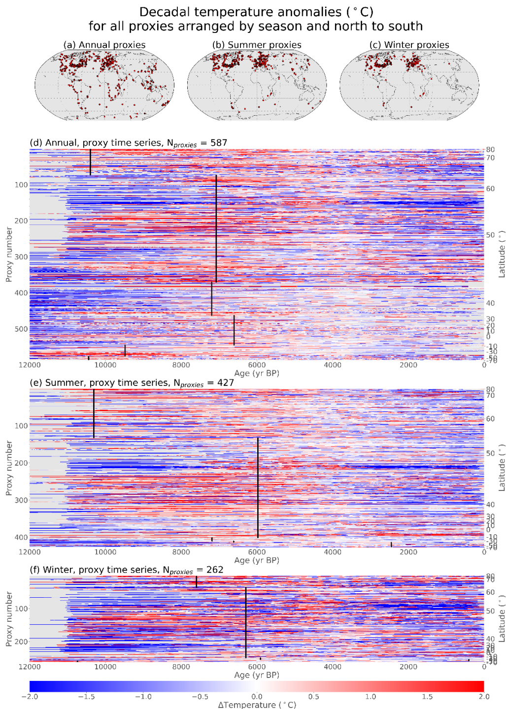
Figure 3. Temperature anomalies for calibrated proxy records separated by seasonal metadata. (a-c) Maps of proxy record locations, separated by season. (d-f) Relative temperatures of calibrated records, as in Fig. 1, separated by season.
