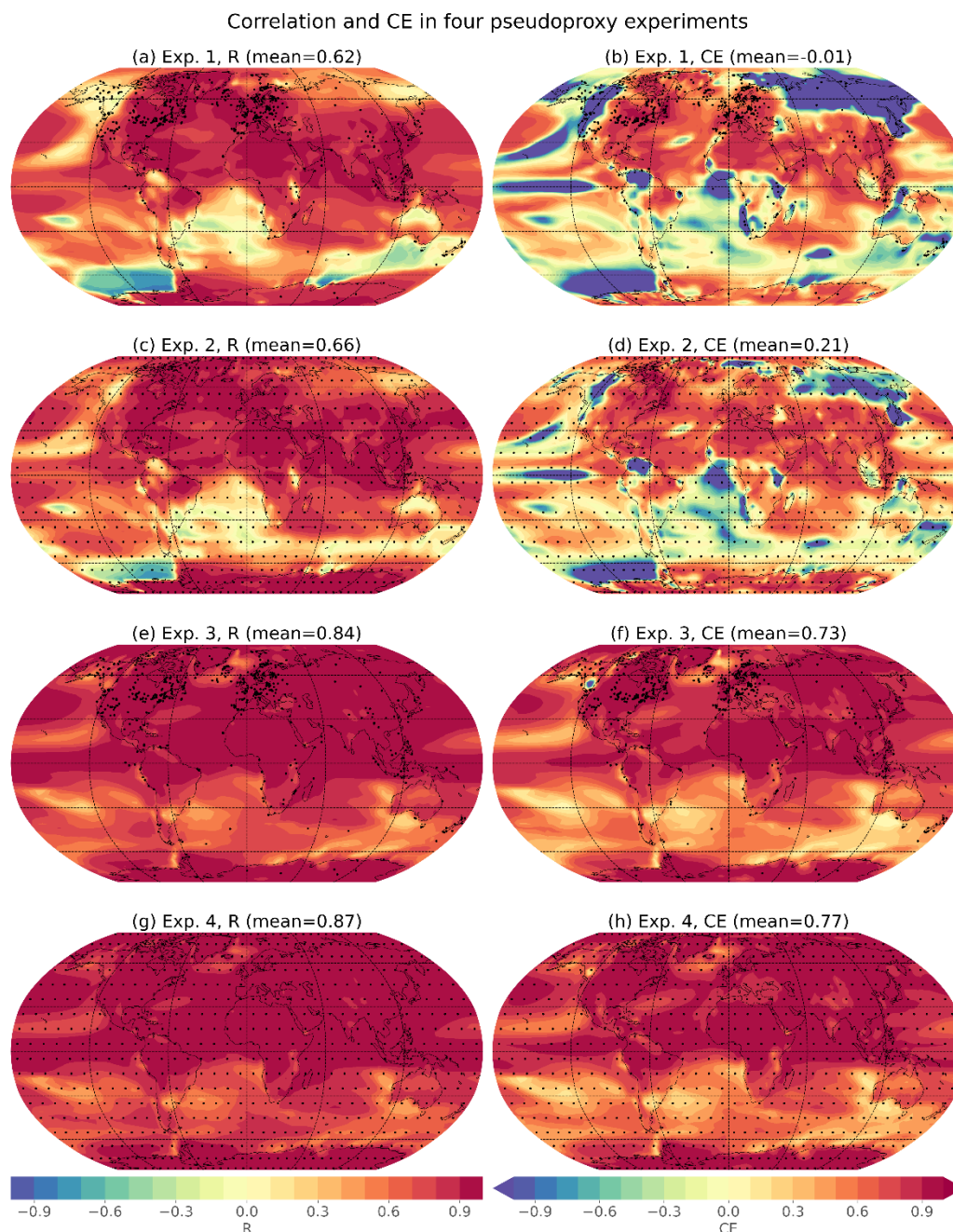
655 Figure A2. Spatial skill of pseudoproxy experiments. Spatial correlations (R) and coefficients of efficiency (CE) for four different pseudoproxy experiments. Global mean values, calculated as the area-weighted mean of the spatial values, as given above each map. Each experiment uses HadCM3 as the prior but differ in the model used to generate the pseudoproxies (Exps. 1, 2: TraCE- 21ka; Exps. 3, 4: HadCM3) and the spatial, temporal, and seasonal characteristics of the pseudoproxies (Exps. 1, 3: as in Temperature 12k; Exps. 2, 4: uniform proxy network). When pseudoproxies are based on the Temperature 12k network, they use the spatial, temporal, and seasonal characteristics as the real proxy records ( N_{\text{pseudoproxies}}=711 ). When pseudoproxies are generated on a uniform 10^\circ by 10^\circ grid, they are all annual mean and cover the entire Holocene with decadal resolution ( N_{\text{pseudoproxies}}=648 ). 660 More details about these experiments are given in Table 2.
