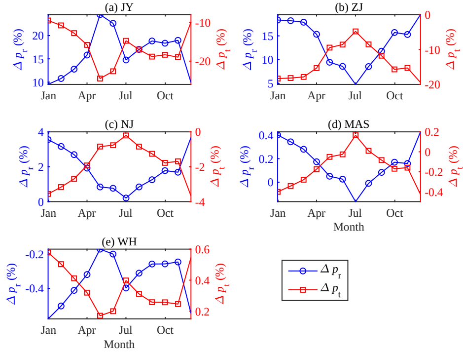
Figure 8. Alterations in variance contributions of riverine \Delta p_r and tidal \Delta p_t forcing at different gauging stations along the upper YRE: (a) Jiangyin (JY), (b) Zhenjiang (ZJ), (c) Nanjing (NJ), (d) Maanshan (MAS), (e) Wuhu (WH).
