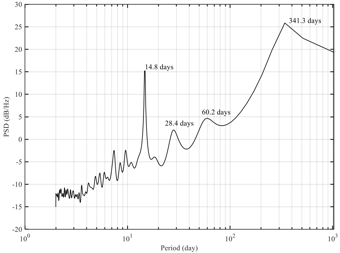
Figure R3. Autoregressive power spectral density estimate of the daily averaged water level observed at TSG gauging station
