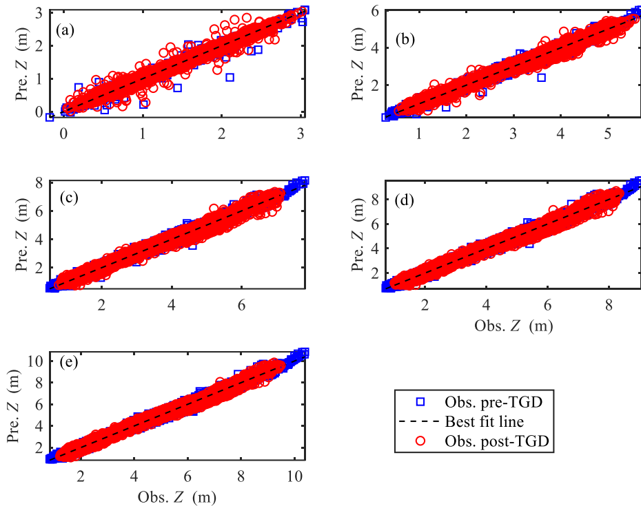
Figure R2. Comparison between predicted and observed daily averaged water levels for both the pre-TGD and post-TGD periods at different gauging stations along the YRE by means of Equation R1: (a) Jiangyin (JY), (b) Zhenjiang (ZJ), (c) Nanjing (NJ), (d) Maanshan (MAS), (e) Wuhu (WH).
