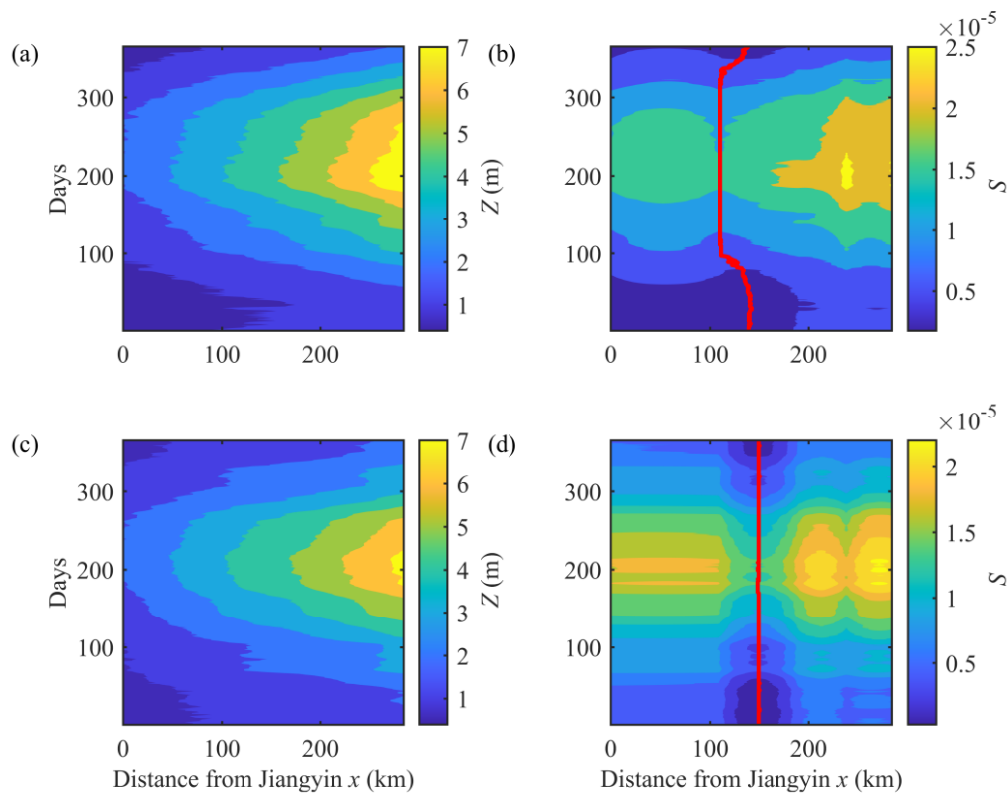
Figure R4. Reconstructed spatial-temporal water levels, Z , (a, c) and their slopes, S , (b, d) for the climatological year during both the pre-TGD (a, b) and post-TGD (c, d) periods. The red lines in subplots (b) and (d) indicate the local minimum water level slopes in the central section of the YRE (between Jiangyin and Zhenjiang).
