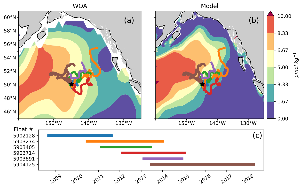
645 Fig 02. Argo float trajectories overlaid on late summer (August) surface nitrate concentrations in (a) the World Ocean Atlas, and (b) MOM6-COBALT. The sampling period of each float is shown in (c). Note that float 5904125 (brown) travels west across the east-west nitrate gradient, and is the only float sampling the region between 2015 and 2018.
