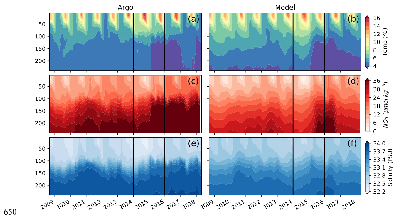
Fig 03. Comparison of observations from BGC-Argo floats shown in Fig 2 (left) and sampled along their trajectories in MOM6-COBALT (right) for temperature (a,b), nitrate concentration (c,d) and salinity (e,f). The “warm blob” period (January 2014 to December 2015) is delimited by vertical black lines.
