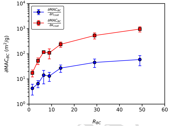
Figure 3. Average change in \text{MAC}_{\text{BC}} per change in coating real refractive index ( \partial \text{MAC}_{\text{BC}} / \partial n_{\text{coat}} ) and average change in \text{MAC}_{\text{BC}} per change in coating imaginary refractive index ( \partial \text{MAC}_{\text{BC}} / \partial \kappa_{\text{coat}} ) with constant \phi . We find that \partial \text{MAC}_{\text{BC}} / \partial \kappa_{\text{coat}} is 4 to 16 times greater than \partial \text{MAC}_{\text{BC}} / \partial n_{\text{coat}} , depending on \rho_{\text{BC}} . These results imply that the choice of the coating imaginary refractive index is more important than the choice of the coating real refractive index when calculating \text{MAC}_{\text{BC}} . Error bars represent 1 standard deviation.
