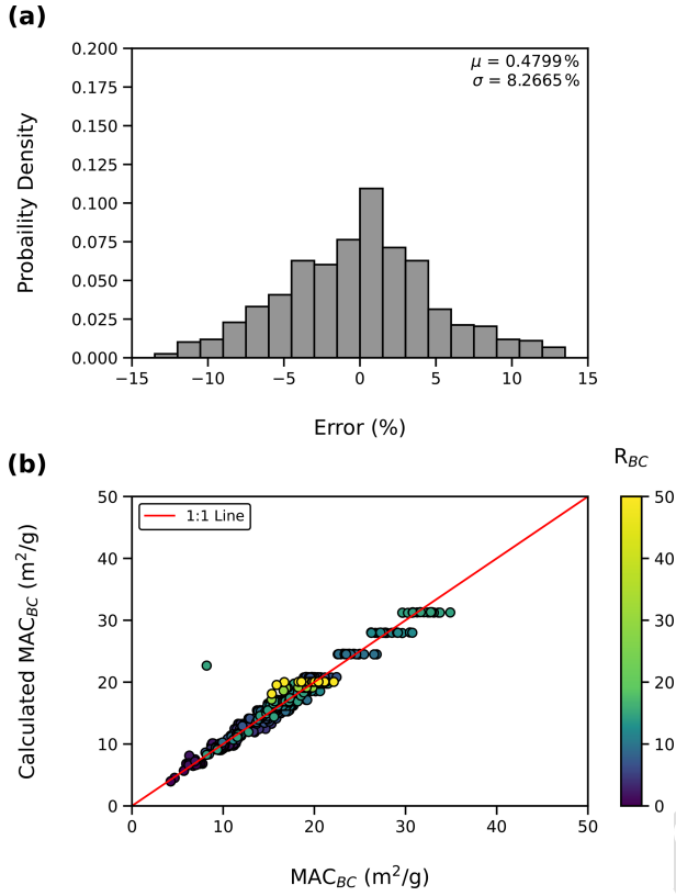
Figure 5. (a) Residual plot of fitting of Eq. (3). On average, Eq. (3) overestimates \text{MAC}_{\text{BC}} by 0.47 %, with a standard deviation of 8.26 % ( \mu and \sigma , respectively). (b) \text{MAC}_{\text{BC}} calculated using Eq. (3) as a function of \text{MAC}_{\text{BC}} from ADDA. Equation (3) accurately predicts \text{MAC}_{\text{BC}} from the mixing state and morphology of the BC aggregates used to develop Eq. (3), but relative errors increase with increased R_{\text{BC}} . It should be noted that the outlier point is a thickly coated aggregate with \rho_{\text{BC}} \gg 1 and \kappa_{\text{coat}} > 0.00 , representing the limitations of the developed framework.
