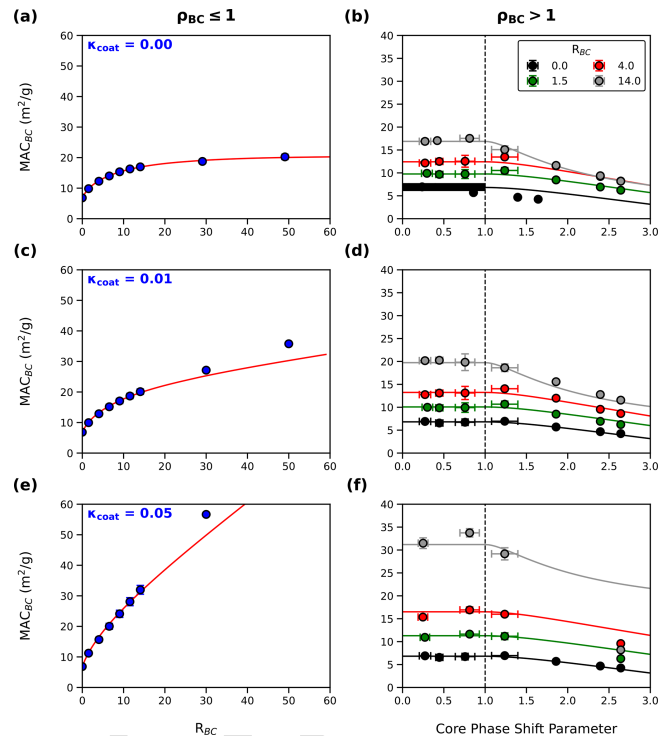
Figure 4. Data and fitting of \text{MAC}_{\text{BC}} as a function of \rho_{\text{BC}} and R_{\text{BC}} for BC internally mixed with a coating imaginary refractive index ( \rho_{\text{coat}} ) of 0.00 (a–b), 0.01 (c–d), and 0.05 (e–f). We find that for constant \rho_{\text{BC}} , \text{MAC}_{\text{BC}} increases with increasing R_{\text{BC}} . Additionally, for constant R_{\text{BC}} , \text{MAC}_{\text{BC}} decreases when \rho_{\text{BC}} surpasses unity. Solid lines show the scaling of \text{MAC}_{\text{BC}} given by Eq. (3).
