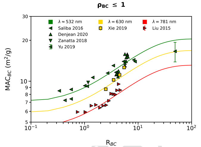
Figure 7. Scaling of MAC_{BC} with R_{BC} for aggregates with \rho_{BC} \leq 1 (Eq. 3a, solid lines) compared to the findings of several other studies which find significant MAC_{BC} (Yu et al., 2019; Saliba et al., 2016; Liu et al., 2015; Xie et al., 2019; Denjean et al., 2020; Zanatta et al., 2018). We find that measurements from these studies are well described by Eq. (3a), indicating that the aggregates measured in these studies had \rho_{BC} \leq 1 .
