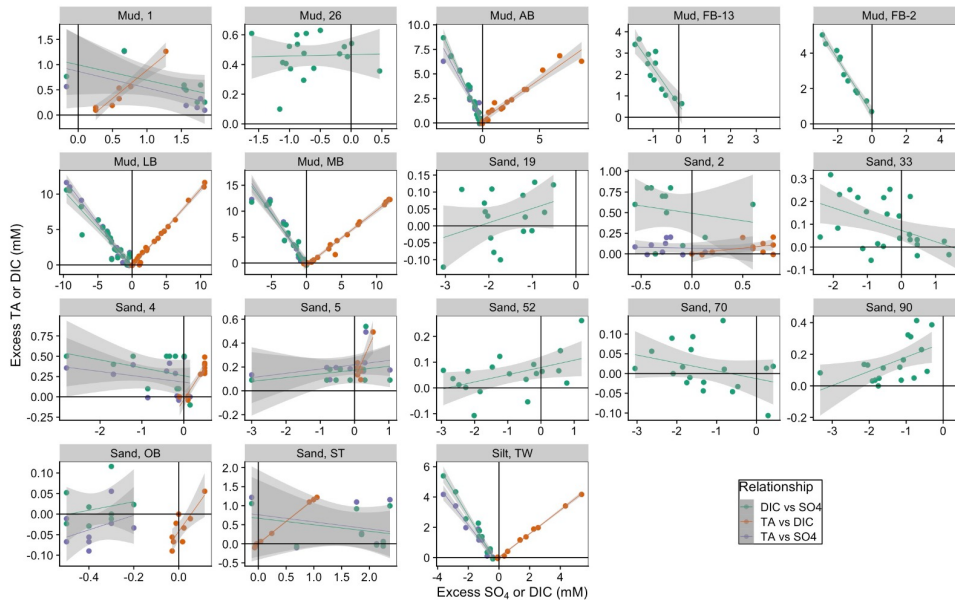
515 Figure 6. Relationships between excess DIC and excess \text{SO}_4^{2-} (green points), excess TA and excess DIC (orange), and excess TA vs excess \text{SO}_4^{2-} (purple). Positive values indicate a larger concentration in porewater relative to surface water.
