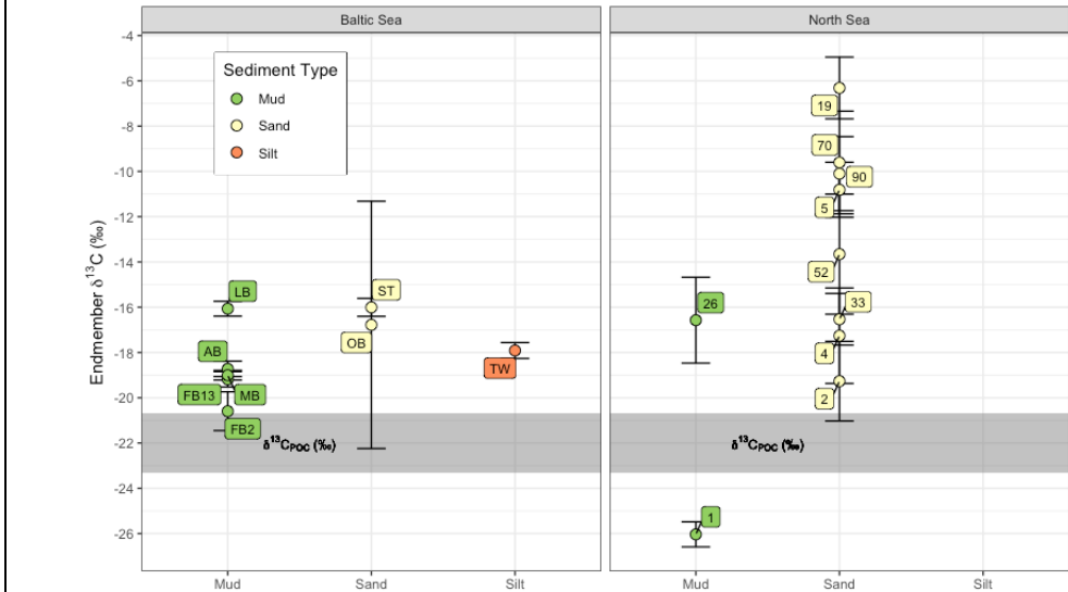
Figure 5. Potential end-member isotopic values for porewater DIC, derived from Miller-Tans plots of DIC * \delta^{13}\text{C} -DIC vs DIC (shown in Fig S1). The grey area represents a range in expected \delta^{13}\text{C} -POC values for the North Baltic seas combined, and the error bars represent the standard error of the Miller-Tans slope.
