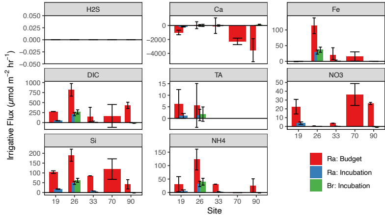
Figure 3. Average sediment-water fluxes ( \mu\text{mol m}^{-2} \text{hr}^{-1} ) derived from Ra or Br- incubation or Ra-decay from the North Sea sites only. In this figure, the error bars represent minimum and maximum fluxes calculated from replicate pore-water cores taken at each site.
