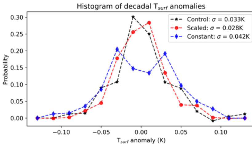
240 Figure 9. Histogram of decadal averaged surface temperature anomalies (K) in CONTROL (black), SCALED (red) and CONSTANT (blue)
