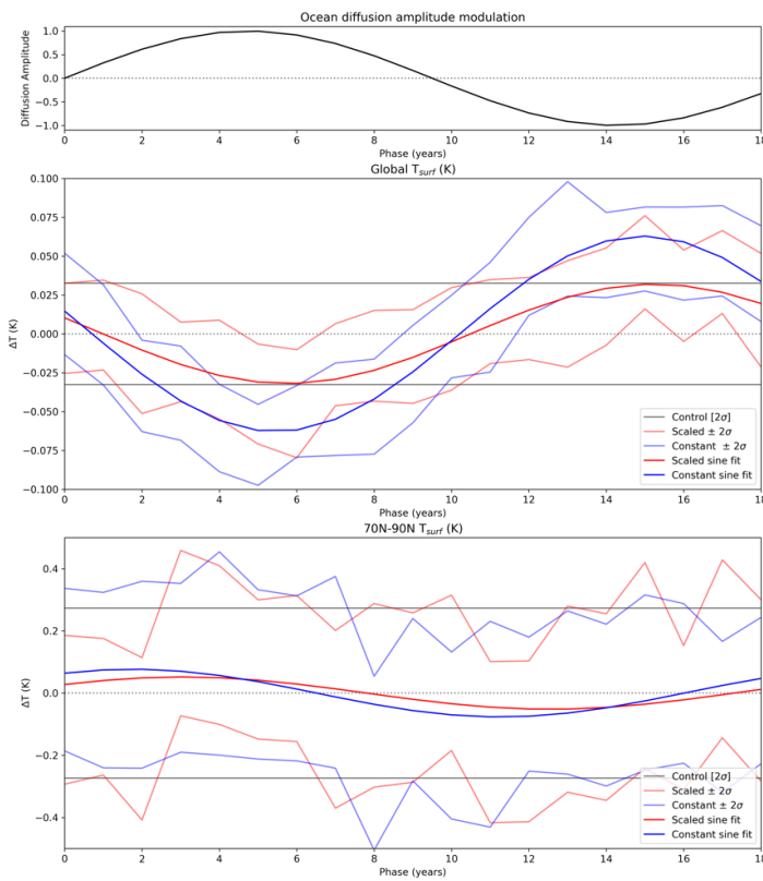
145 Figure 4. As Figure 3 but Middle panel- globally averaged surface temperature T_{surf} (K) vs tidal modulation phase. Bottom panel- as for middle panel but for surface temperature (K) in the Arctic region (70°N-90°N).
