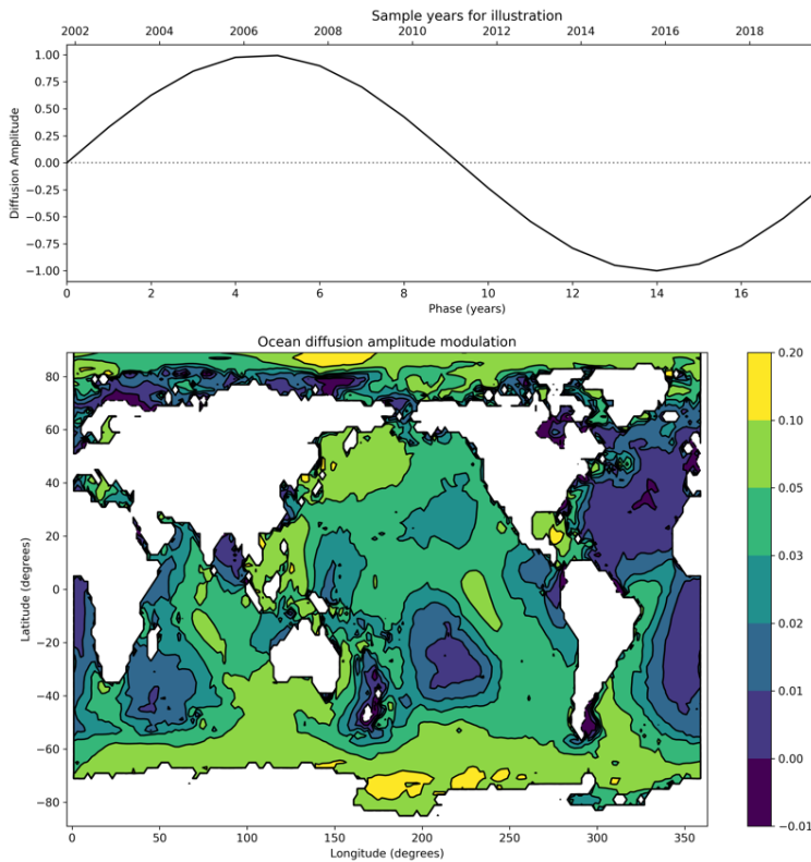
90 Figure 1. Top panel- variation in time of the modulation (with reference year for illustrative purposes on the top axis). The tidal modulation in the model is the top panel T(t) multiplied by the bottom panel M(x,y) , multiplied by 1.0 for run CONSTANT, or a scaled function in run SCALED- see equation (1). Bottom panel- geographical distribution of the modulation of tidally-driven diffusion by the 18.6 year lunar nodal cycle.
