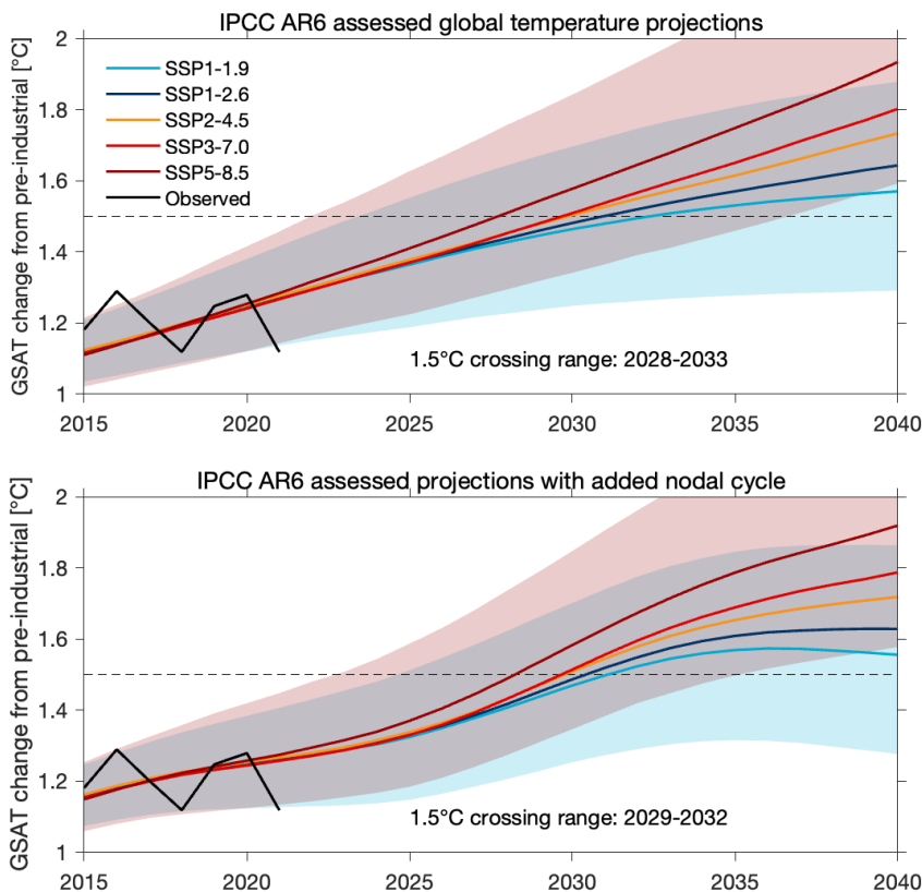
265 Figure 10. Top panel: IPCC AR6 assessed trends for different shared socioeconomic pathways (SSPs). Bottom panel: as top panel but with a lunar nodal cycle of 0.04K amplitude, chosen to be approximately an average of the CONSTANT and SCALED runs.
