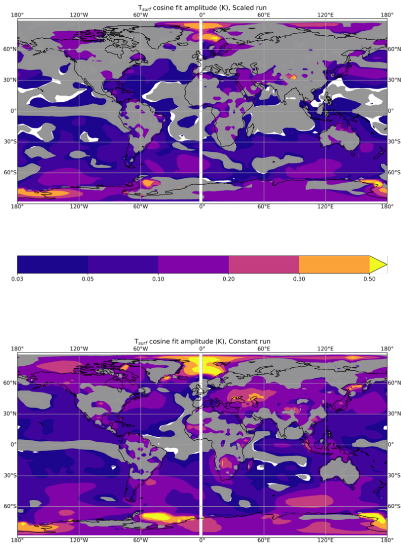
160 Figure 5. Top panel- geographical variation of the amplitude of the sinusoidal trigonometrical fit to surface temperature (K) whose globally-averaged counterpart is shown in Figure 4 (middle panel) in SCALED; i.e. yellow colours are where the fitted curve has an amplitude of > 0.5K . Grey shaded areas show where the amplitude is less than 2 standard errors of annually averaged T_{surf} in the CONTROL integration and are used to denote areas where the response is likely to be noise; note nonlinear contour interval. Bottom panel- as top panel but for CONSTANT.
