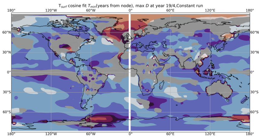
215 Figure 6. Top panel- geographical variation of the phase of the sinusoidal trigonometrical fit to surface temperature (K) shown in Figure 5. At each point, the colour denotes the phase in years (see Figure 1 top panel) where the fitted T_{surf} reaches its most negative value. Note the cyclic colour interval, since a phase of 19 years is equivalent to a phase of 0 years. Blue colours correspond to phases associated with a globally averaged minimum in T_{surf} (Figure 4 middle panel). As with Figure 5, grey shaded areas show where the amplitude is less than 2 standard errors of annually averaged T_{surf} in the CONTROL integration and are used to denote areas where the response is likely to be noise. Bottom panel- as top panel but for CONSTANT.
