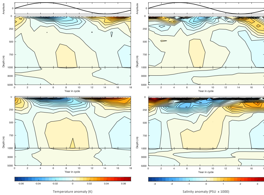
105 Figure 2. Top left panel- globally averaged variation of ocean temperature anomalies (K) vs ocean depth and phase (years) in the SCALED run. The phase coordinate describes the temporal modulation of the vertical diffusion shown in the inset at the top (T(t) in equation 1), and in Figure 1 (top panel), i.e. maximum diffusion is in year 5 and minimum diffusion is in year 14. Bottom left panel- as top left but for CONSTANT run. Top right panel- as top left but for global salinity (PSU). Bottom right panel- as bottom left but for global salinity.
