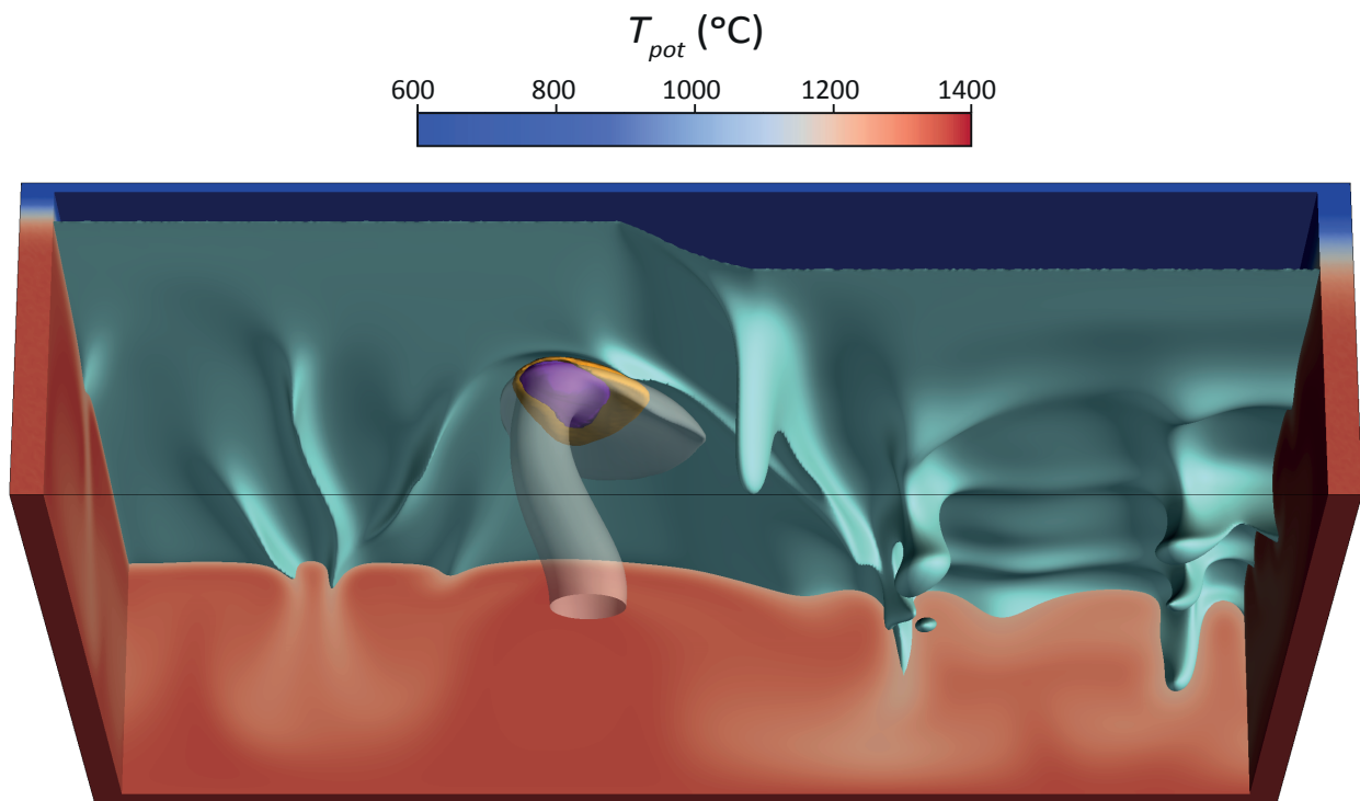
Figure A5. Snapshot of test case with an increased continental lithospheric thickness ( \tau_c = 200 Ma), D_{plume} = 200 km, and otherwise properties as in the reference case. See text for details.
