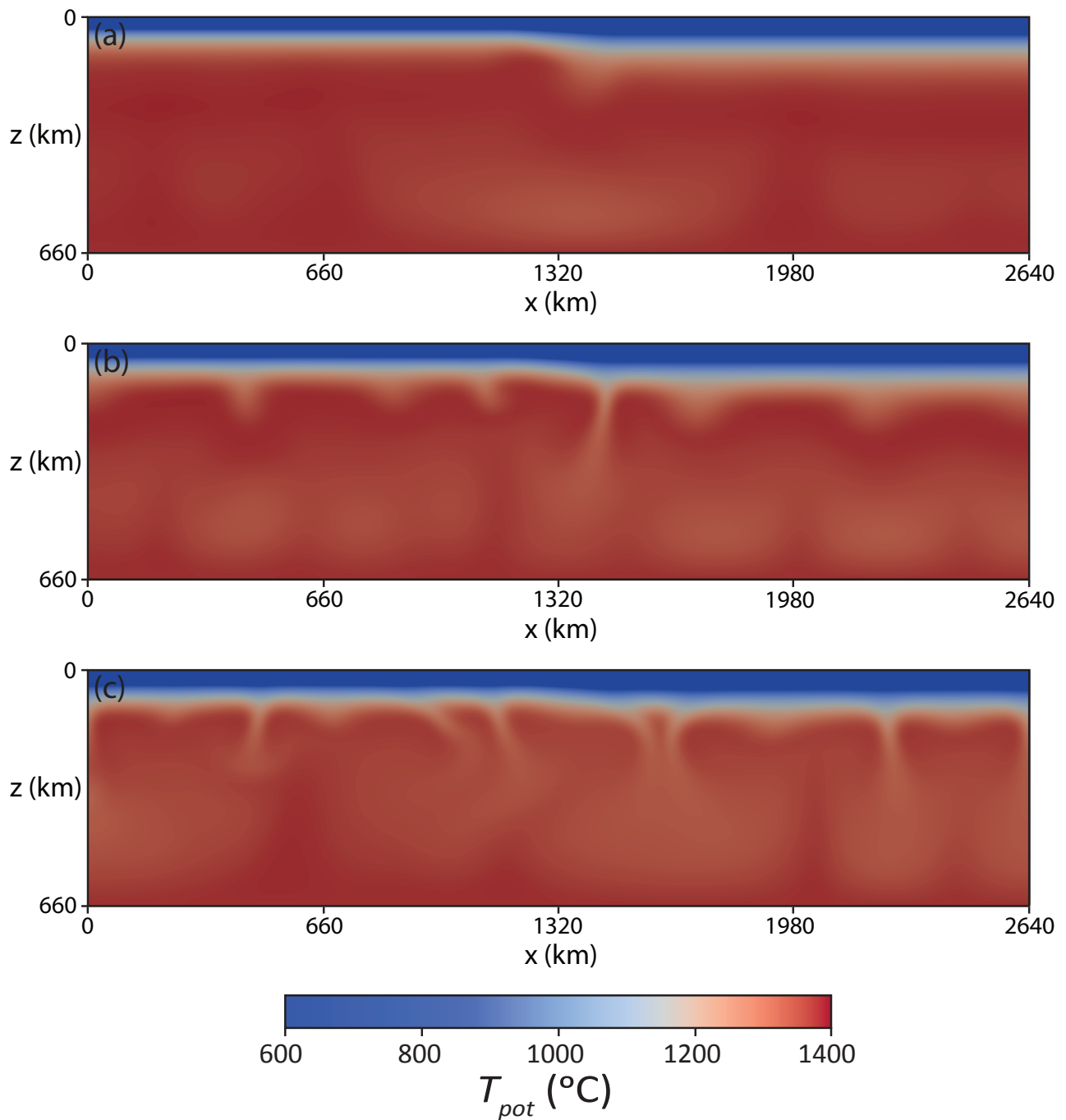
Figure A3. Vertical cross-sections of a case without a plume perpendicular to plate velocities. (a) y = 220 km; (b) y = 660 km; (c) y = 1320 km. Compared with Figure 3 of Manjón-Cabeza Córdoba and Ballmer (2021), changes in time of EDC are well represented in depth, while plate velocities do not disrupt the general planforms of EDC.
