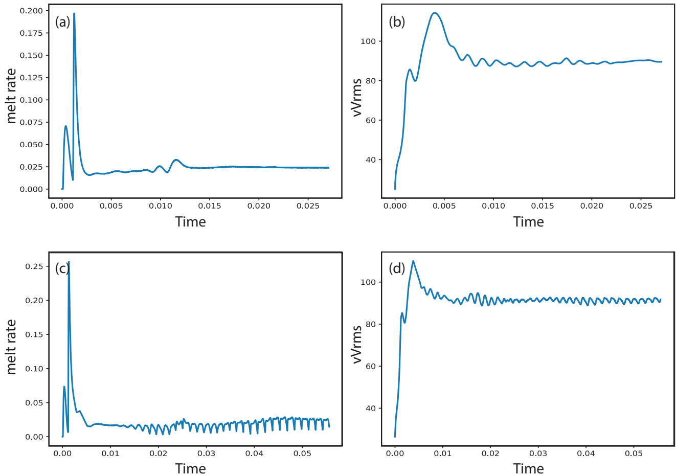
Figure A1. Example of trends used to evaluate steady state in our models. Shown are the reference case (panels a and b, see also Figure 3), and the case of D_{plume} = 400 km, \Delta T_{plume} = 150 °C and B_{plume} = 100 kg·s -1 (panels c and d, see also Figure 7b and supplementary video). Panels (a) and (c) show the total melting rate (integrated across the whole model) and panels (b) and (d) show the root mean square of the vertical velocity (vVrms). All axes are in non-dimensional scale.
