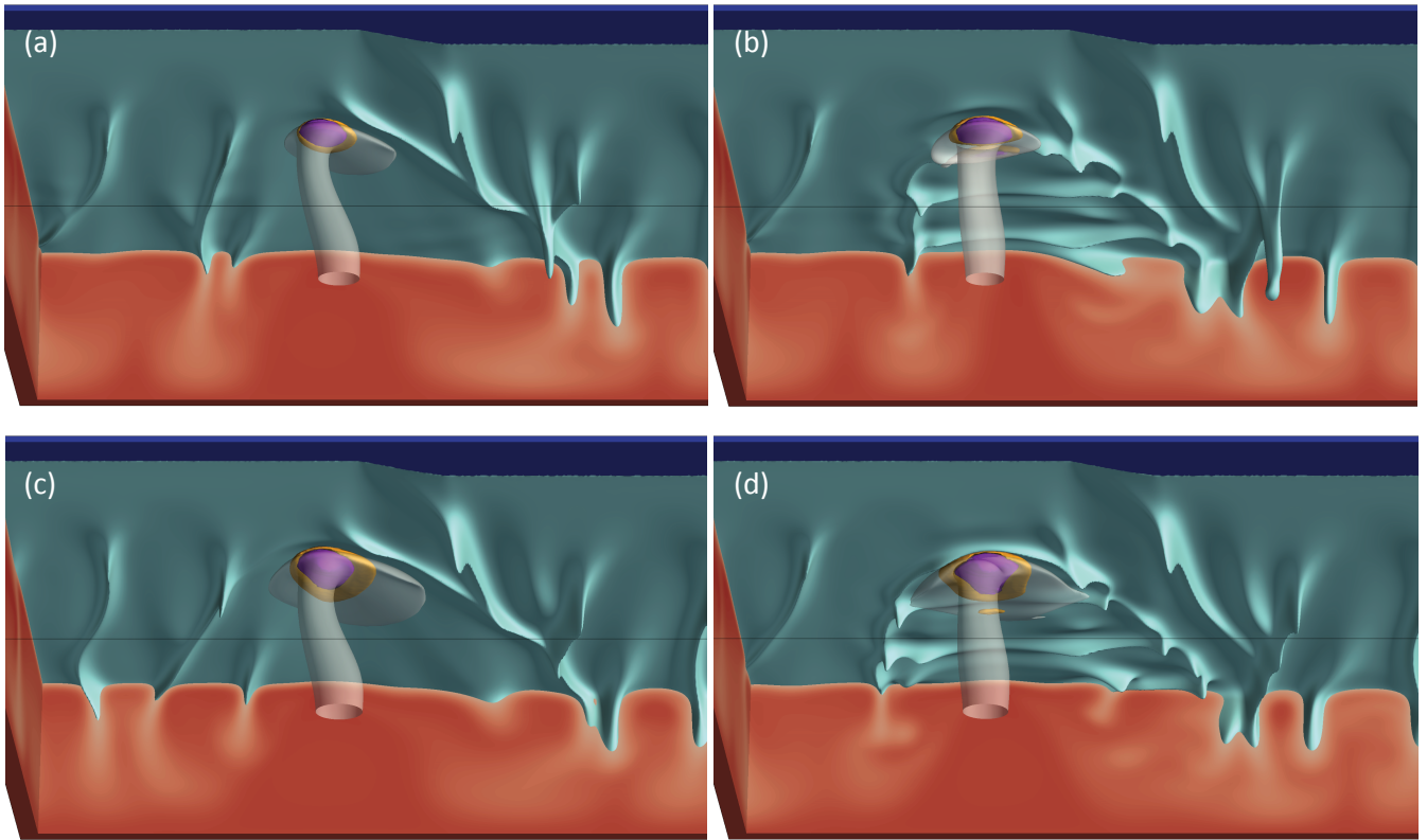
Figure 7. Steady-state snapshots of representative cases with variable D_{plume} . (a,c) Cases with D_{plume} = 200 km. (b,d) Cases with D_{plume} = 400 km. In the top row, models with a relatively weak plume with \Delta T_{plume} = 150 °C and B_{plume} = 100 kg·s -1 are shown. In the bottom row, models with a relatively strong plume with \Delta T_{plume} = 200 °C and B_{plume} = 200 kg·s -1 are shown. For reference to colors of surfaces and cross-sections, see fig. 3 caption and legend. The 3D perspective is the same as in Figure 3.
