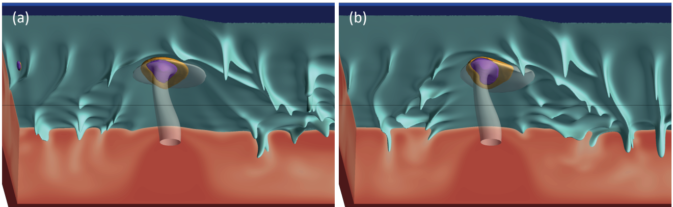
Figure 10. Steady-state model snapshot for the low viscosity cases ( \eta_0 = 5.53 \times 10^{18} Pa·s). (a) Case with D_{plume} = 200 km and B_{plume} = \text{kg} \cdot \text{s}^{-1} . (b) Case with D_{plume} = 300 km and B_{plume} = \text{kg} \cdot \text{s}^{-1} . Note that the deflection of the pancake at 300 km is greater than that of 200 km (Figure 9) as opposed to the case for intermediate and high viscosity.
