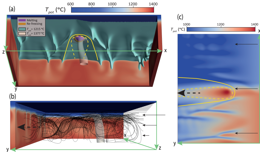
Figure 3. Steady-state temperature field and melting for the reference case with \Delta T_{plume} = 150 °C, B_{plume} = 100 kg·s -1 , D_{plume} = 0 km, and \eta_0 = 8.29 \cdot 10^{18} Pa·s. (a) Front perspective of the reference case. Cross sections of potential temperature (at the margins of the model) are shown in red-to-blue colors. The light blue and white surfaces mark isotherms (as labeled), showing the base of the lithosphere and the plume, respectively. The purple isosurface outlines the region of active melting while the orange isosurface outlines the region of finite melt presence, including where active melt re-freezing occurs. Dashed and solid lines depict the dynamic and thermal PET (see text) respectively. (b) Side view of the model with stream lines. (c) top-view with cross section of the temperature field at z = 106 km. Black arrows depict plate motion. Note that the colorscale is different than in panels (a) and (b).
