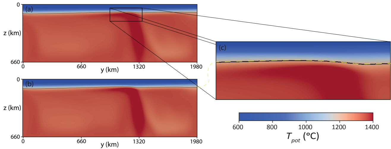
Figure A4. Vertical cross-sections parallel to the edge (perpendicular to the x -direction) and x = 1254 km. The isotherm of T_{pot} = 1215 ^{\circ}\text{C} is drawn as a black line. (a) Reference case. (b) Case with \Delta T = 200 ^{\circ}\text{C} and other values as in the reference case. (c) Closeup of the reference case with the isotherm of the case depicted in panel (b) (dashed yellow line). Note that due to plume deflection, the x coordinate for maximum lithospheric erosion does not correspond with the location of the thermal anomaly at the bottom.
