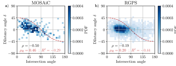
Figure 6. Scatter plot of the dilatancy angles \delta versus the intersection angles between LKFs. The correlation between the intersection angle and the dilatancy angle is \rho = -0.5 for MOSAiC and \rho = -0.19 for RGPS. The red dashed line shows the relationship between dilatancy and angles expected following a normal flow rule or the Roscoe angle theory. The correlation between this prediction and the observed dilatancy angles are \rho_R = 0.46 for MOSAiC and \rho_R = 0.20 for RGPS. All correlations are significant.
