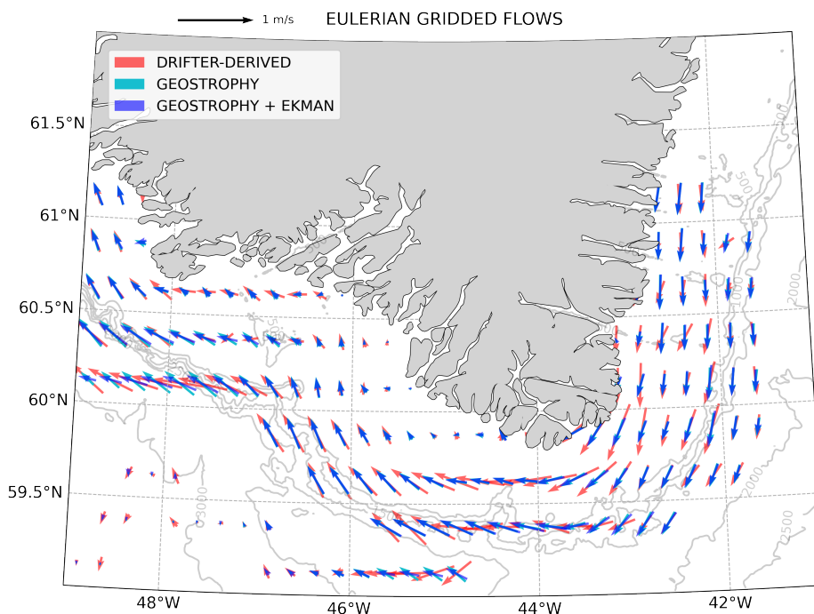
Figure 6. Gridded surface currents derived from drifter data (red), Geostrophy product (cyan) and Geostrophy+Ekman product (blue).
