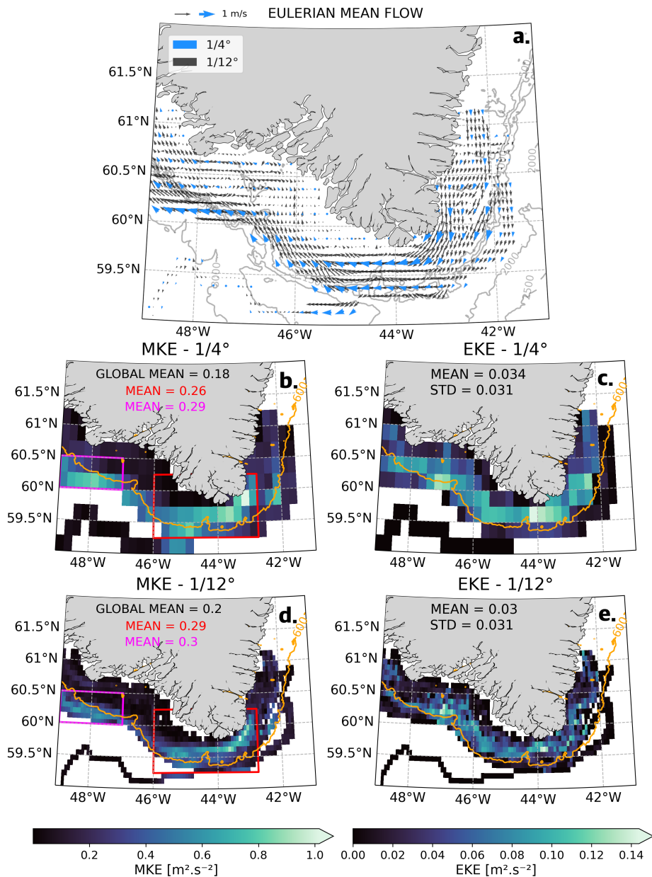
Figure 8. Comparison of gridded flows derived from drifter trajectories with varying resolution. (a) Comparison of 1/4^\circ (blue) and 1/12^\circ (black) vectors. Mean Kinetic Energy (MKE) maps obtained on 1/4^\circ (b) and 1/12^\circ (d) grids. Eddy Kinetic Energy (EKE) maps obtained on 1/4^\circ (c) and 1/12^\circ (e) grids. Values provided in panels b-e are the means over the color-coded boxes.
