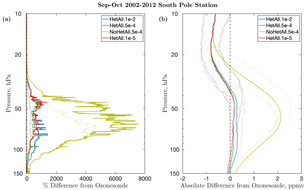
Figure S5. Same as Fig. 5 of the main manuscript, but showing South Pole Station.
