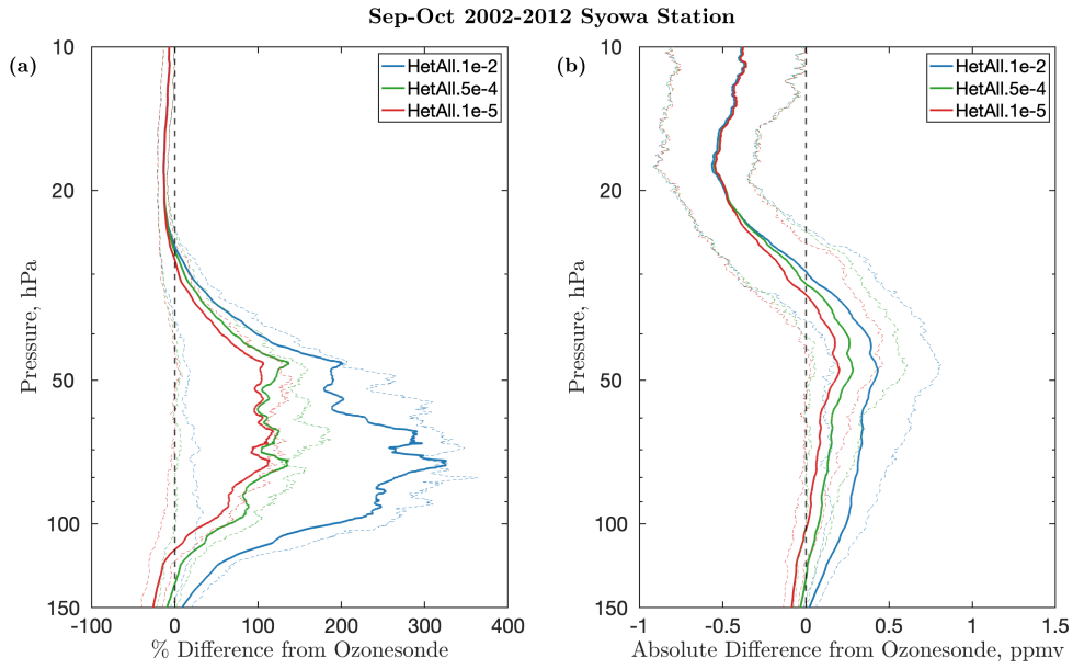
Figure S4. Same as Fig. 5 of the main manuscript, but showing Syowa Station without the noHetAll simulation.
