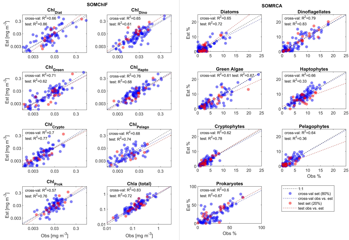
Figure 5. Results of the two-step cross-validation (blue) and test (red) procedures for SOMChIF (left) and SOMRCA (right) with the chosen best combination of satellite parameters and a SOM grid, respectively, of 242 and 222 neurons. From the initial dataset consisting of 145 observations, two sets were split: 80% to be used in a one-leave-out cross-validation procedure, and 20% as an independent test. For the cross-validation, each observation among the 115 observations, was used iteratively as a training set and as a test set until all observations served as tests (blue dots). This procedure was used to identify the best satellite combination and SOM grid size. Finally, the remaining 30 observations were used as a test to evaluate the generalization capacity of the SOM with the chosen configuration (red dots). One should note that, for SOMChIF, the R^2 was calculated using log-transformed Chla values. For complete evaluation metrics refer to Table 3.
