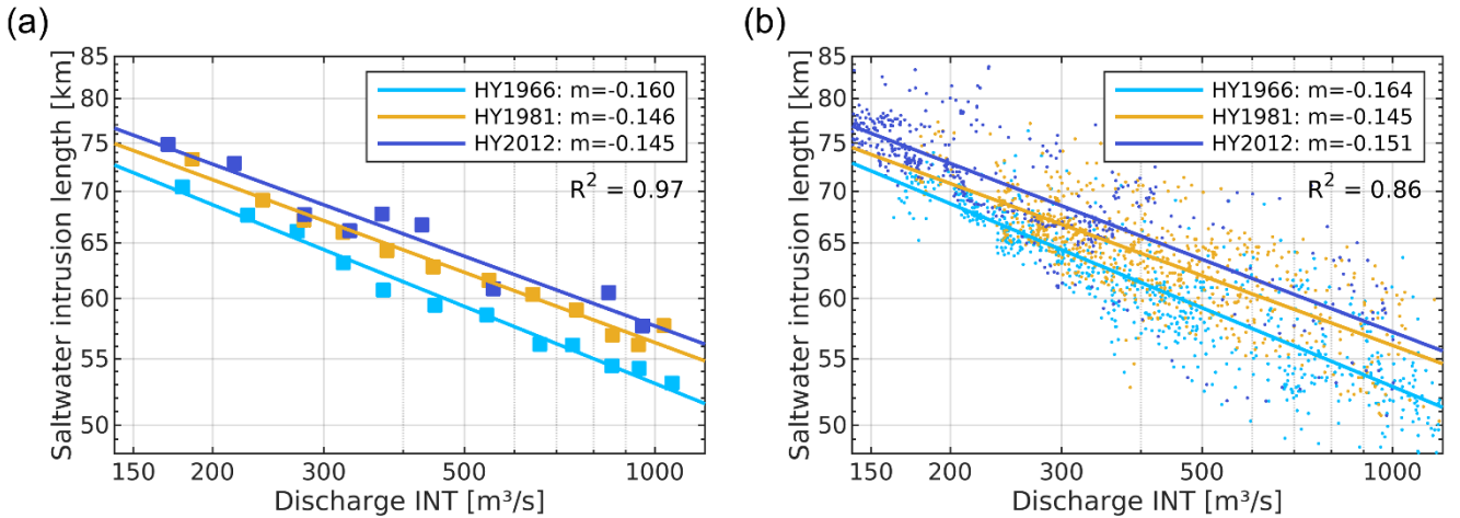
Figure 6. Saltwater intrusion length L^* (distance from the estuary mouth at Weser-km 126.2, see Fig. 1, along the navigation channel to the tide-averaged 5 psu isohaline) in hindcast models of 1966, 1981, and 2012, in relation to discharge Q measured upstream of weir Bremen at station Intschede (INT). On the left, squares represent the average saltwater intrusion length for different discharge categories and lines represent trends of the form L^* = kQ^m . With logarithmic scales, m represents the gradient of the lines (a). The analysis was repeated with non-aggregated data points to test the method's validity (b).
