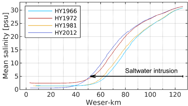
Figure 5 Annual mean, vertically averaged salinity along the navigation channel of the Weser estuary (see Fig. 1) in hindcast models of 1966, 1972, 1981, and 2012.
