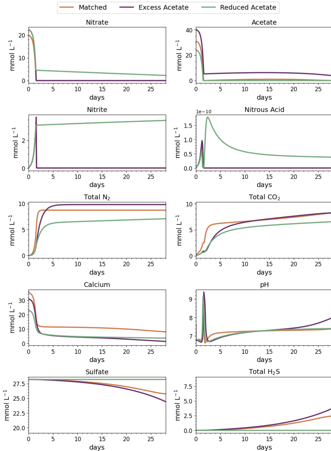
360 Figure 4. Water-quality results for 28 days of MIDP in coastal seawater conditions targeting a desaturation level of 10% in three different treatment recipes: empirically matched, 25% excess acetate, and 25% reduced acetate.
