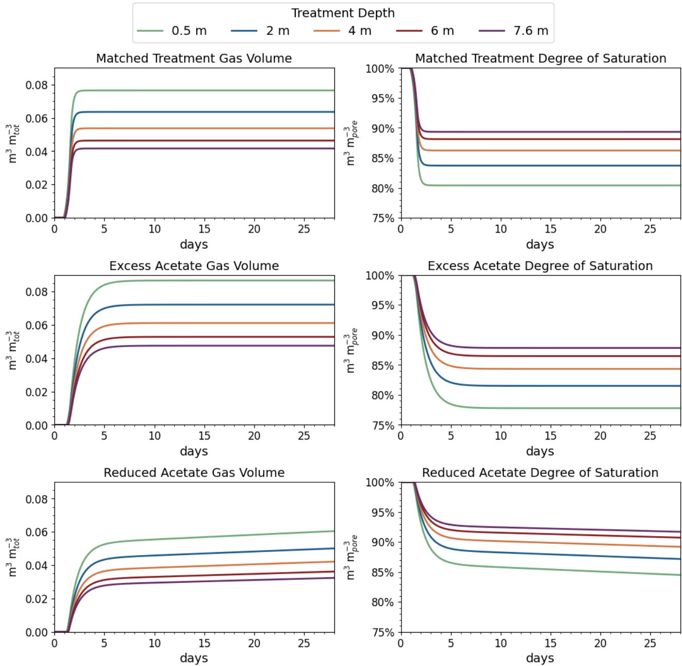
Figure 3. Gas volumes normalized to the total soil volume (left) and degree of saturation by depth for the simulated Coastal seawater conditions. The desaturation target was 10%, or a saturation ratio of 90%.
