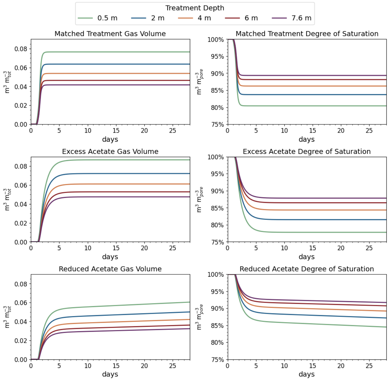
Figure 3. For the coastal seawater conditions, the target desaturation level of 10% at 7.6 m (or a degree of saturation of 90%) was achieved by N_2 generation in approximately 2.0 days. The amount of CO_2 produced did not reach its saturation threshold, and CO_2 did not contribute to desaturation at any of the modeled depths. The difference in volume of gas at the different levels is due to the increase in hydrostatic pressure with depth.
