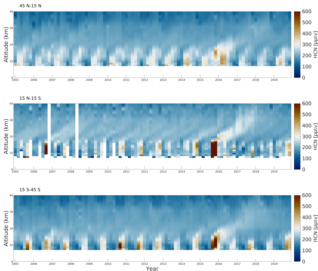
Figure 2. Time-altitude sections of two-month-mean HCN mixing ratios (pptv) from ACE-FTS averaged into three 30^\circ latitude bins, 45^\circ\text{N} - 15^\circ\text{N} , 15^\circ\text{N} - 15^\circ\text{S} and 15^\circ\text{S} - 45^\circ\text{S} for 2005–2020. Note that the colour scale saturates and the maximum observed HCN mixing ratio in the tropical band in 2015 is over 1300 pptv.
