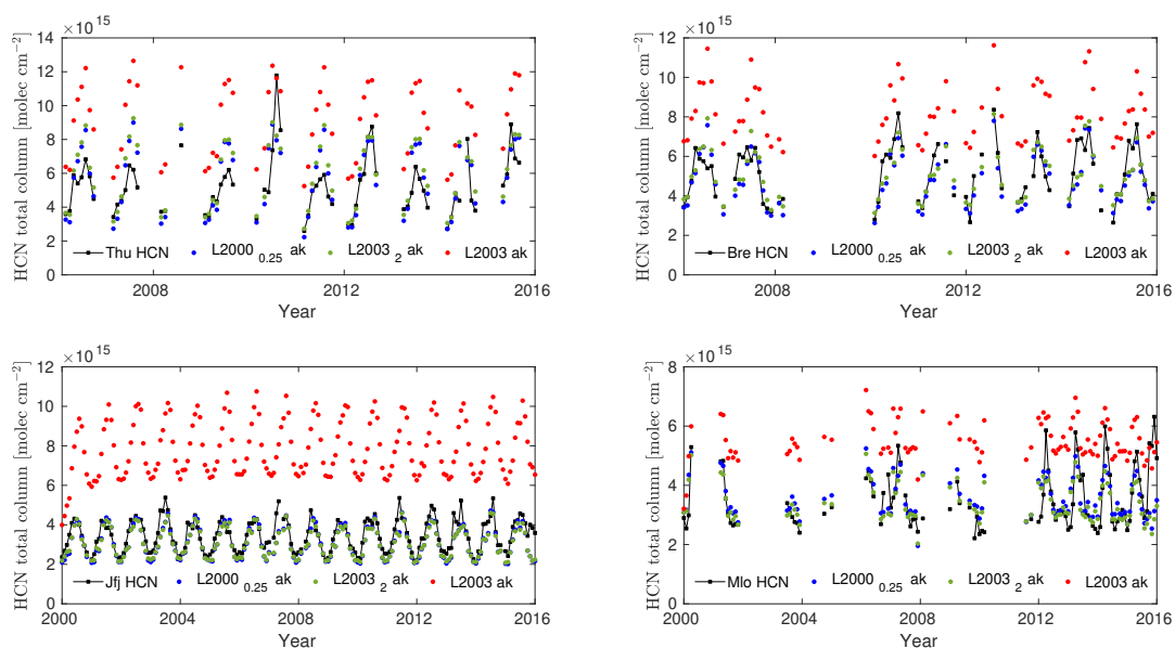
Figure 4. HCN total column time series (molecules cm -2 ) measured at 4 NDACC stations (Thule (Thu), Bremen (Bre), Jungfraujoch (Jfj), and Mauna Loa (Mlo); black lines) and modelled by the L2000 0.25 (blue dots), L2003 2 (green dots) and L2003 (red dots) tracers (with averaging kernels applied). Note the different time periods at the different stations.
