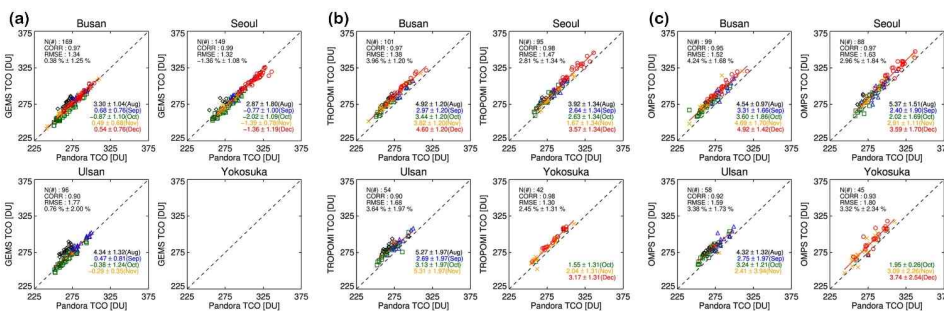
300 Figure 44. Scatter plots of Pandora TCO with (a) GEMS TCO, (b) TROPOMI TCO, and (c) OMPS TCO at Busan, Seoul, Ulsan, and Yokosuka. A linear fit representing a 1:1 ratio is shown in black dotted lines. The legends of N, CORR, RMSE and the number in percentage represent the number of data points, correlation coefficient, RMSE, and mean bias with standard deviation, respectively. The number on the bottom right is the percentage bias for each month. The comparison between GEMS and Pandora was conducted at the overpass time of TROPOMI/OMPS to eliminate potential errors that vary over the course of the day and were not included in this comparison. As mentioned earlier, because GEMS operates in Full West mode starting at 13 KST during November and December, and there are no GEMS measurements at the overpass time of TROPOMI/OMPS in Yokosuka, Japan.
