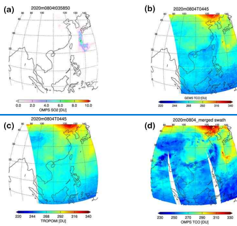
450 Figure 11. The map of (a) OMPS SO 2 , (b) GEMS TCO, (c) TROPOMI TCO, and (d) OMPS TCO in the case of the volcanic eruption of Nishinoshima on 4 August 2020.
