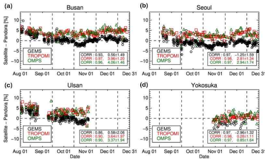
Figure 55. Time series of the daily percentage difference between Pandora and three satellite observations (with GEMS in black, TROPOMI in red and OMPS in green) at Busan, Seoul, Ulsan, and Yokosuka from August to December, 2020.
