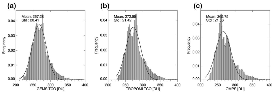
415 Figure 99. Histogram distribution of TCO from (a) GEMS, (b) TROPOMI, and (c) OMPS from August 01 to December 31, 2020, with their corresponding Gaussian fitting lines (black).
