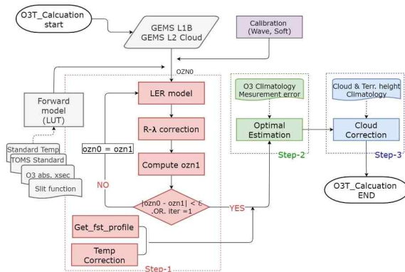
Figure 11. Flowchart of GEMS-O3T retrieval algorithm, consisting of a forward model for TOA radiance calculation and an inverse model for total ozone derivation. Step 1-3 are highlighted with pink, green, and blue color, respectively.
