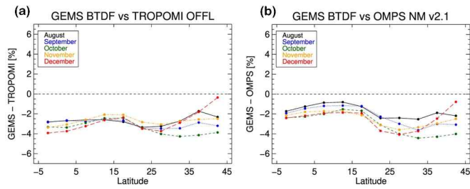
Figure 1313. The Mean Bias (MB) in TCO between GEMS with BTDF correction and TROPOMI (on the left), and between GEMS with BTDF correction and OMPS (on the right), as a function of latitude and month from August 2020 to December 2020.
