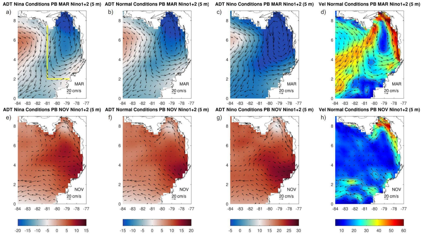
33 34 Figure 4. Monthly averaged ADT anomalies (color scale in cm) and associated geostrophic circulation (vectors) for the Panama 35 Basin. Seasonal changes are indicated within two months: March (a,b,c) and November (e,f,g). ENSO-related conditions (based on 36 Niño 1+2) shown are: normal (b,f), negative ENSO (a,e) and positive ENSO (c,g). Each condition has a different color range to 37 highlight the ADT regional gradients, responsible for the geostrophic circulation. ADT Anomalies are computed subtracting the 38 ETP regional mean during the 1993-2019 period (66.5 cm). Geostrophic vectors and their speed (color scale in \text{ms}^{-1} ) for normal 39 conditions are included for the same months (d,h) with 20 and 40 \text{cms}^{-1} contours included. In panel (a) the yellow line indicates the 40 Panama Bight area used to compute regionally-averaged time series shown in Figure 5a to d.
