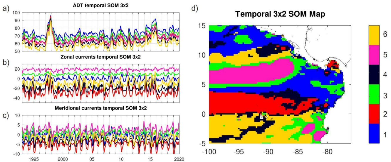
99 Figure 7. a) Absolute Dynamic Topography (cm), b) zonal and c) meridional geostrophic currents (cm s -1 ) time series from 1993 to 00 2019 which results from a 3x2 SOM temporal analysis in the Eastern Tropical Pacific. d) Sub-regions represented by the six temporal 01 SOM patterns.
