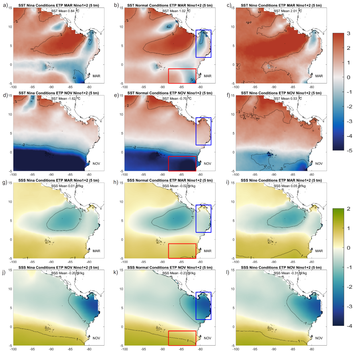
56 57 Figure 5. Monthly averaged anomalies of Sea Surface Temperature (SST – a to f) in °C and Sea Surface Salinity (SSS - g to l) in gr 58 kg -1 for the Eastern Tropical Pacific – ETP. Seasonal changes are indicated within two months: March (a,b,c and g,h,i) and 59 November (d,e,f and j,k,l). ENSO-related conditions (based on Niño 1+2) shown are: negative ENSO (first column), normal (second
