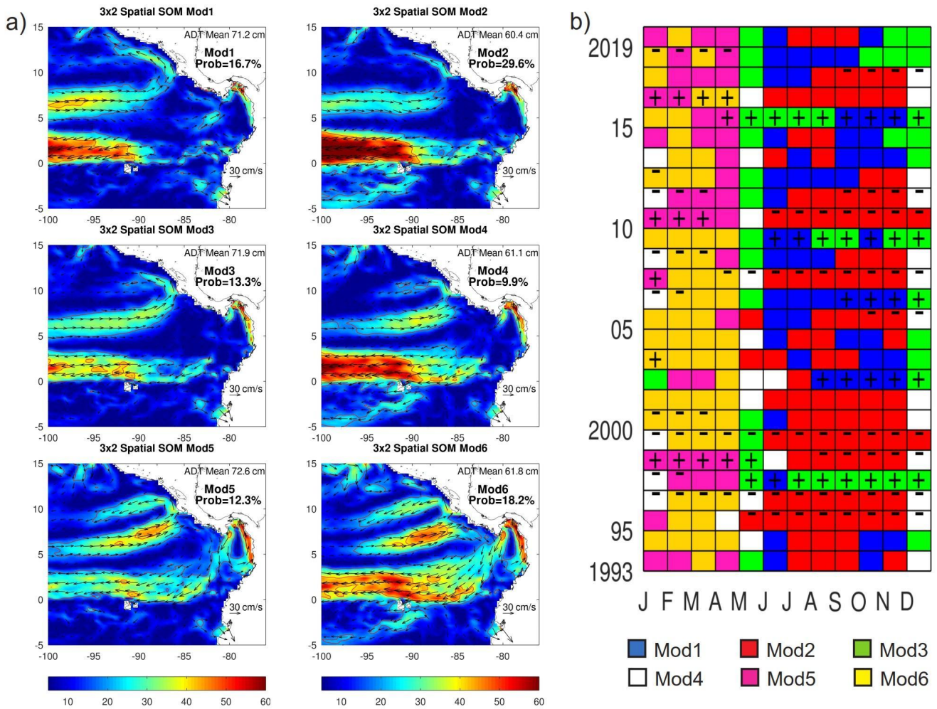
27 Figure 8. a) Spatial patterns of geostrophic speed (color scale) and currents (vectors in cm s -1 ), which results from a 3x2 SOM spatial 28 analysis in the Eastern Tropical Pacific, computed from 1993 to 2019. 20 and 40 cm s -1 contours are included. b) Monthly Best 29 Matching Unit (BMU) of SOM patterns, indicating negative (-) and positive (+) ENSO-related conditions, based on Niño 3 region.
