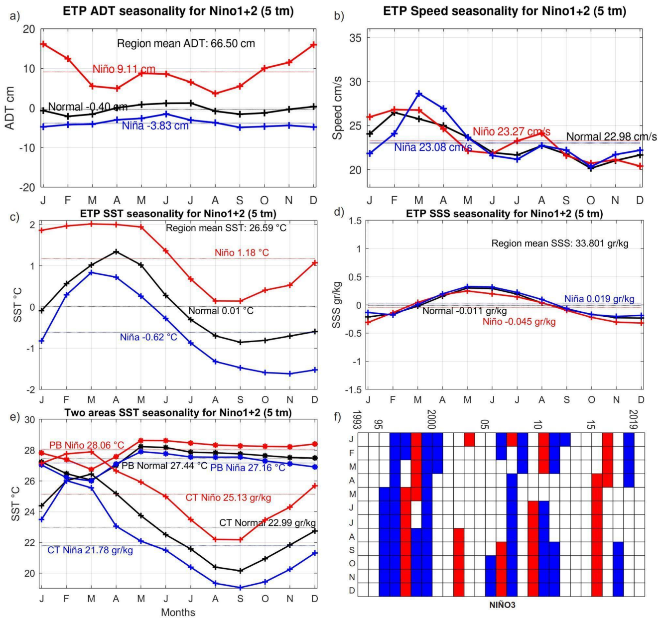
09 Figure Aux. 2. Monthly spatially averaged values in the Eastern Tropical Pacific for 1993-2019, differentiating three ENSO-related 10 conditions (based on Niño 1+2): normal (black), negative (blue) and positive (red), showing each time series annual mean. a) Absolute 11 Dynamic Topography (ADT) anomalies in cm. b) Geostrophic currents speed in cm s -1 . c) Sea Surface Temperature (SST) anomalies 12 in °C. d) Sea Surface Salinity (SSS) anomalies in gr kg -1 . Anomalies are computed subtracting the corresponding regional and 13 temporal mean (value shown in the top of each panel). e) Monthly SST of the warm Panama Bight (PB) and the Cold Tongue (CT) 14 areas shown in Figure 4. f) Matrix indicating the monthly ENSO-related condition between 1993-2019, based on Niño 3 region 15 (Section 3). Normal months in white, negative ENSO in blue and positive ENSO in red.
