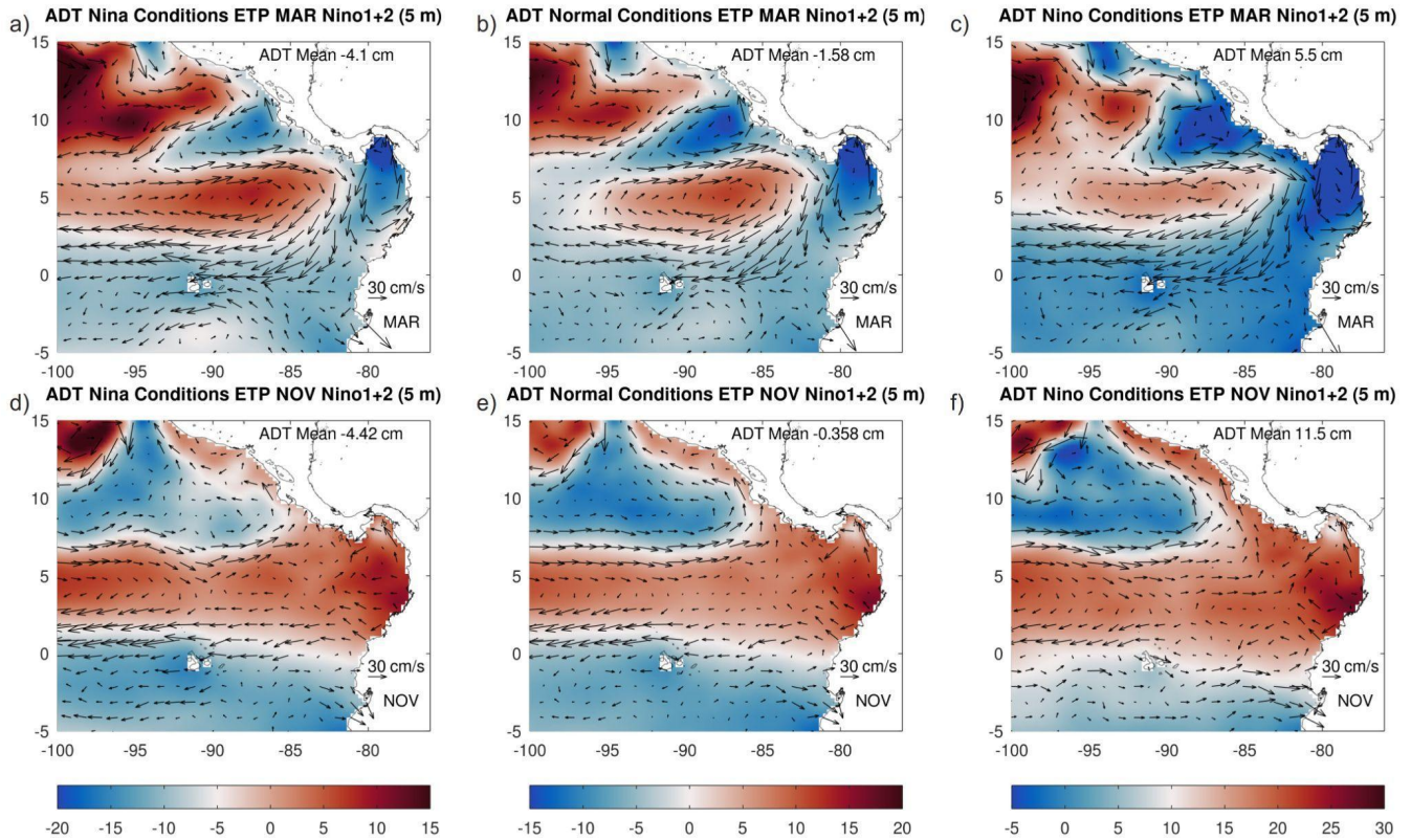
18 19 Figure 3. Monthly average of ADT anomalies (color scale in cm) and associated geostrophic circulation (vectors) for the Eastern 20 Tropical Pacific – ETP. Seasonal changes are indicated within two months: March (a,b,c) and November (d,e,f). ENSO-related 21 conditions (based on Niño 1+2) shown are: normal (b,e), negative ENSO (a,d) and positive ENSO (c,f). Each condition has a different 22 color range to highlight the ADT regional gradients, responsible for the geostrophic circulation. ADT Anomalies are computed 23 subtracting the ETP regional mean during the 1993-2019 period (66.5 cm). The regional average of the ADT anomalies for each 24 month is shown in the upper right of each panel, which coincides with time series values in Figure Aux. 3a.
