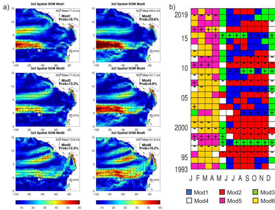
Figure 8. a) Spatial patterns of geostrophic speed (color scale) and currents (vectors in \text{cm s}^{-1} ), which results from a 3x2 SOM spatial analysis in the Eastern Tropical Pacific, computed from 1993 to 2019. 20 and 40 \text{cm s}^{-1} contours are included. b) Monthly Best Matching Unit (BMU) of SOM patterns, indicating negative (-) and positive (+) ENSO-related conditions, based on Niño 3 region.
