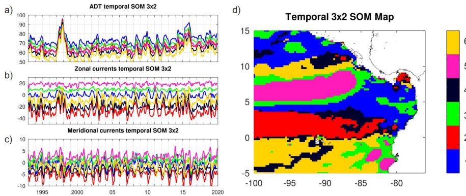
Figure 7. a) Absolute Dynamic Topography (cm), b) zonal and c) meridional geostrophic currents (cm s -1 ) time series from 1993 to 2019 which results from a 3x2 SOM temporal analysis in the Eastern Tropical Pacific. d) Sub-regions represented by the six temporal SOM patterns.
