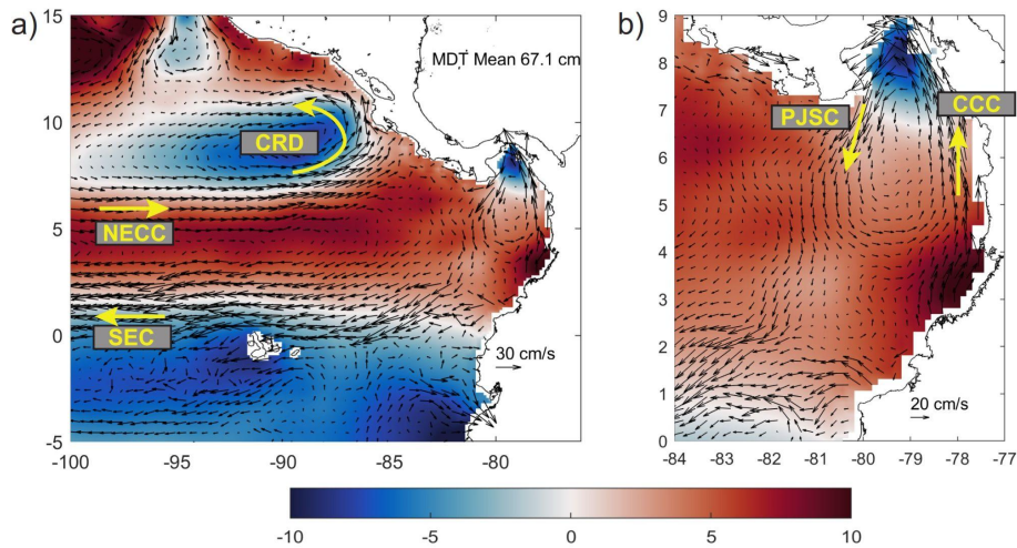
Figure 2. Mean Dynamic Topography (MDT) anomalies (color scale) and associated geostrophic circulation (vectors) representative of the 1993-2012 period for the a) Eastern Tropical Pacific – ETP east of 100° W and b) the Panama Basin. MDT anomalies are computed subtracting the ETP regional mean (67.1 cm). South Equatorial Current (SEC), North Equatorial Counter Current (NECC), Costa Rica Dome (CRD), Colombia Coastal Current (CCC) and the Panama Jet Surface Current (PJSC) are shown.
